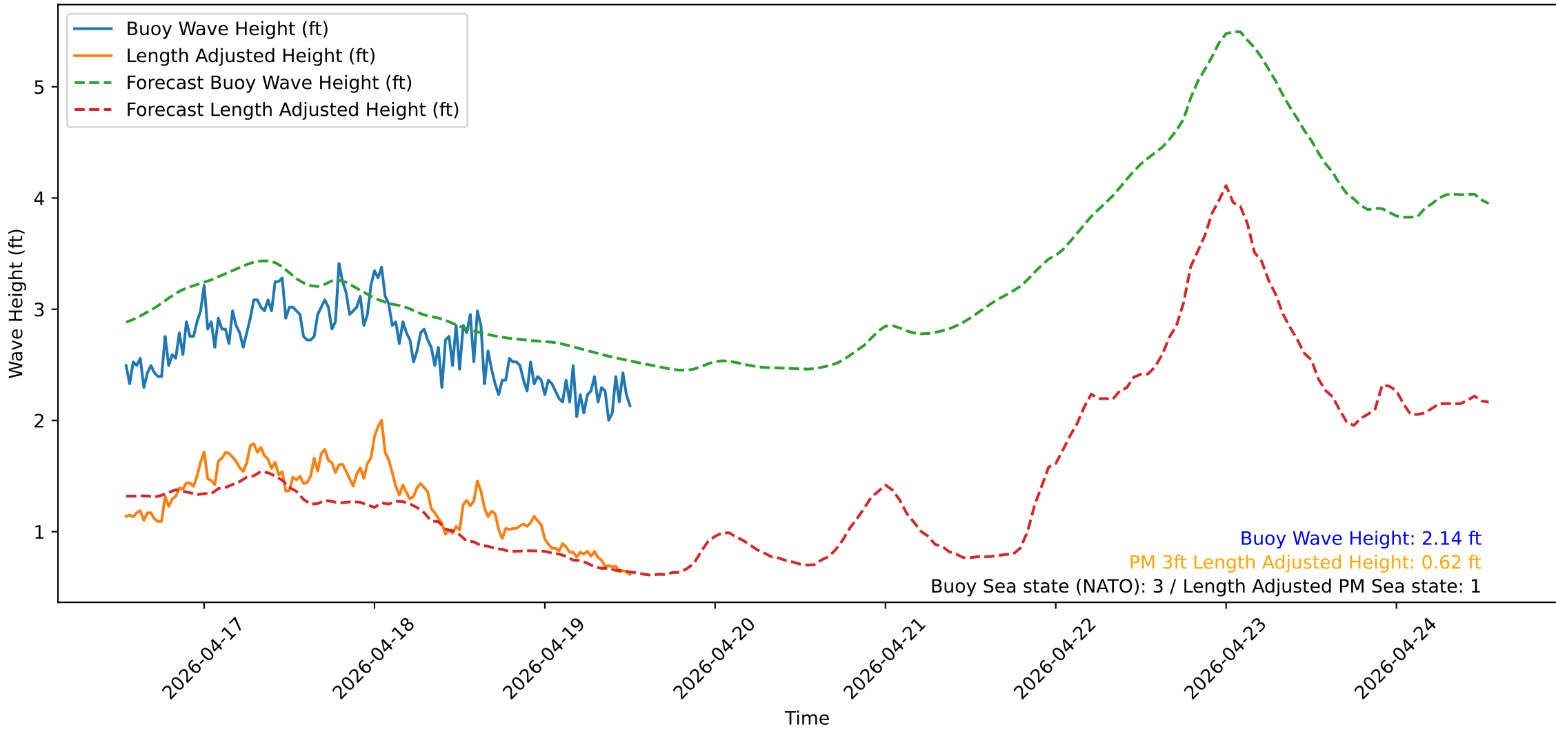
Wave Heights over Time for Oceanside Harbor at 2026-04-19 13:00:31
