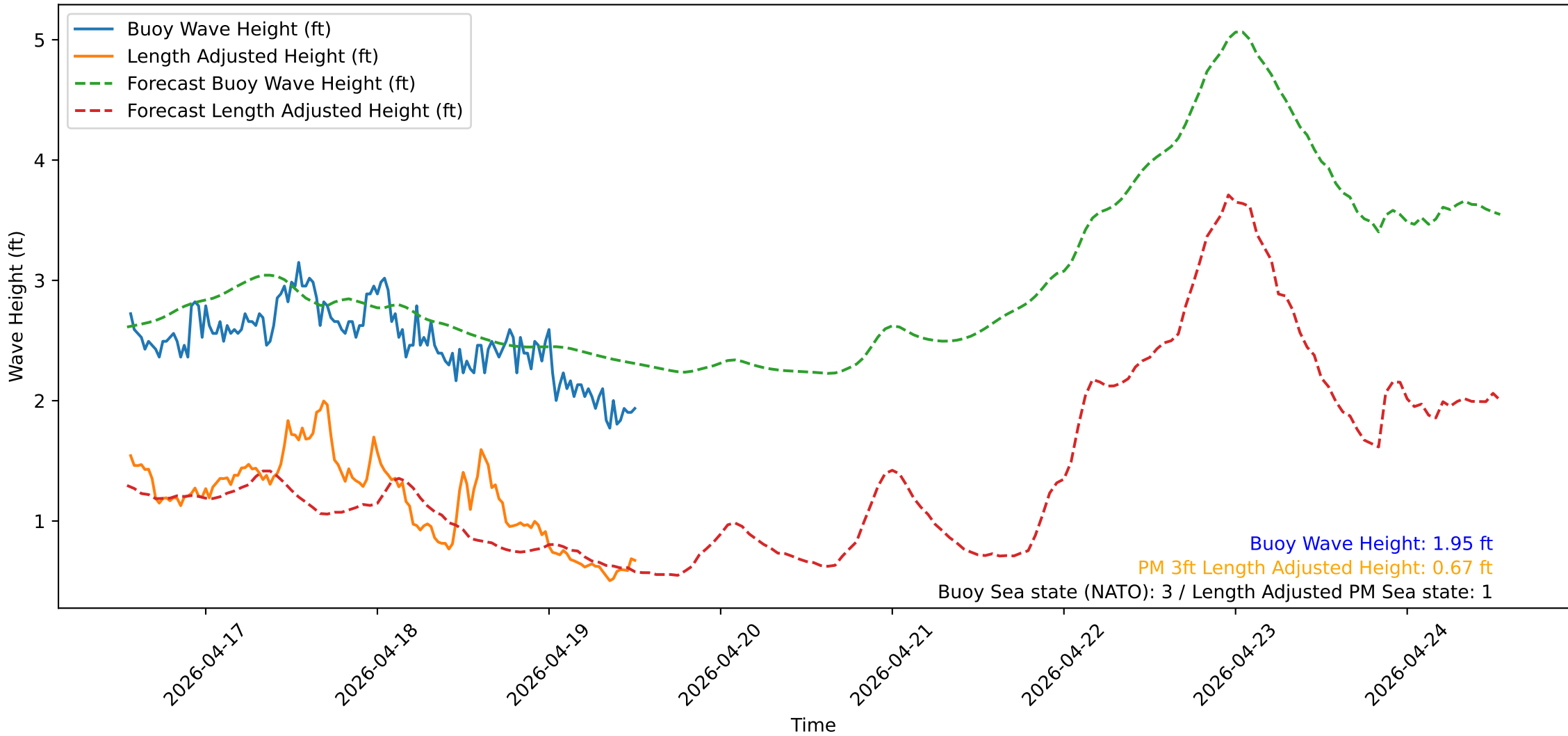
Wave Heights over Time for Red Beach at 2026-04-19 13:00:50
