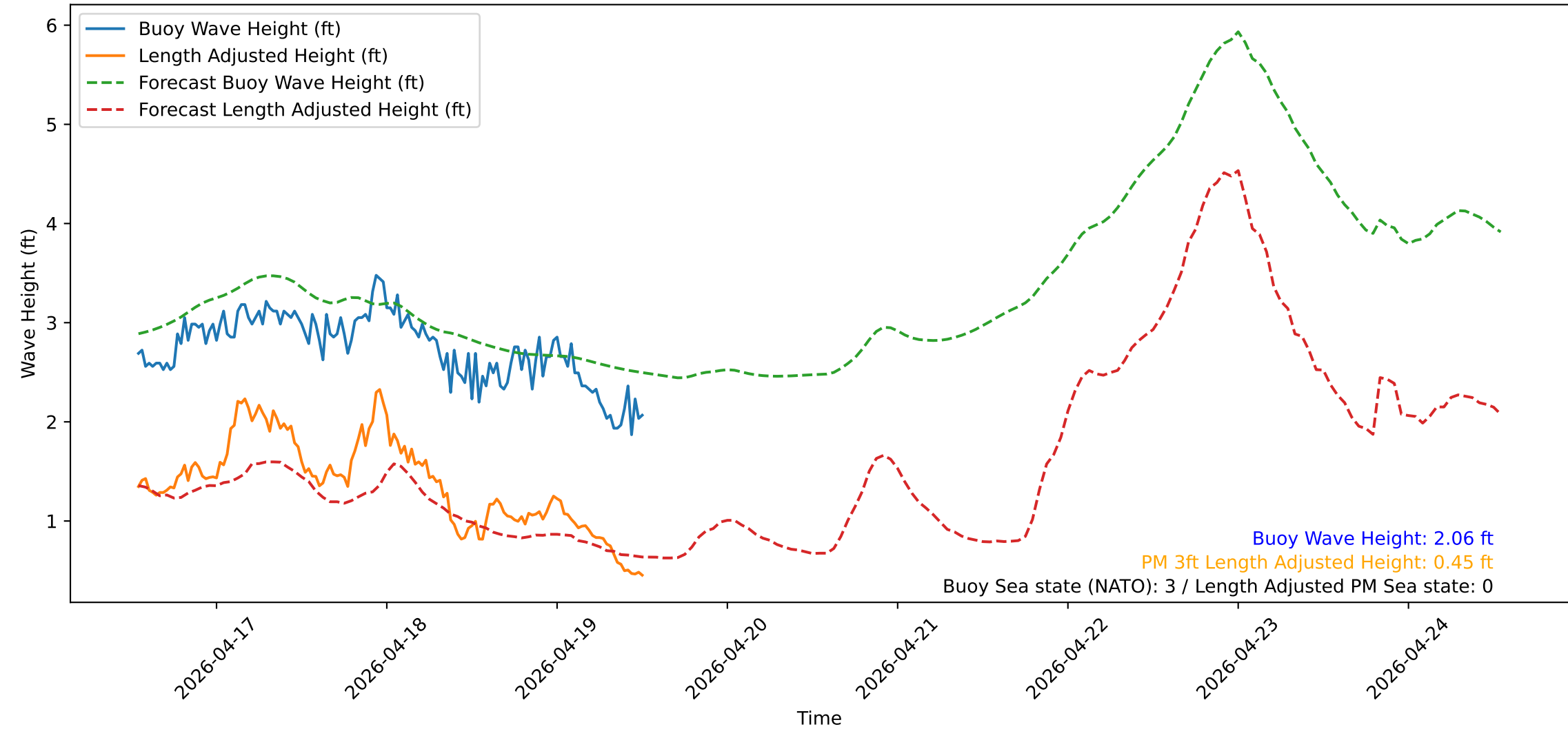
Wave Heights over Time for Green Beach at 2026-04-19 13:01:12
