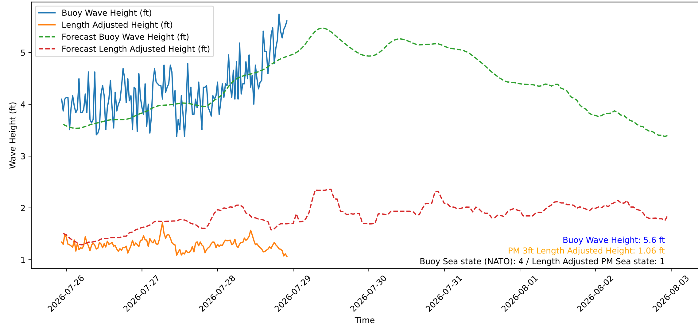
Wave Heights over Time for Green Beach at 2026-07-28 22:41:07
