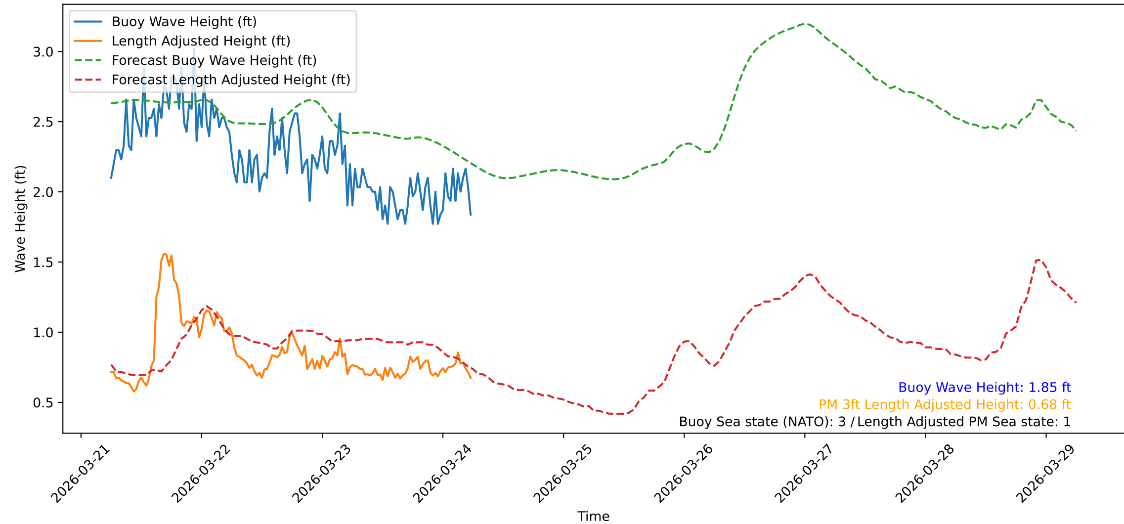
Wave Heights over Time for Oceanside Harbor at 2026-03-24 06:10:31
