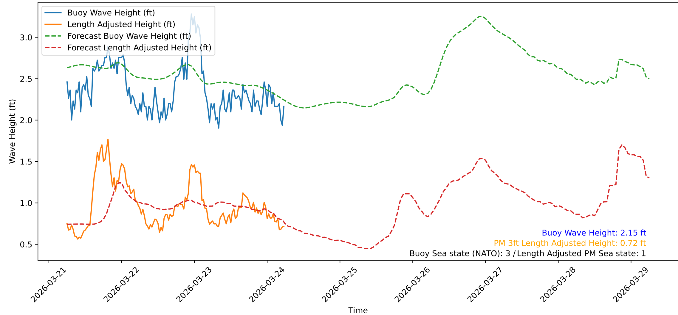
Wave Heights over Time for Green Beach at 2026-03-24 06:11:09
