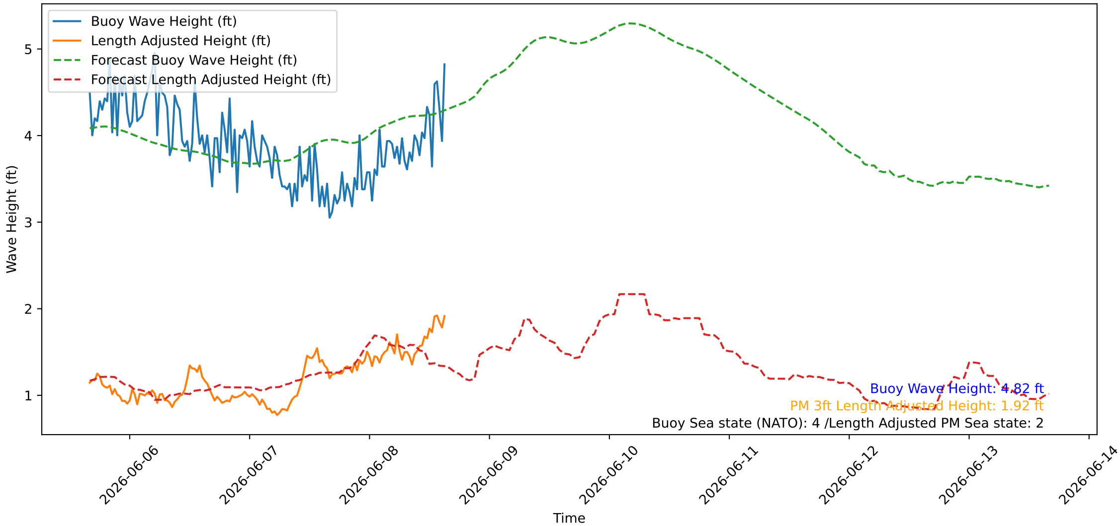
Wave Heights over Time for Red Beach at 2026-06-08 15:40:46
