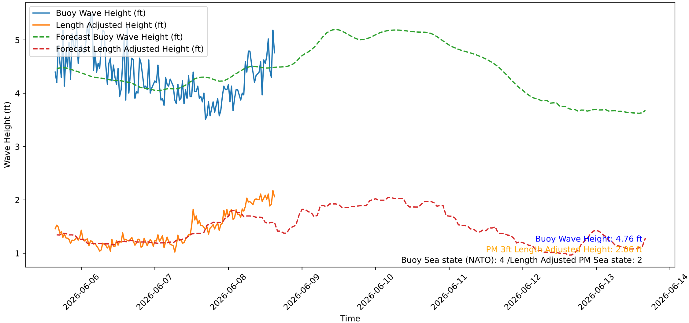
Wave Heights over Time for Oceanside Harbor at 2026-06-08 15:40:26
