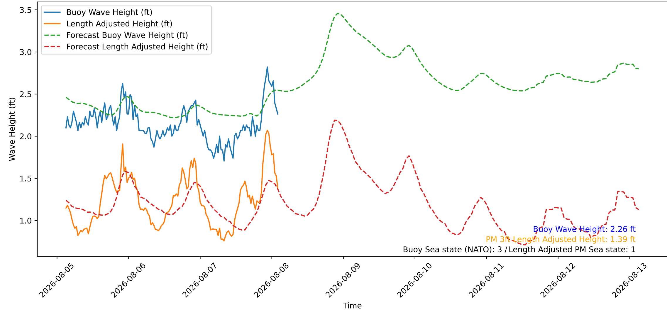
Wave Heights over Time for Green Beach at 2026-08-08 02:51:10
