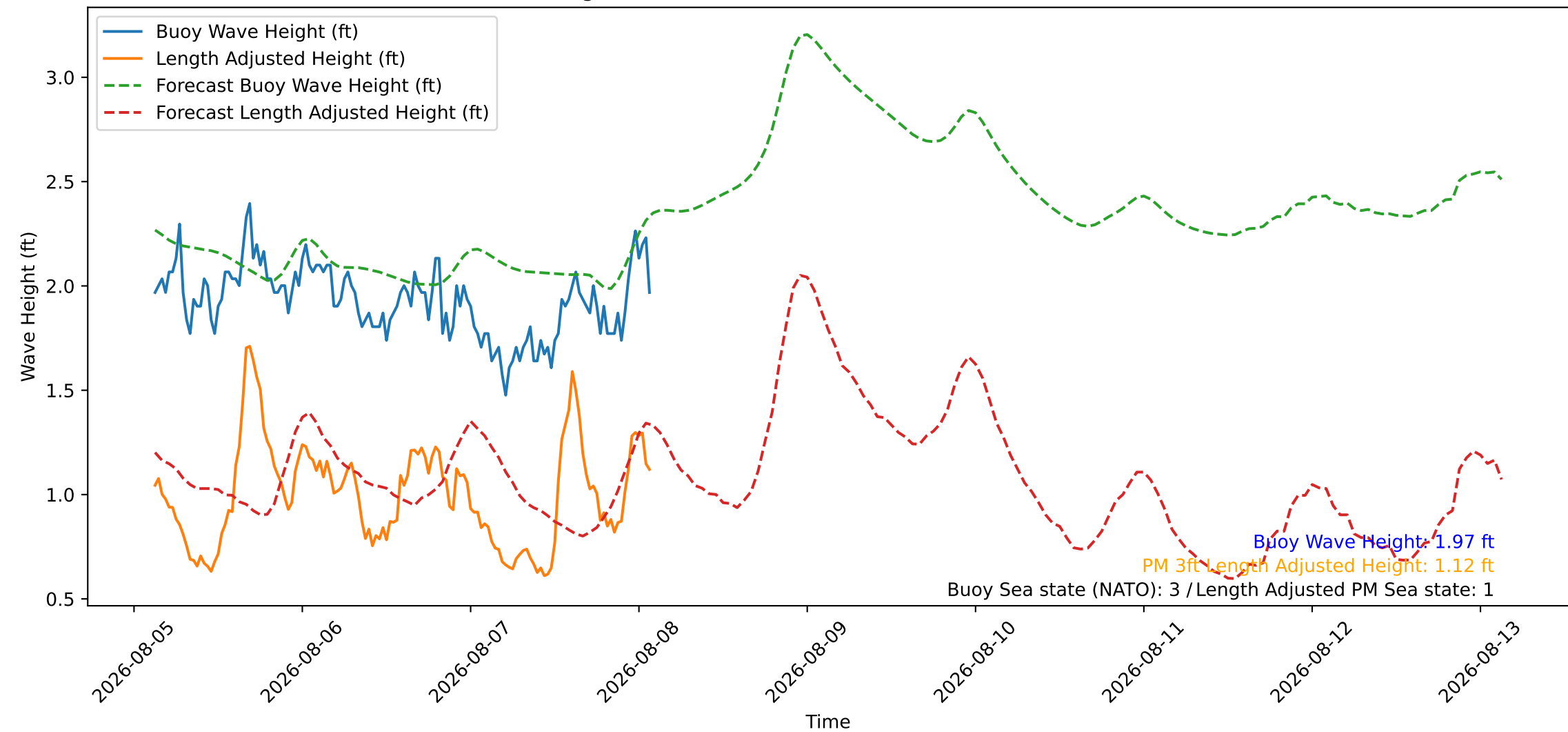
Wave Heights over Time for Red Beach at 2026-08-08 02:50:48
