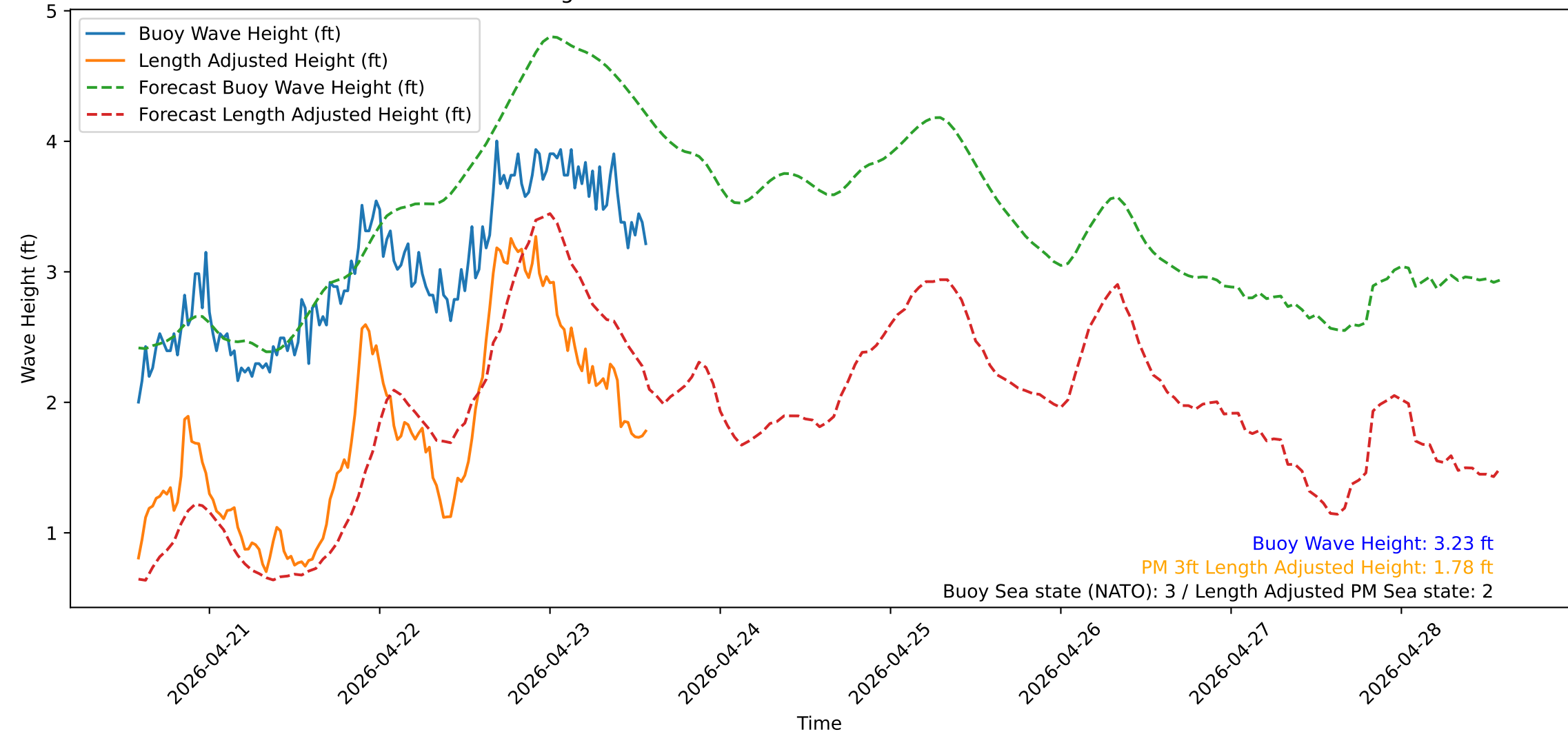
Wave Heights over Time for Green Beach at 2026-04-23 14:11:12
