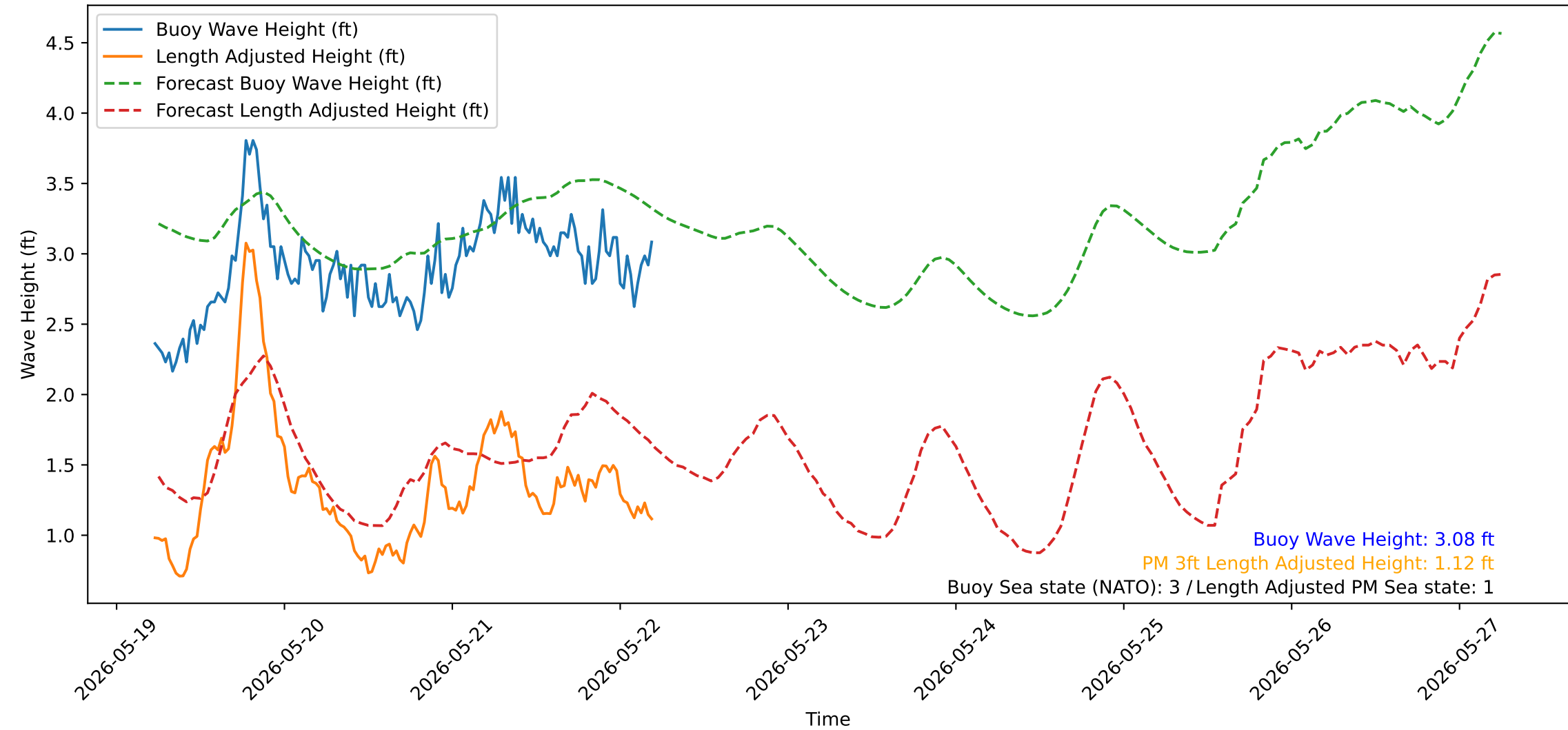
Wave Heights over Time for Green Beach at 2026-05-22 05:31:13
