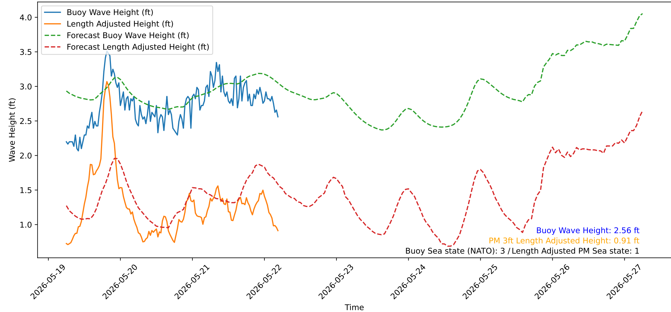
Wave Heights over Time for Red Beach at 2026-05-22 05:30:51
