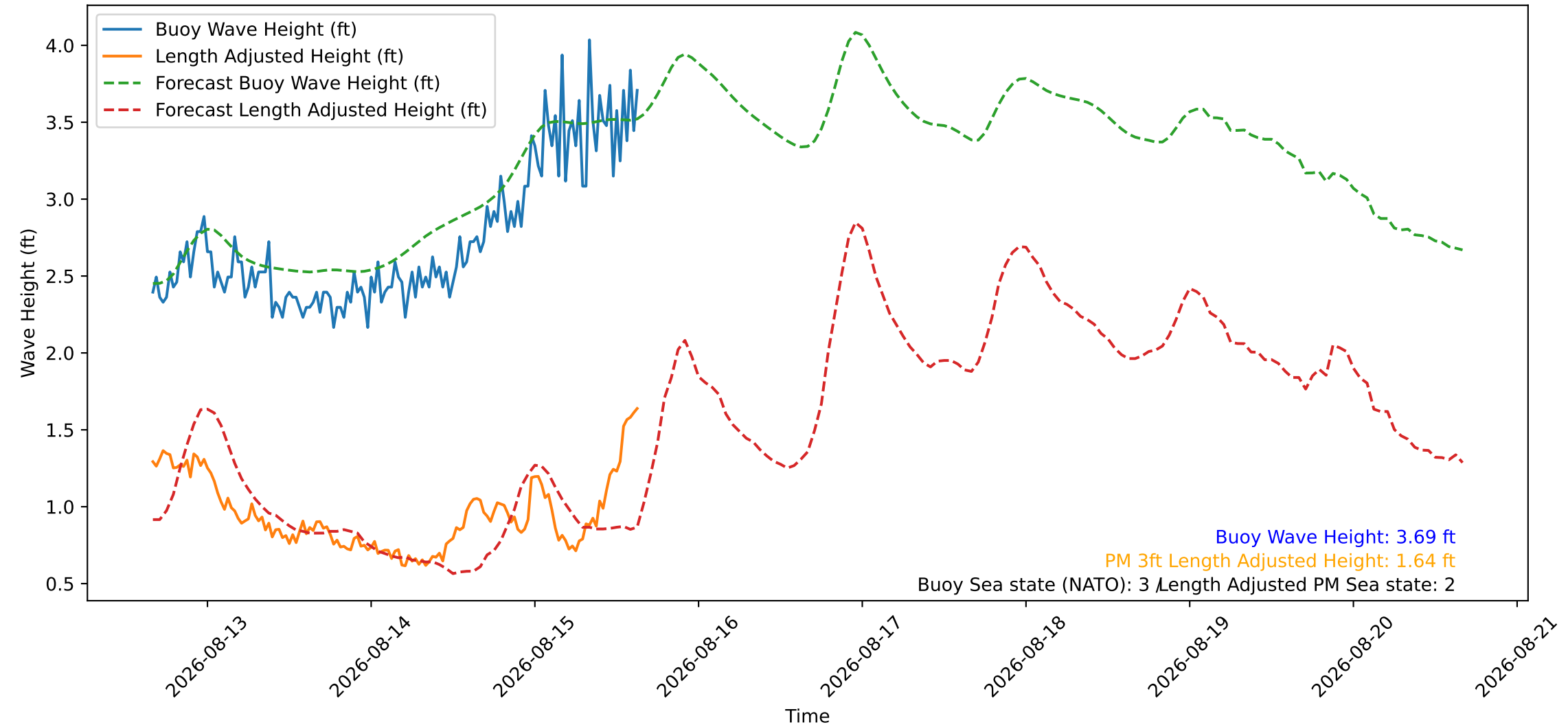
Wave Heights over Time for Red Beach at 2026-08-15 15:50:48
