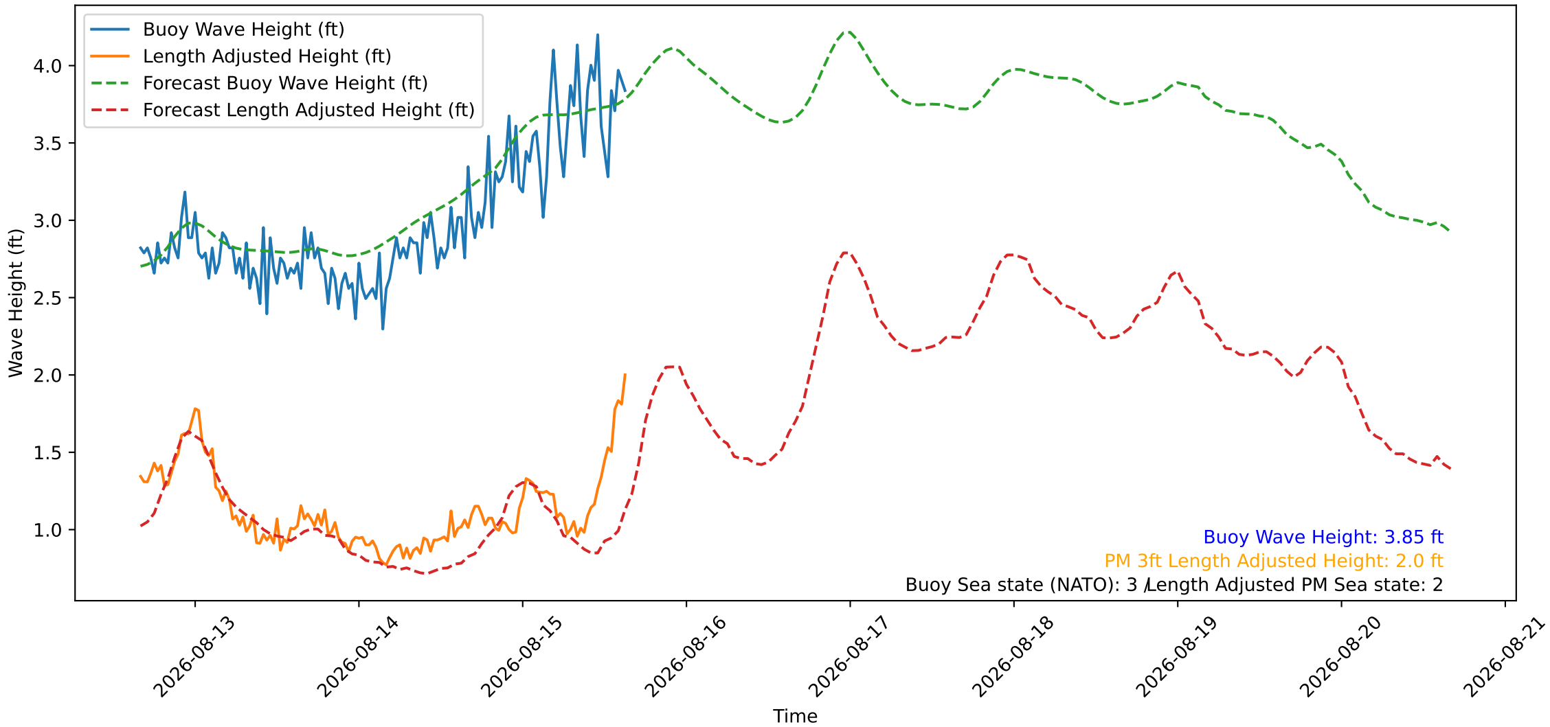
Wave Heights over Time for Oceanside Harbor at 2026-08-15 15:50:27
