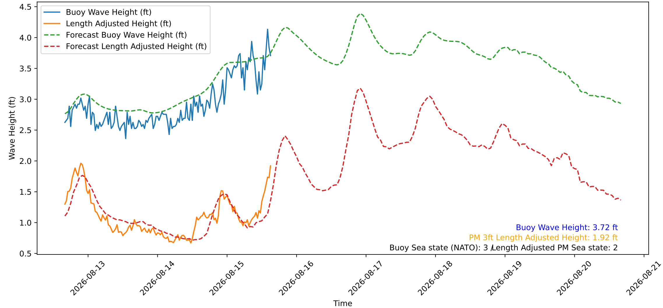
Wave Heights over Time for Green Beach at 2026-08-15 15:51:10
