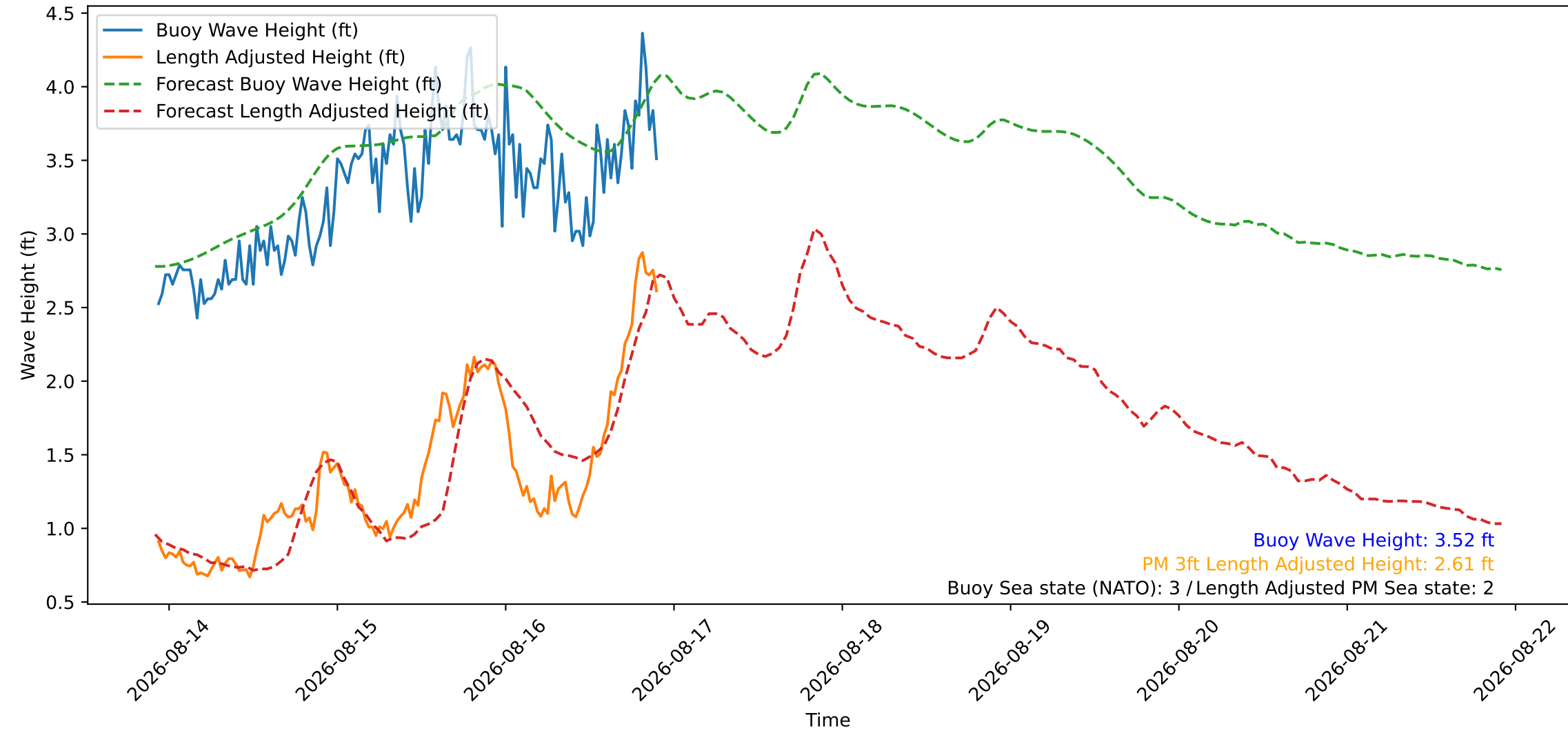
Wave Heights over Time for Green Beach at 2026-08-16 22:11:08
