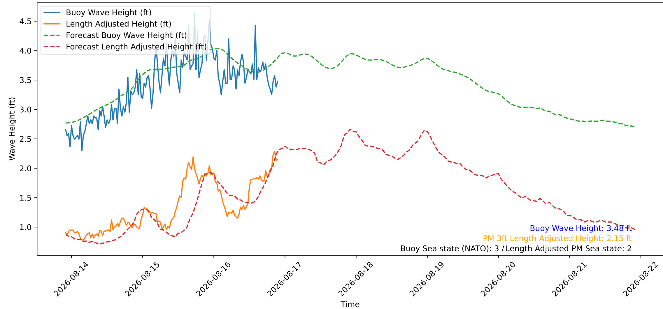
Wave Heights over Time for Oceanside Harbor at 2026-08-16 22:10:26
