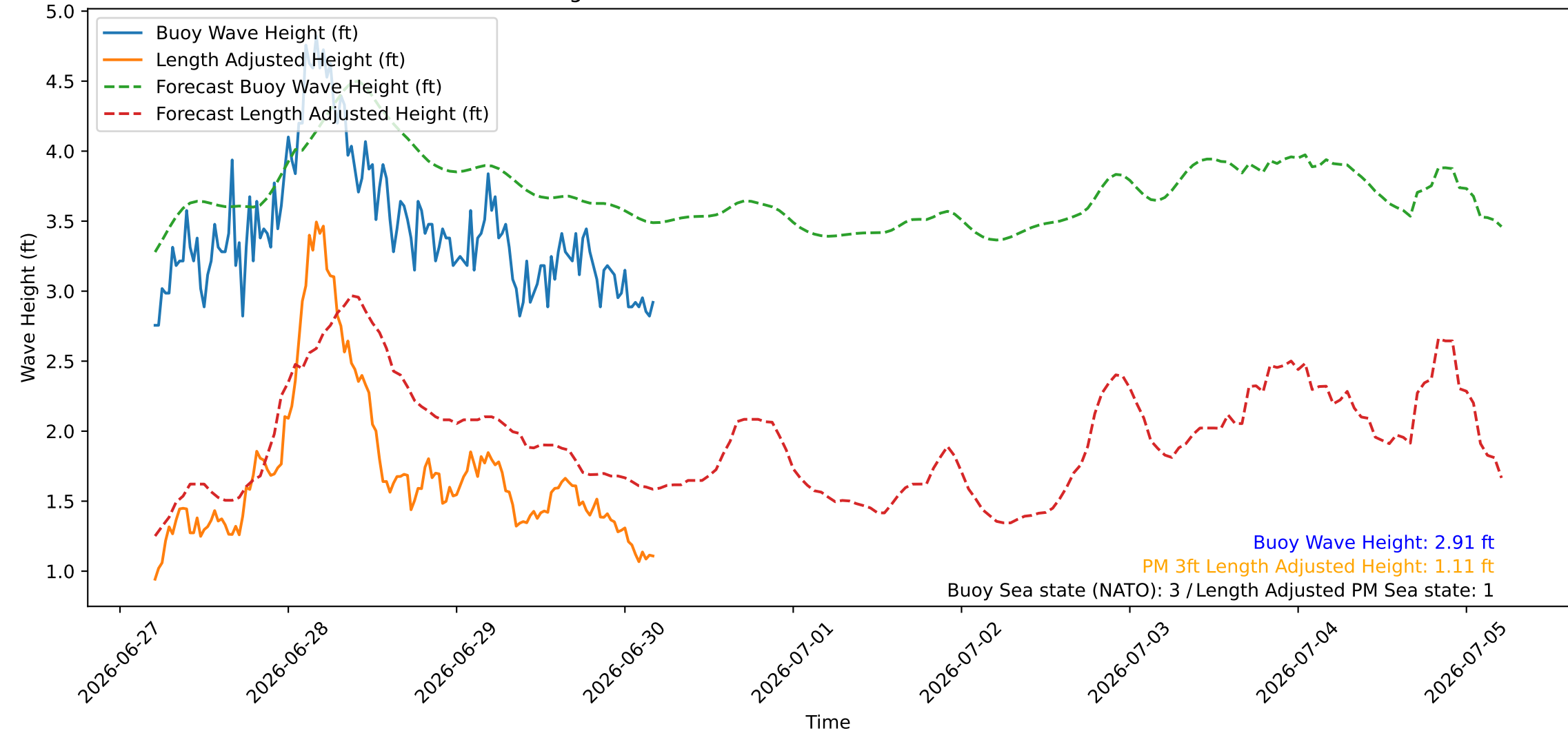
Wave Heights over Time for Green Beach at 2026-06-30 04:51:09
