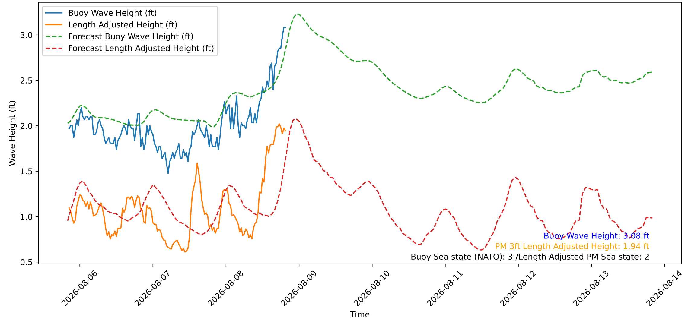
Wave Heights over Time for Red Beach at 2026-08-08 20:10:46
