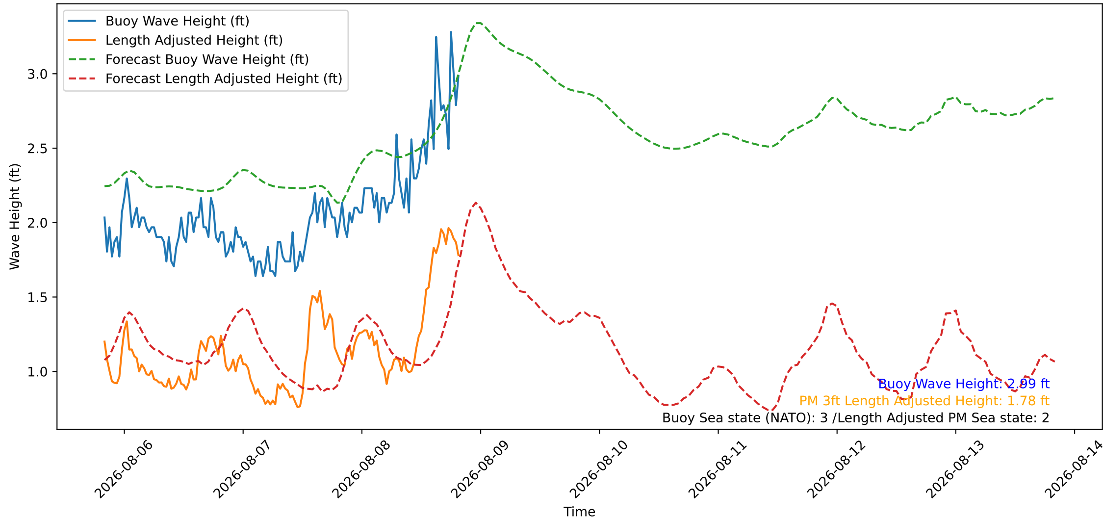
Wave Heights over Time for Oceanside Harbor at 2026-08-08 20:10:26
