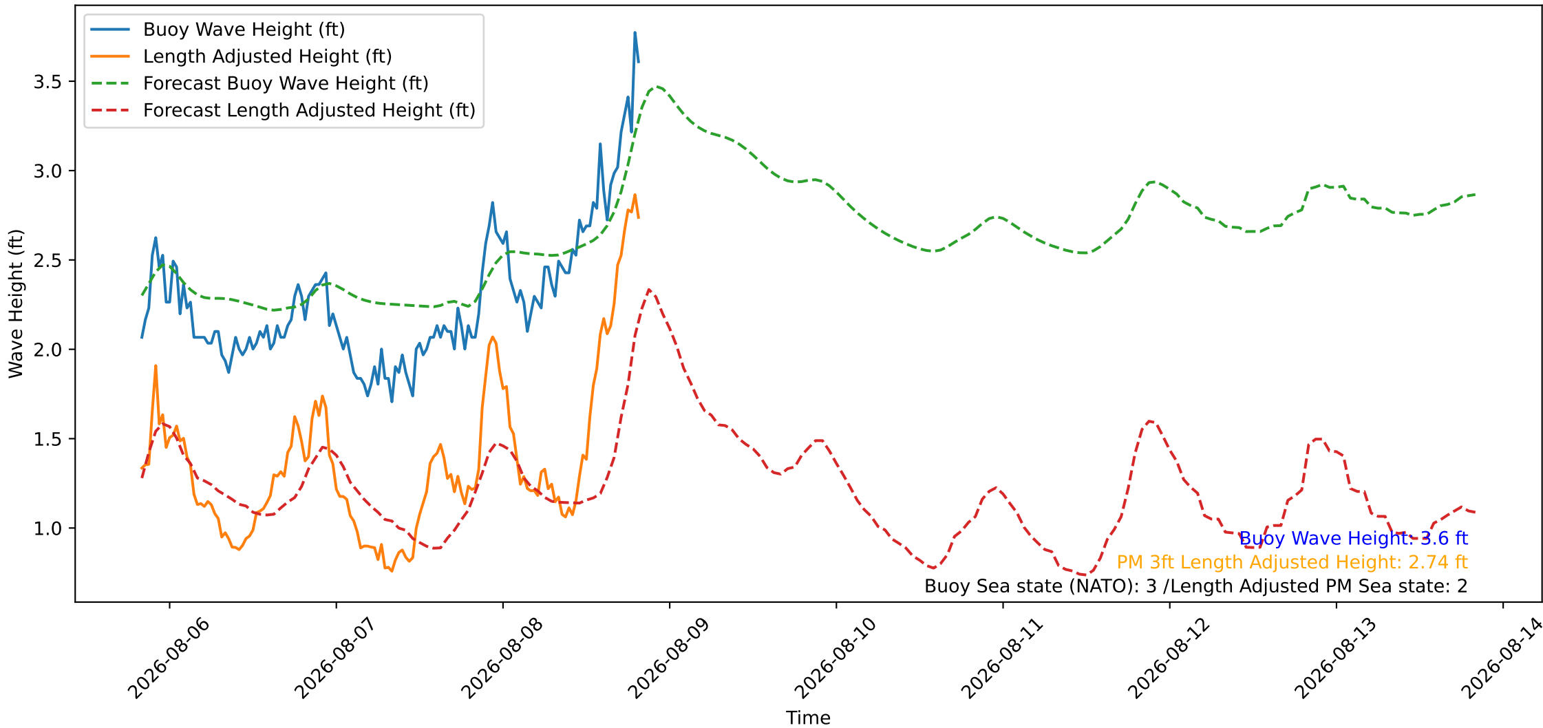
Wave Heights over Time for Green Beach at 2026-08-08 20:11:08
