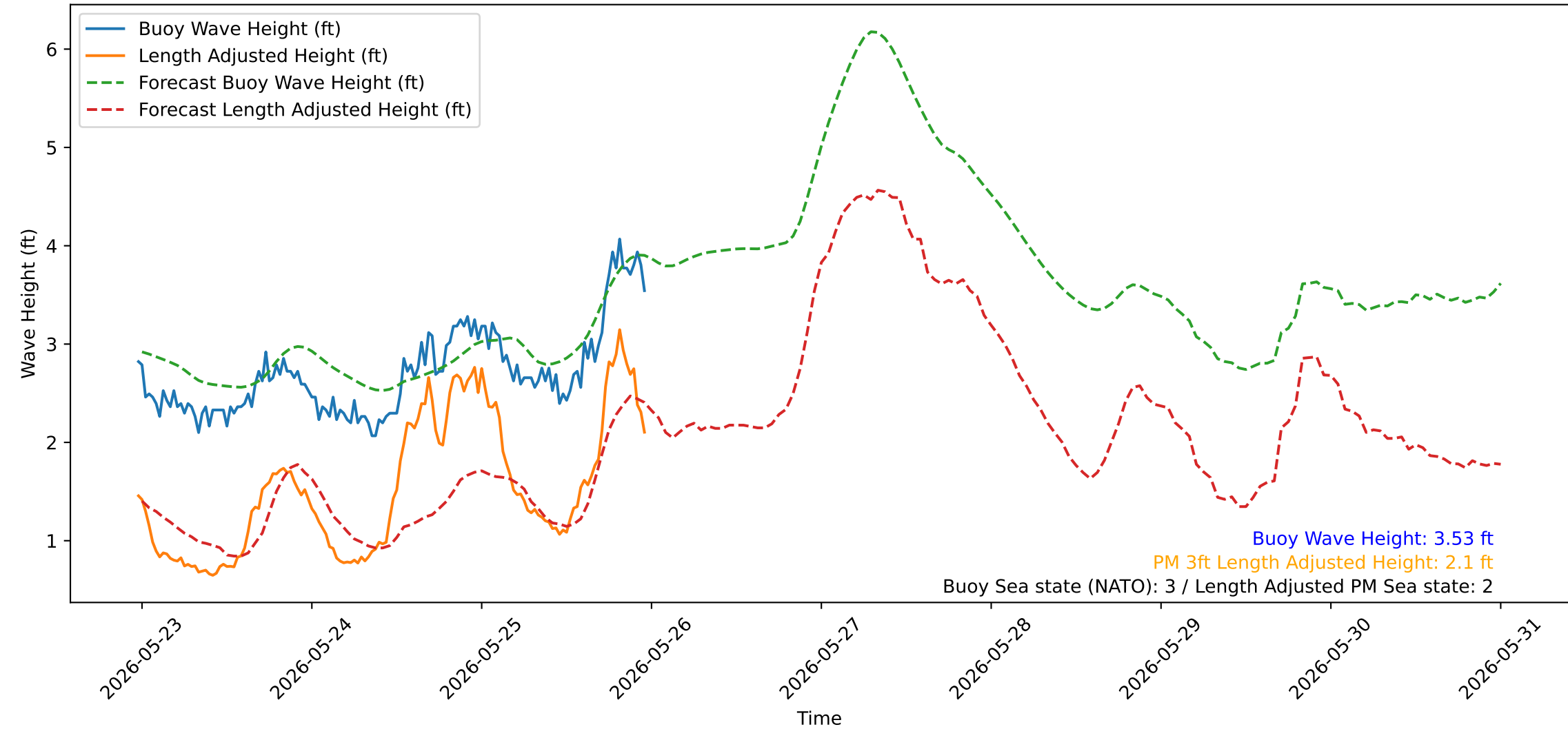
Wave Heights over Time for Green Beach at 2026-05-25 23:41:12
