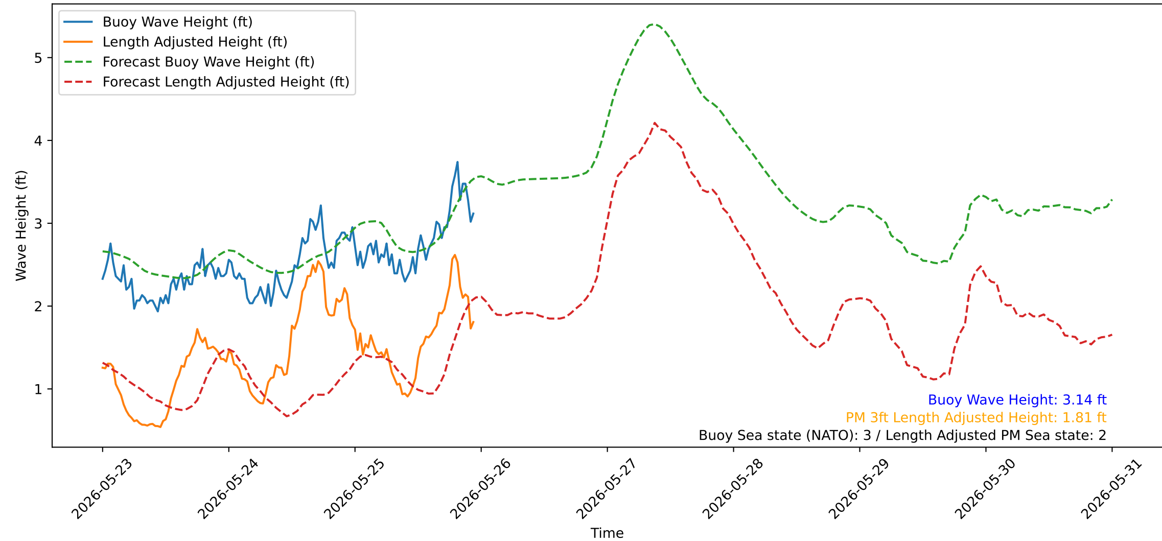
Wave Heights over Time for Red Beach at 2026-05-25 23:40:49
