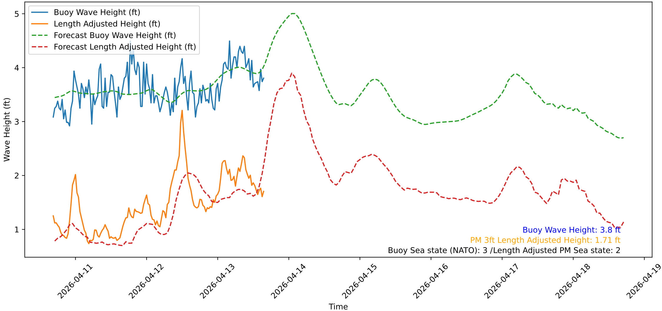
Wave Heights over Time for Green Beach at 2026-04-13 16:31:12
