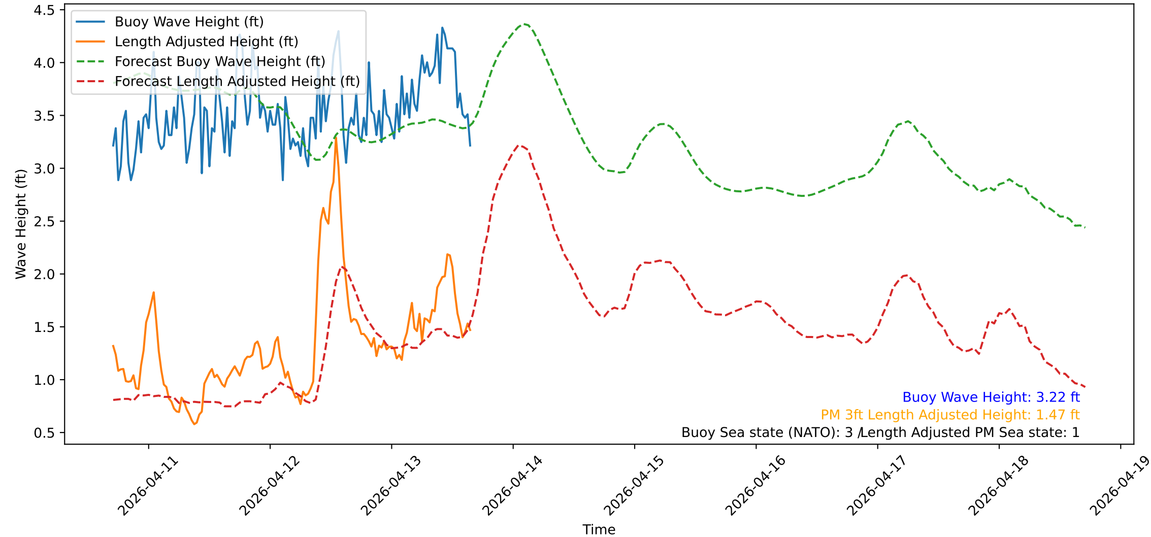
Wave Heights over Time for Red Beach at 2026-04-13 16:30:50
