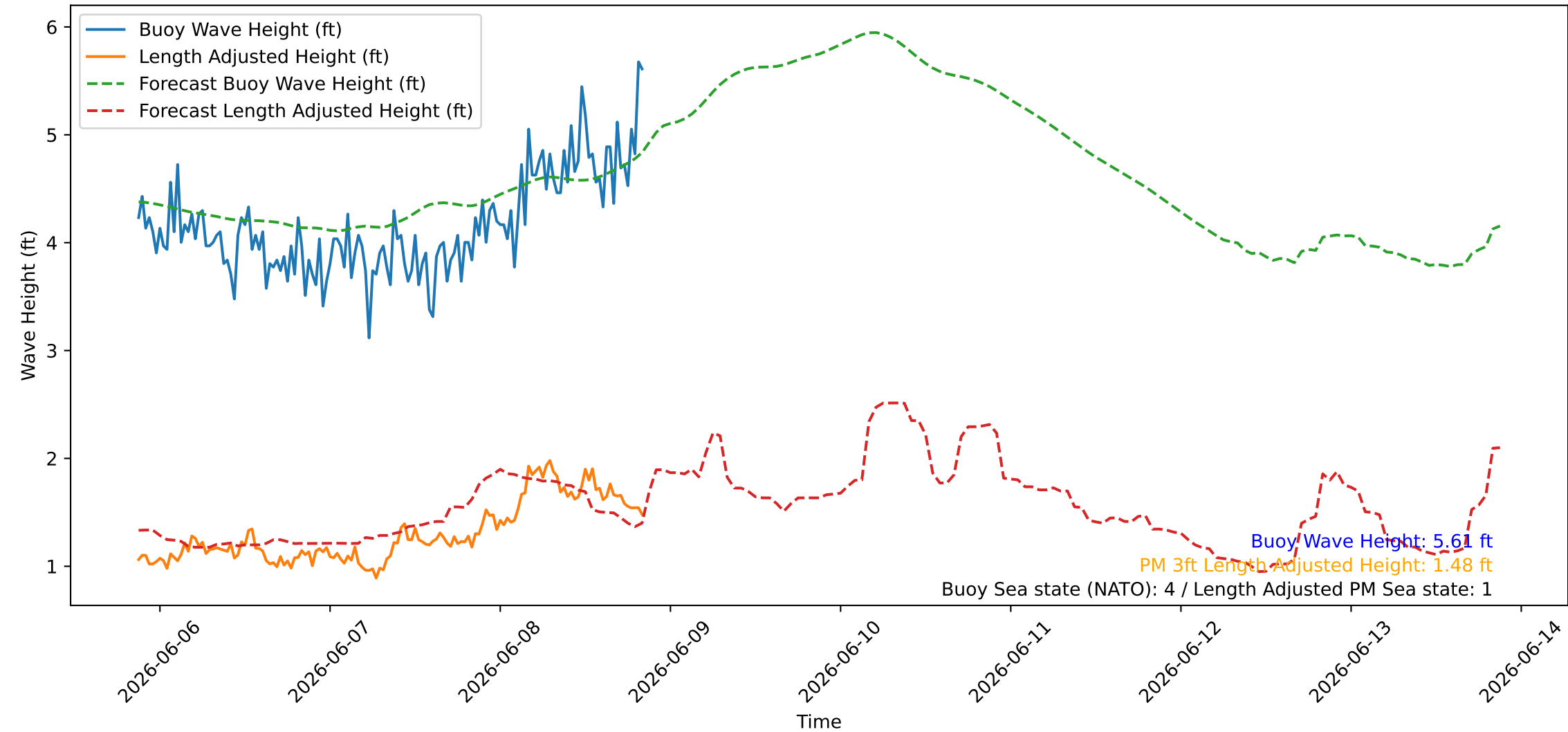
Wave Heights over Time for Green Beach at 2026-06-08 21:01:09
