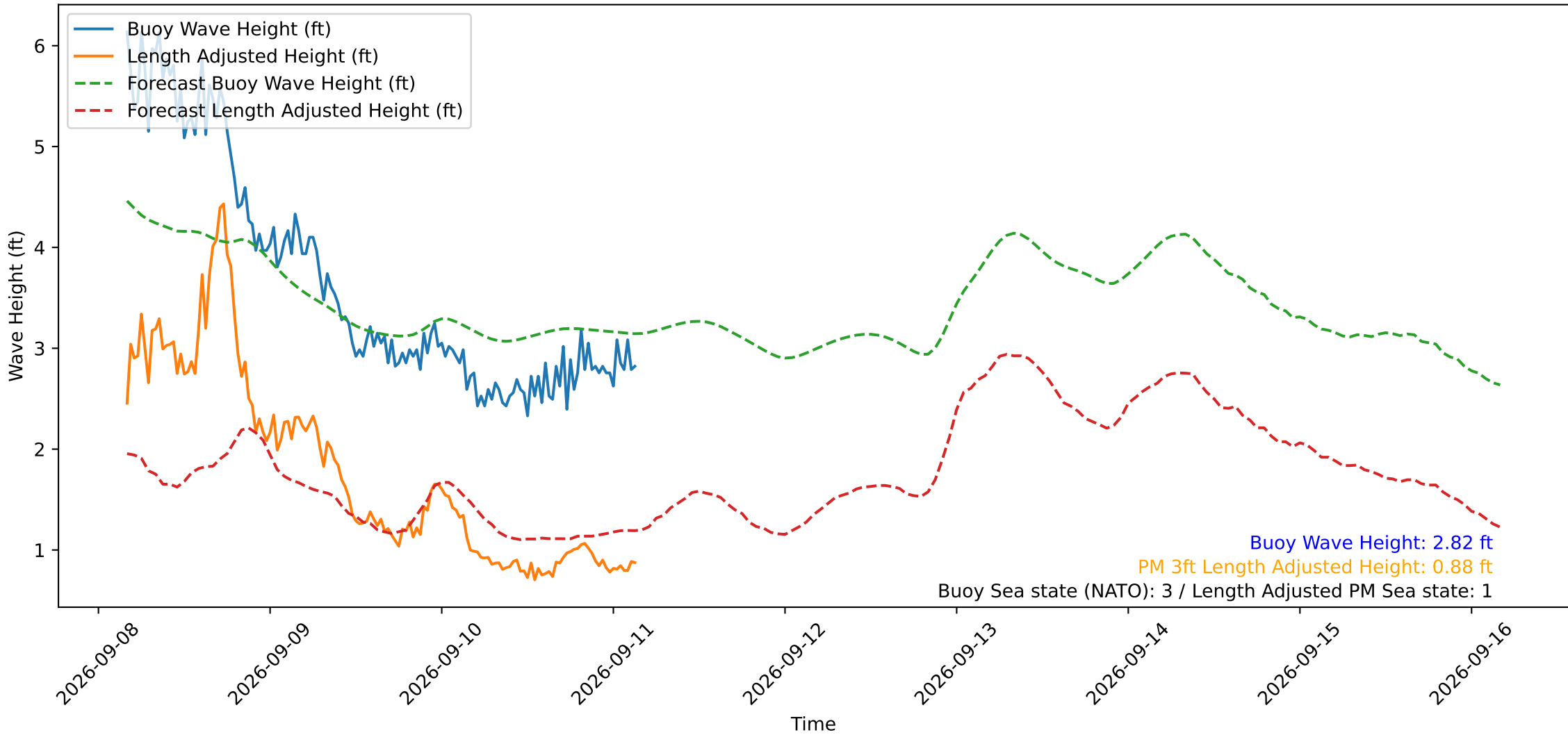
Wave Heights over Time for Red Beach at 2026-09-11 03:50:50
