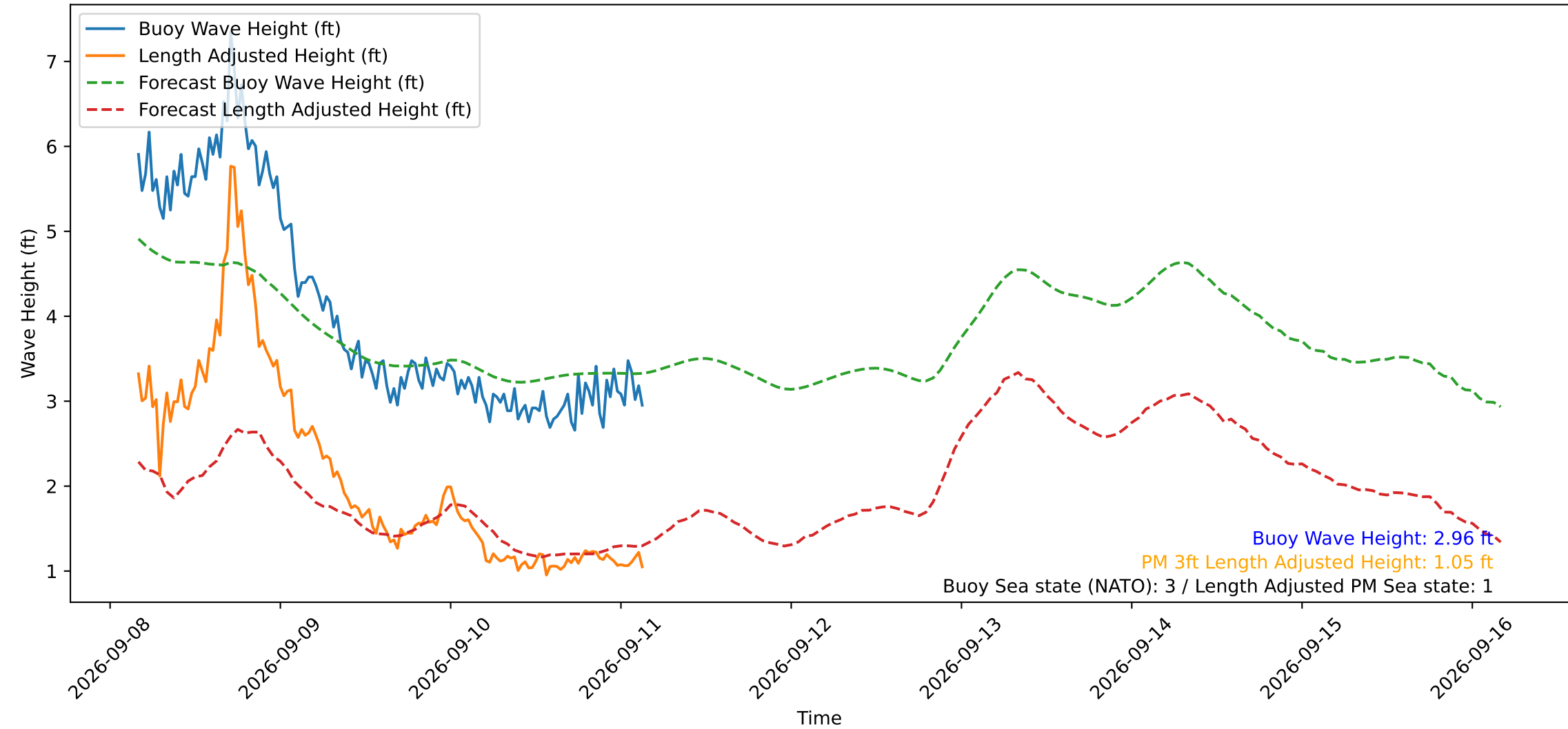
Wave Heights over Time for Oceanside Harbor at 2026-09-11 03:50:29
