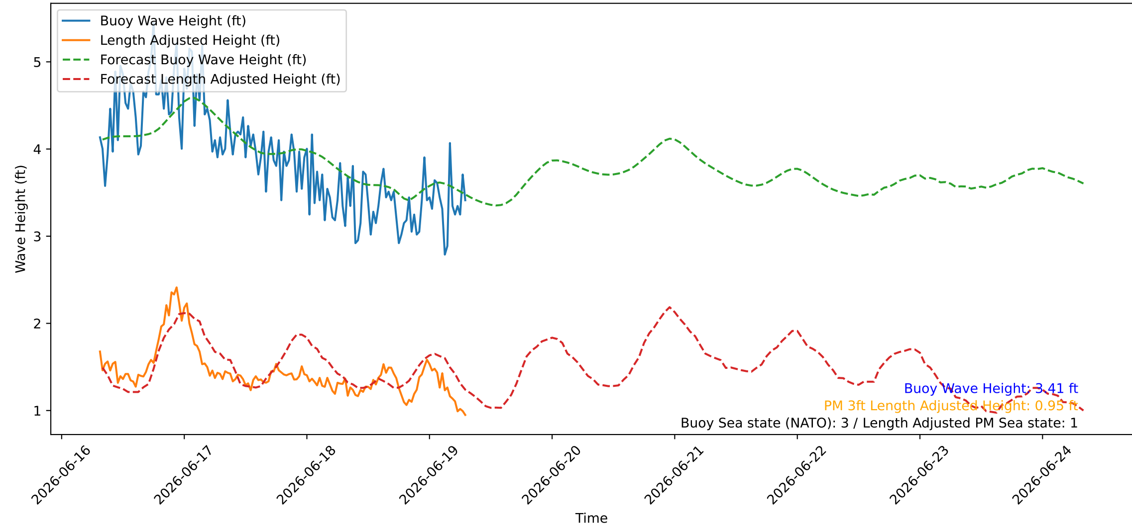
Wave Heights over Time for Oceanside Harbor at 2026-06-19 07:40:27
