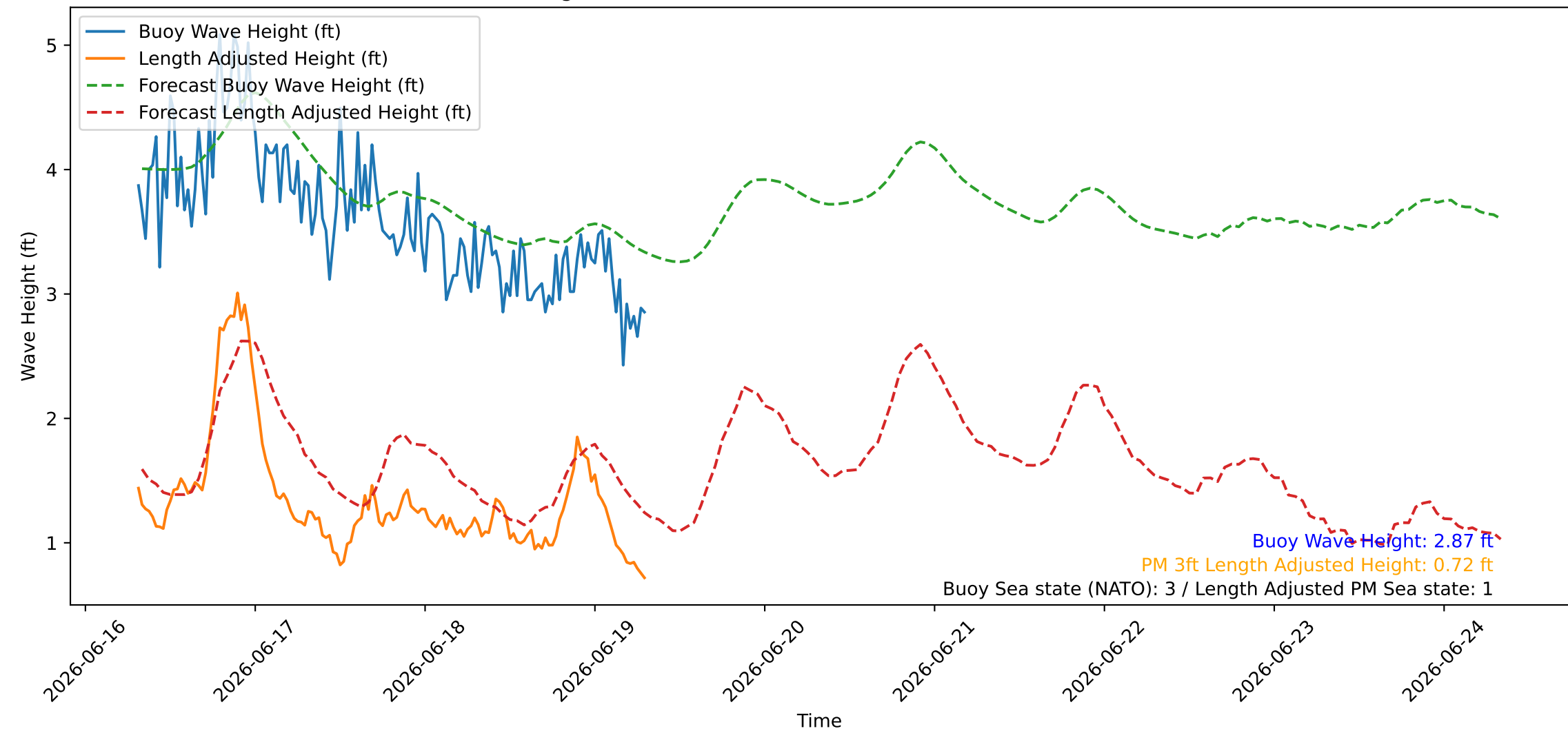
Wave Heights over Time for Green Beach at 2026-06-19 07:41:09
