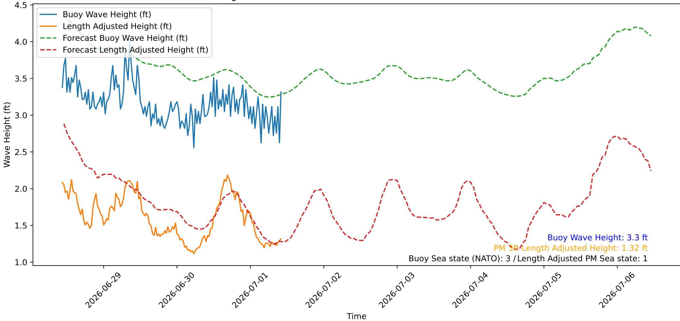
Wave Heights over Time for Oceanside Harbor at 2026-07-01 10:30:27
