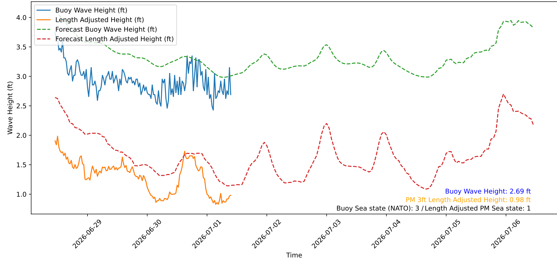
Wave Heights over Time for Red Beach at 2026-07-01 10:30:46
