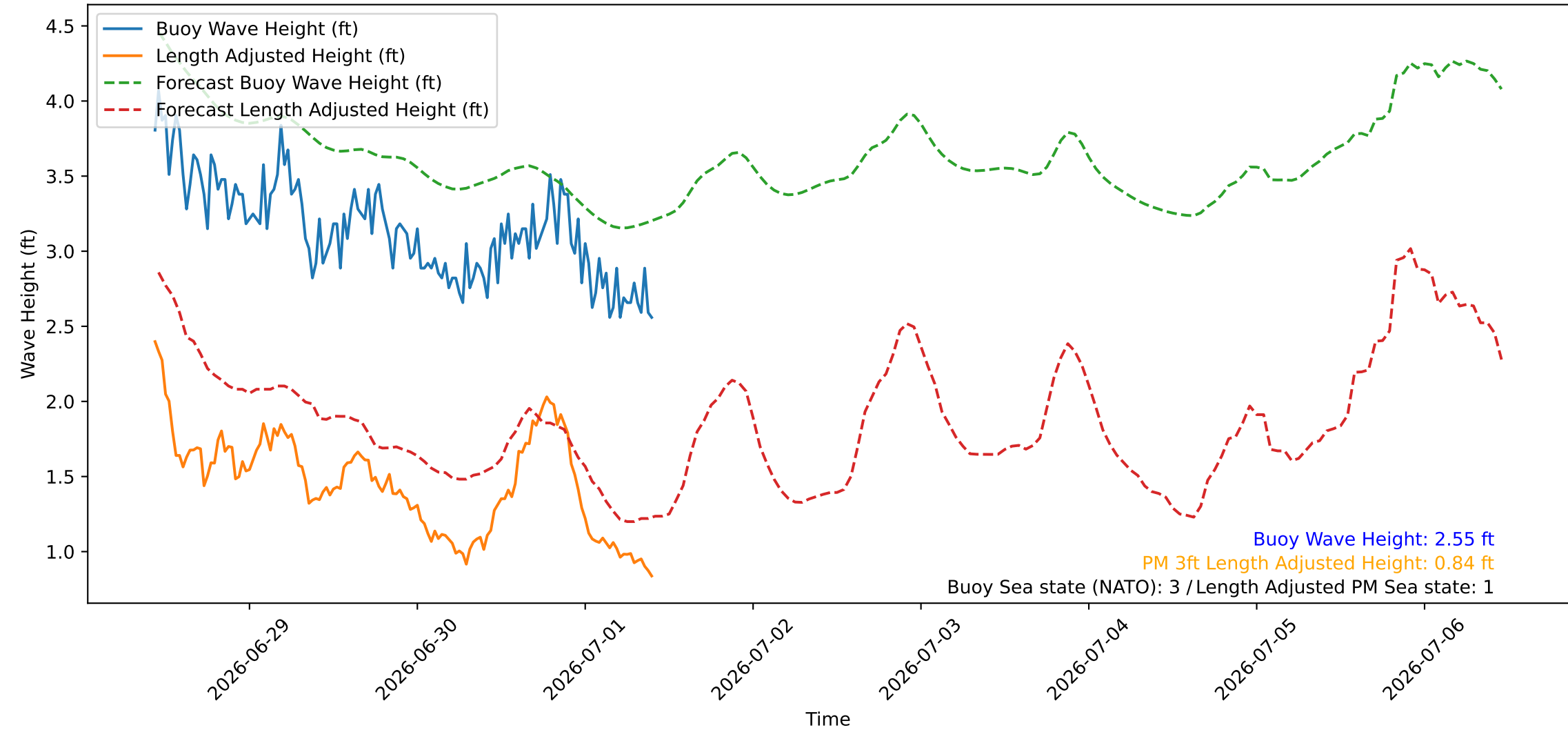
Wave Heights over Time for Green Beach at 2026-07-01 10:31:08
