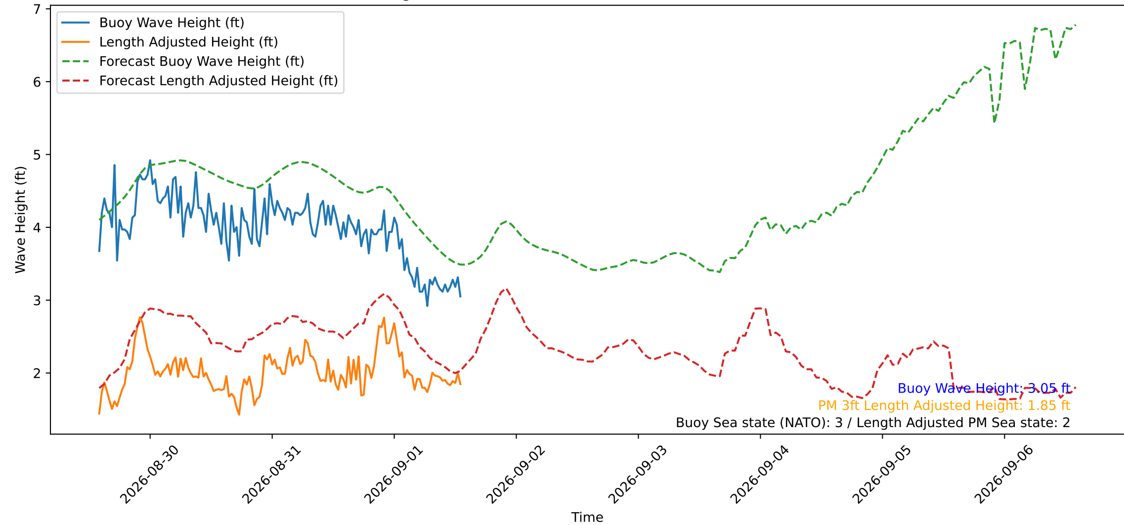
Wave Heights over Time for Green Beach at 2026-09-01 13:51:15
