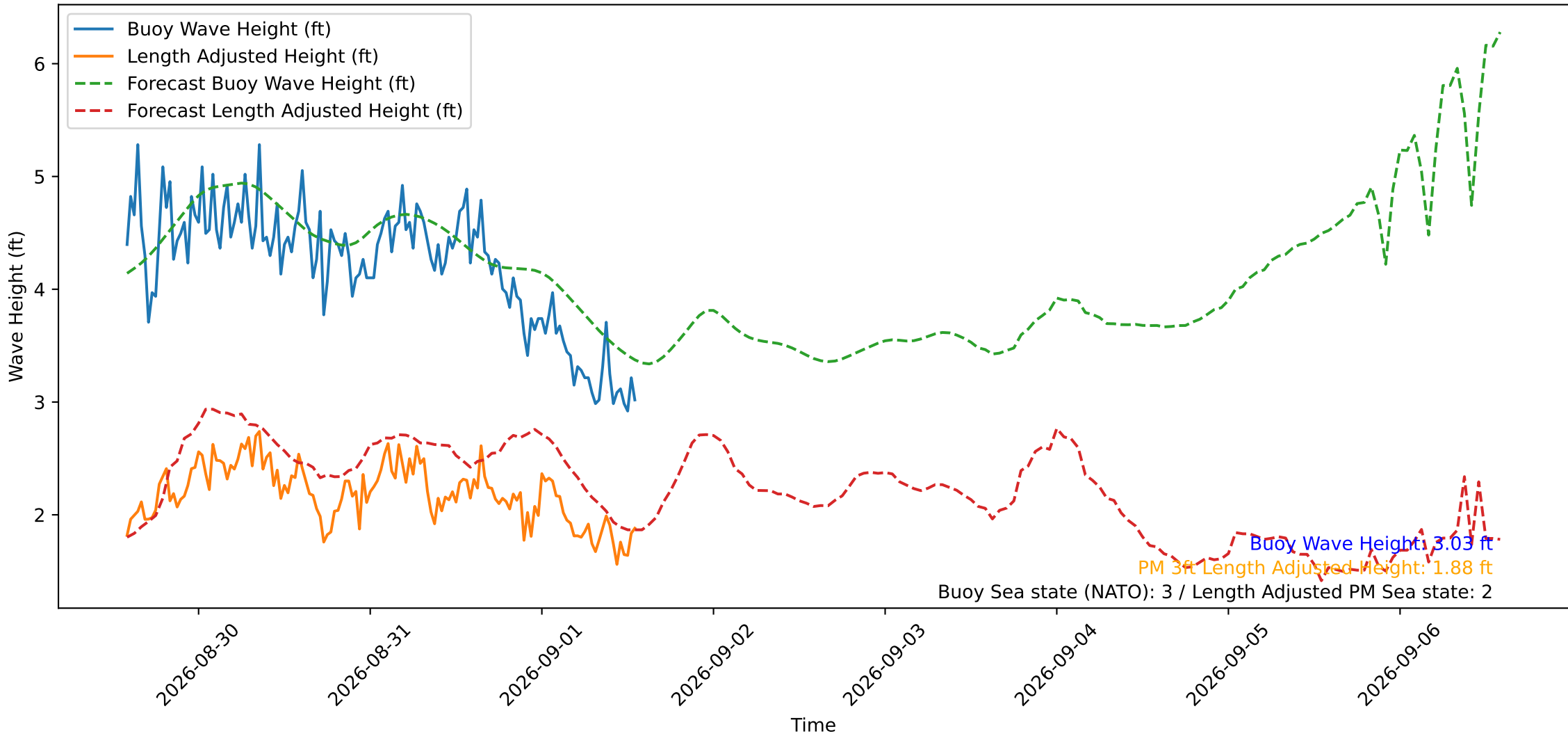
Wave Heights over Time for Oceanside Harbor at 2026-09-01 13:50:30
