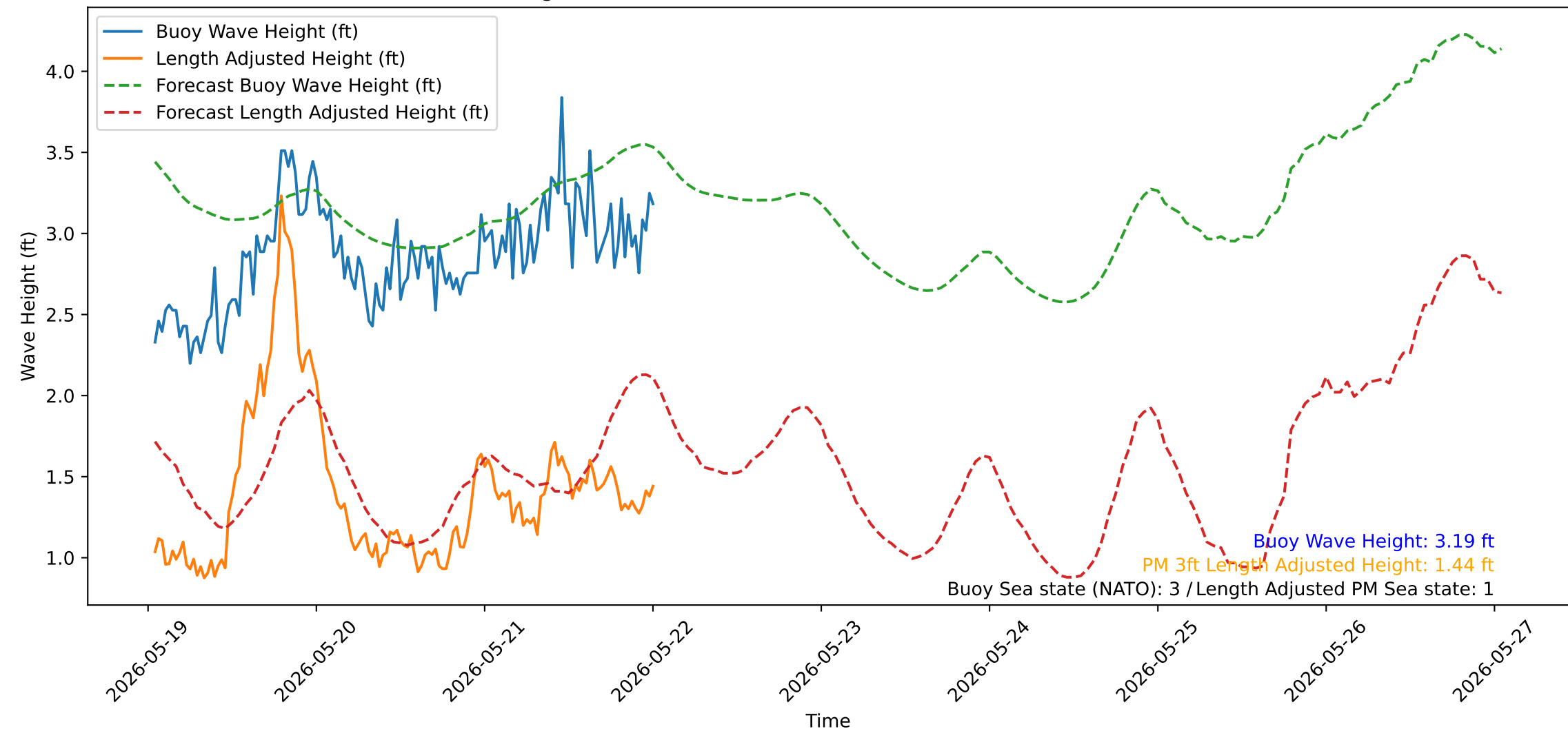
Wave Heights over Time for Oceanside Harbor at 2026-05-22 00:50:31
