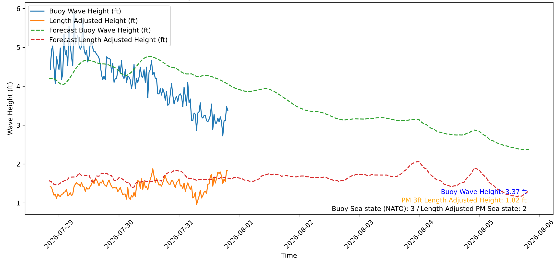
Wave Heights over Time for Oceanside Harbor at 2026-07-31 20:20:27
