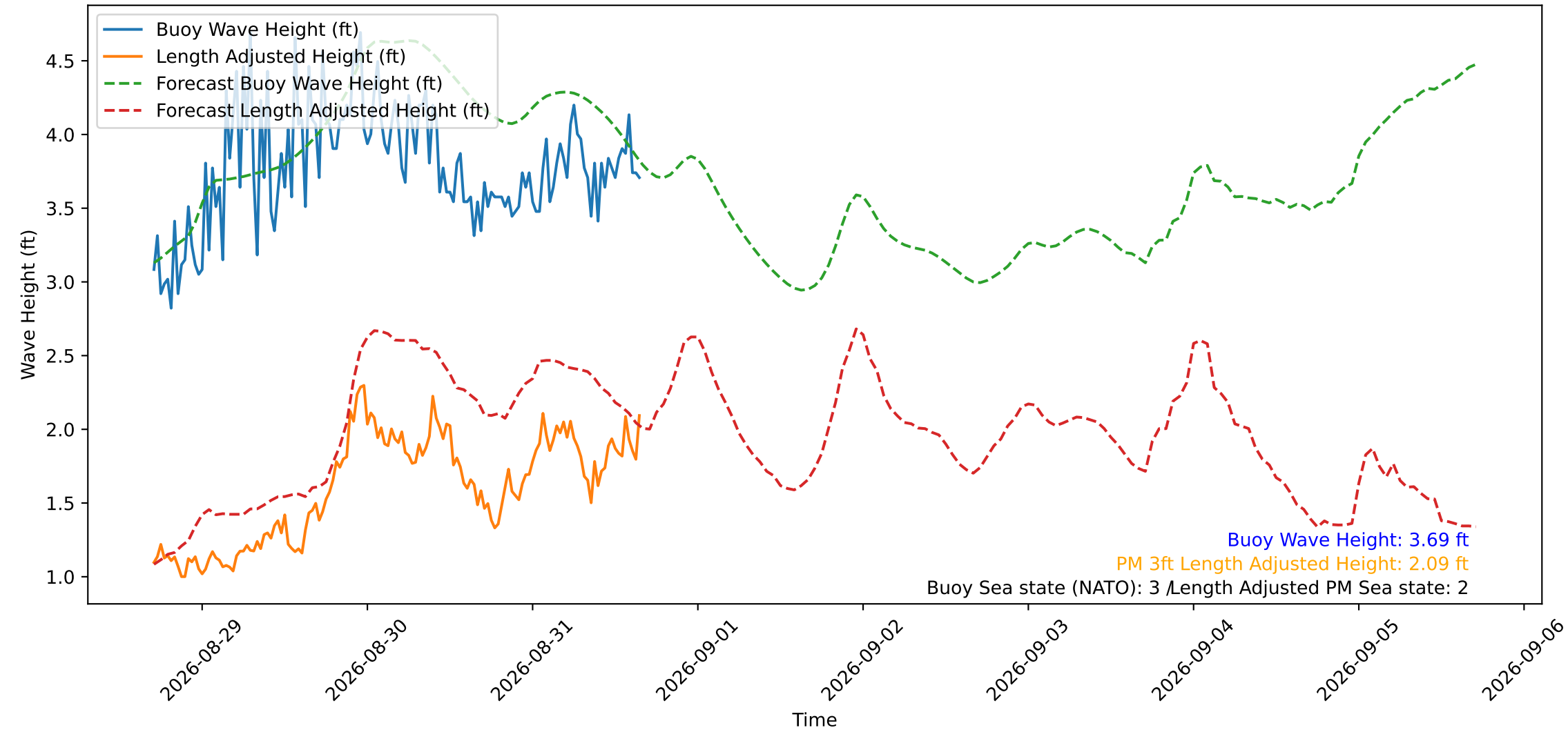
Wave Heights over Time for Red Beach at 2026-08-31 16:30:49
