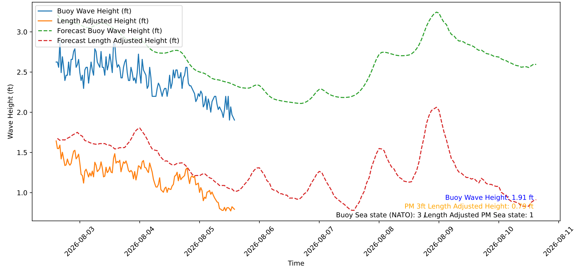
Wave Heights over Time for Oceanside Harbor at 2026-08-05 14:40:27
