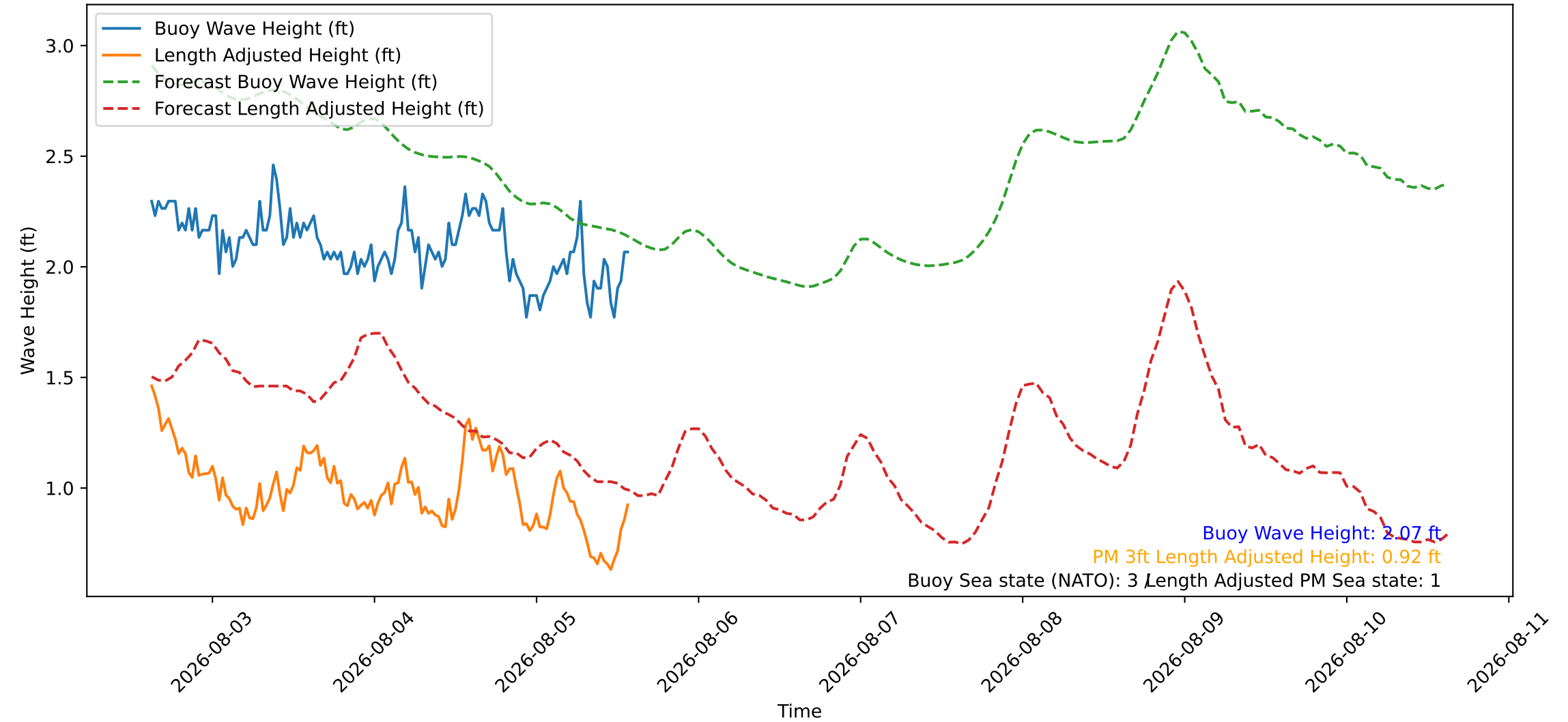
Wave Heights over Time for Red Beach at 2026-08-05 14:40:46
