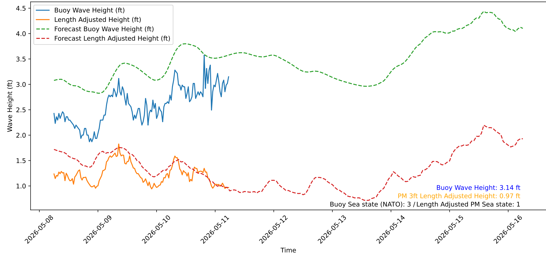
Wave Heights over Time for Oceanside Harbor at 2026-05-11 06:10:31
