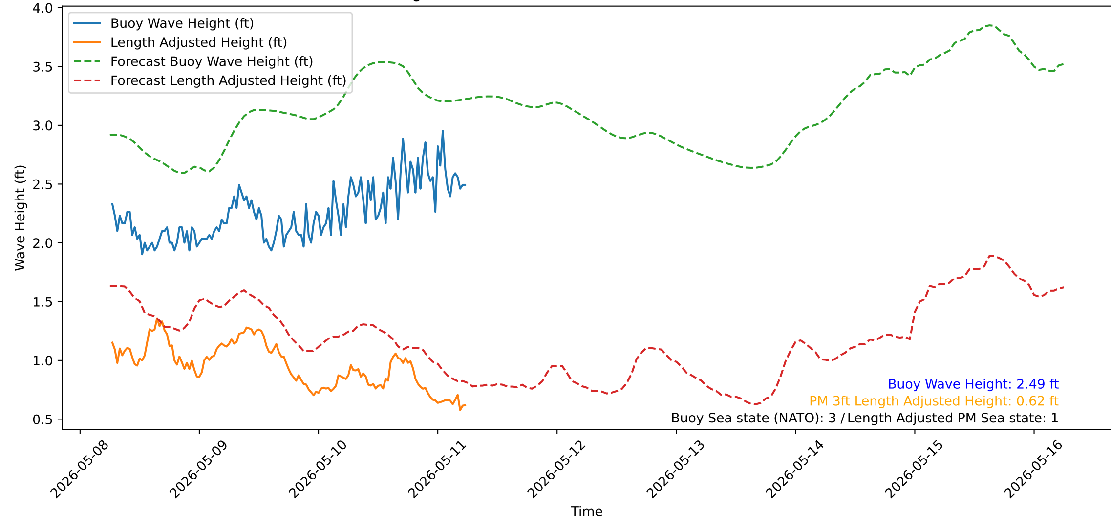
Wave Heights over Time for Red Beach at 2026-05-11 06:10:50
