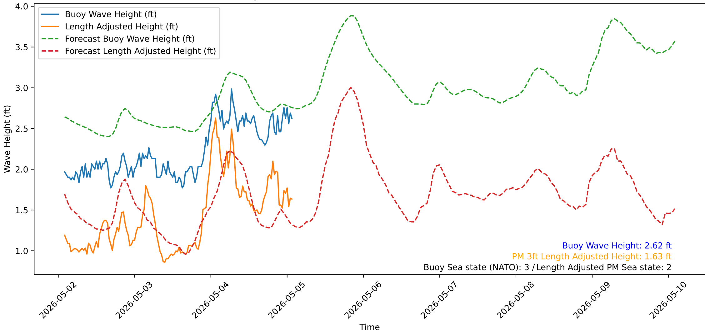
Wave Heights over Time for Green Beach at 2026-05-05 02:11:12
