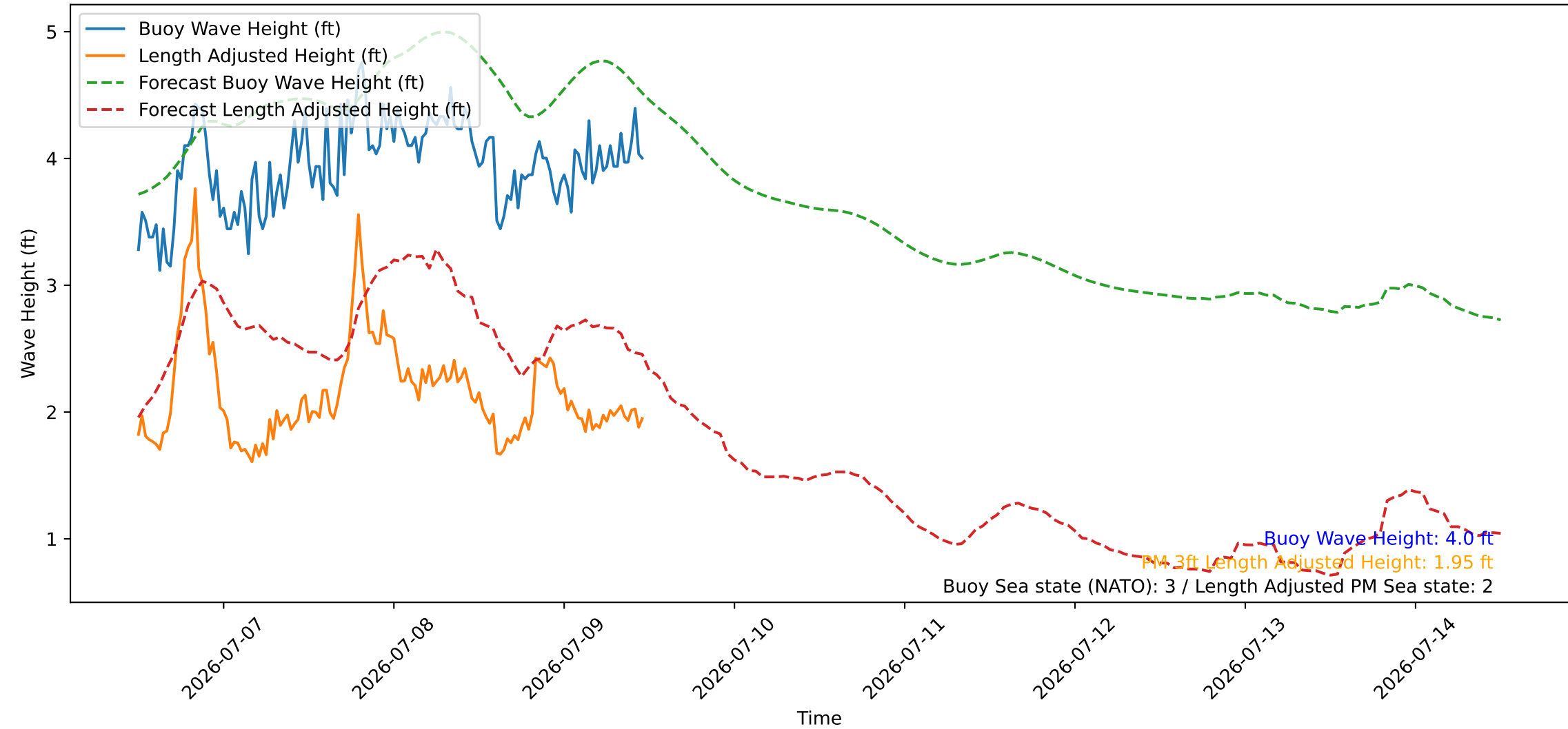
Wave Heights over Time for Green Beach at 2026-07-09 11:51:09
