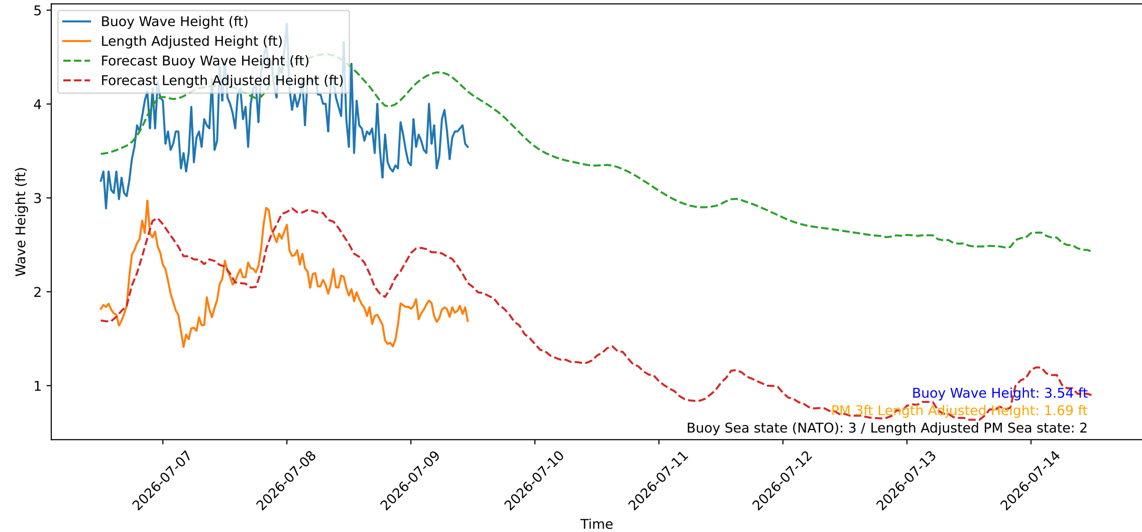
Wave Heights over Time for Red Beach at 2026-07-09 11:50:47
