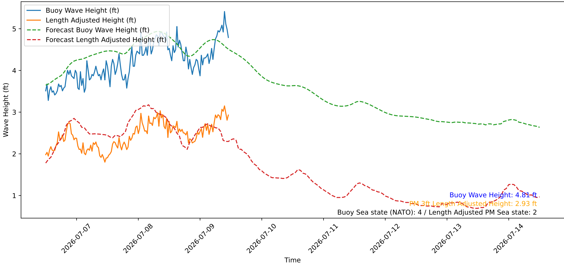
Wave Heights over Time for Oceanside Harbor at 2026-07-09 11:50:26
