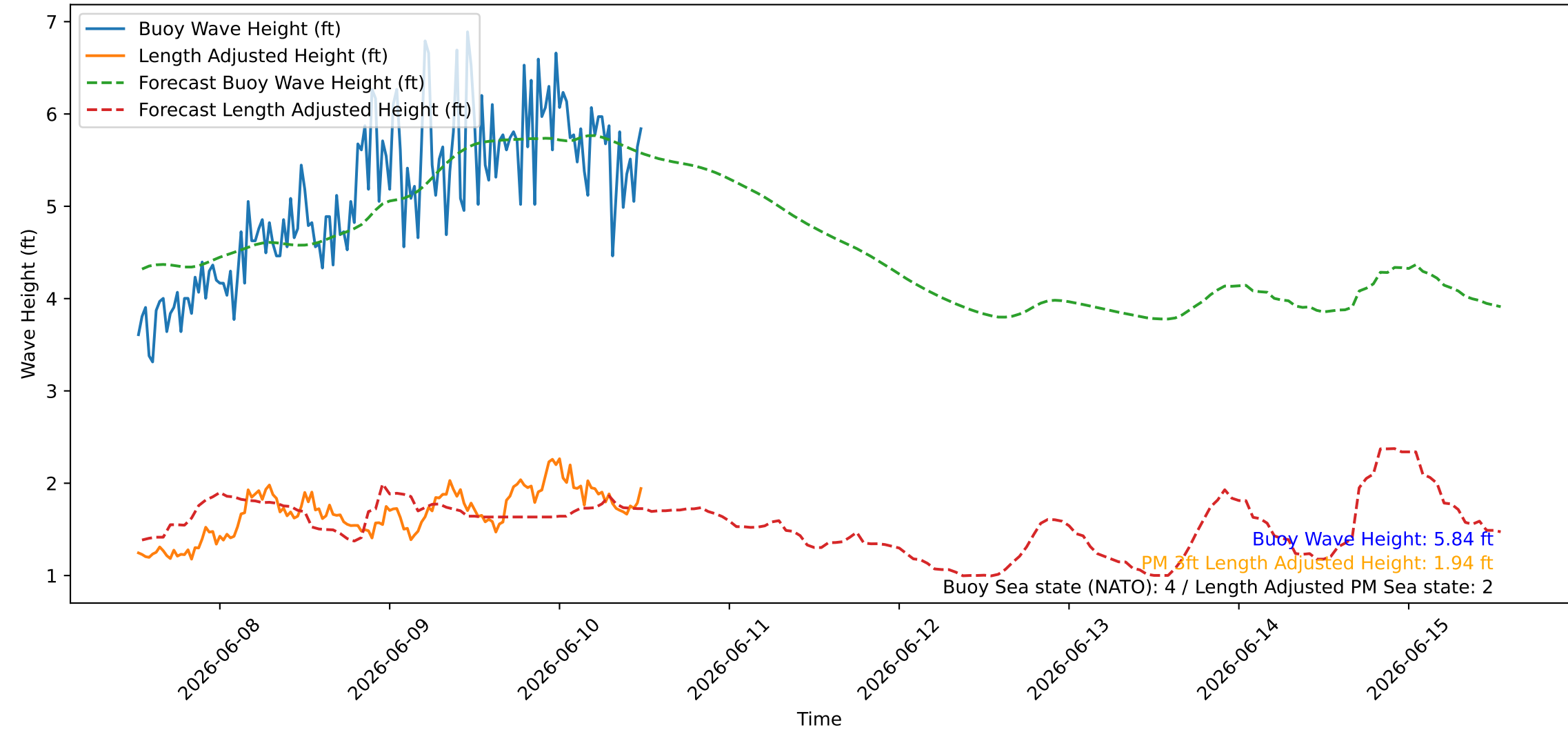
Wave Heights over Time for Green Beach at 2026-06-10 12:31:10
