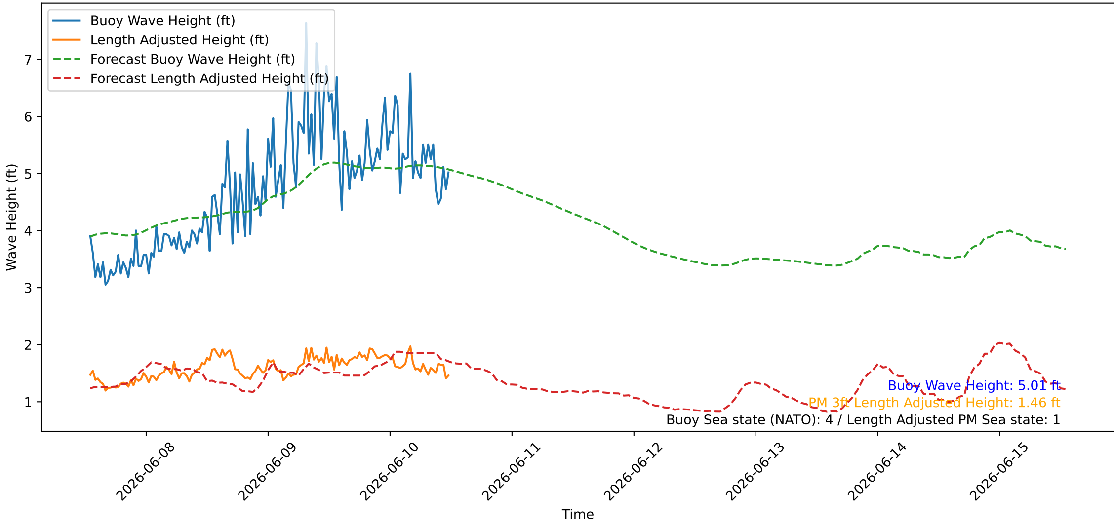
Wave Heights over Time for Red Beach at 2026-06-10 12:30:47
