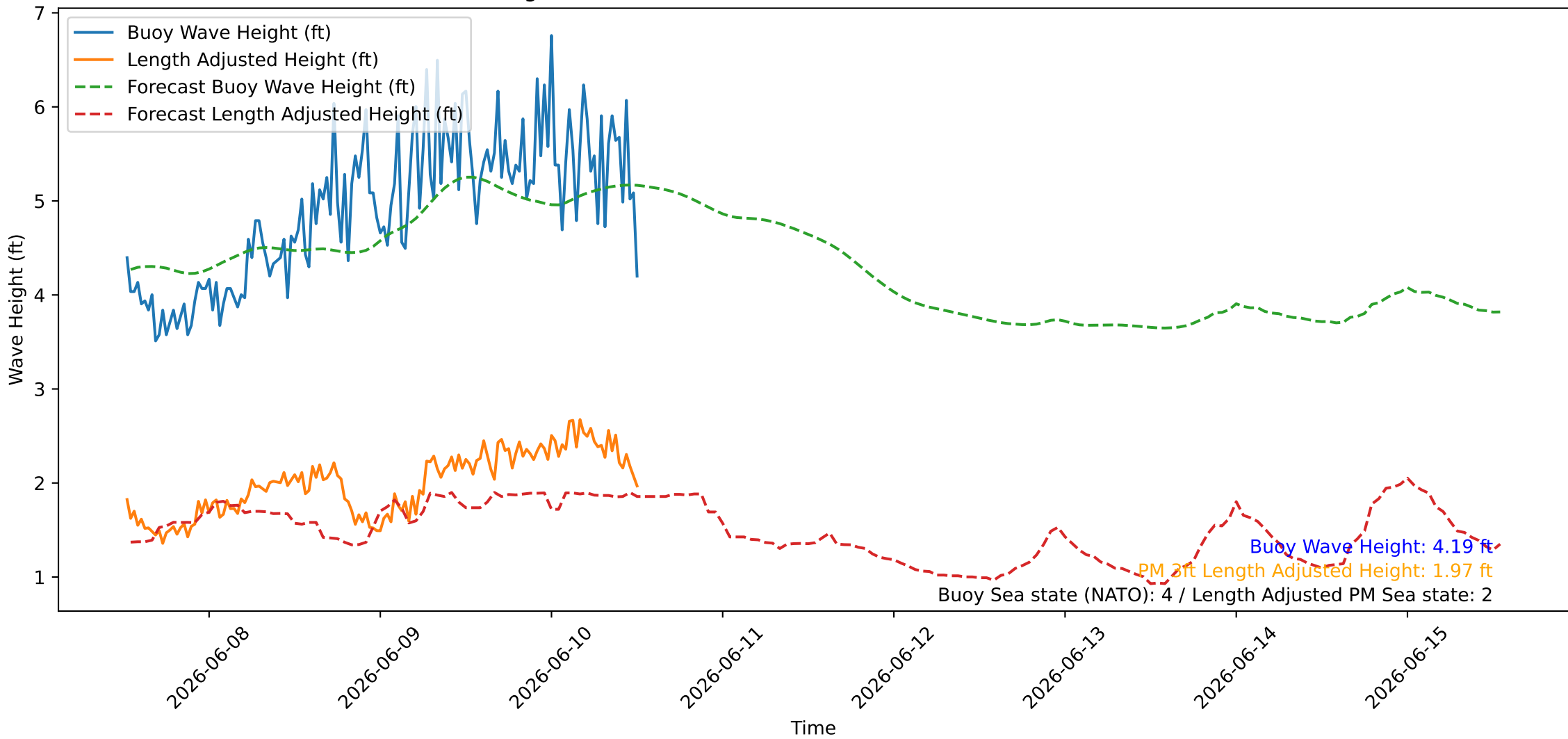
Wave Heights over Time for Oceanside Harbor at 2026-06-10 12:30:27
