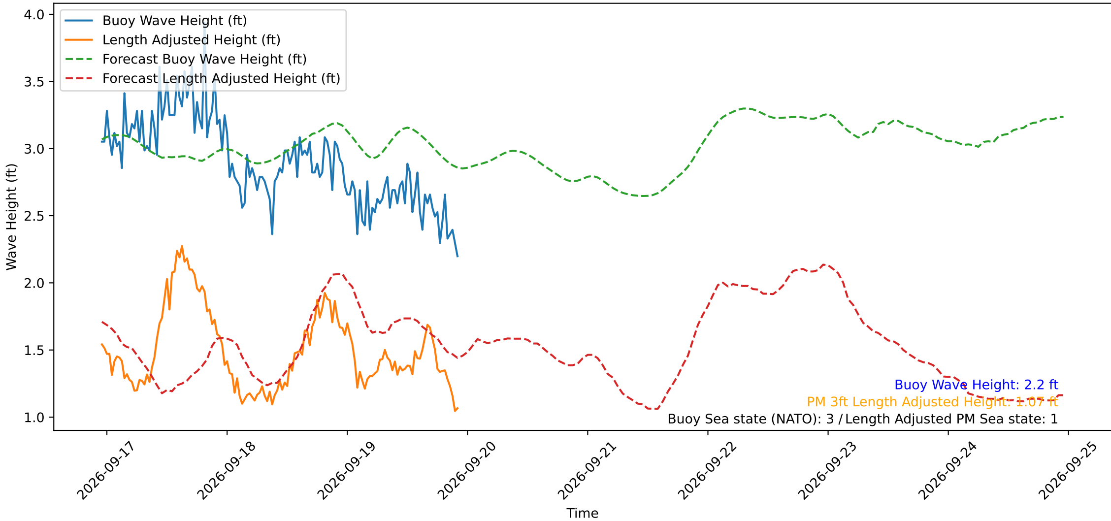
Wave Heights over Time for Oceanside Harbor at 2026-09-19 22:50:29
