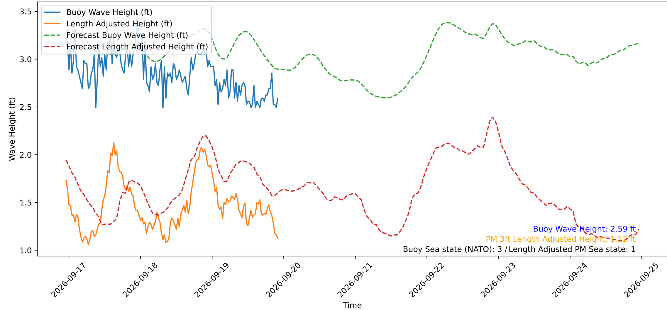
Wave Heights over Time for Green Beach at 2026-09-19 22:51:12
