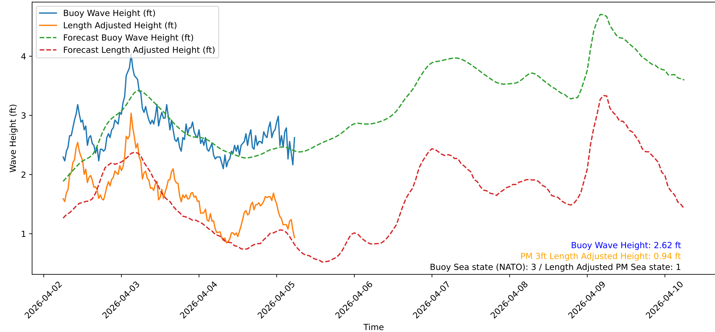
Wave Heights over Time for Oceanside Harbor at 2026-04-05 06:10:31
