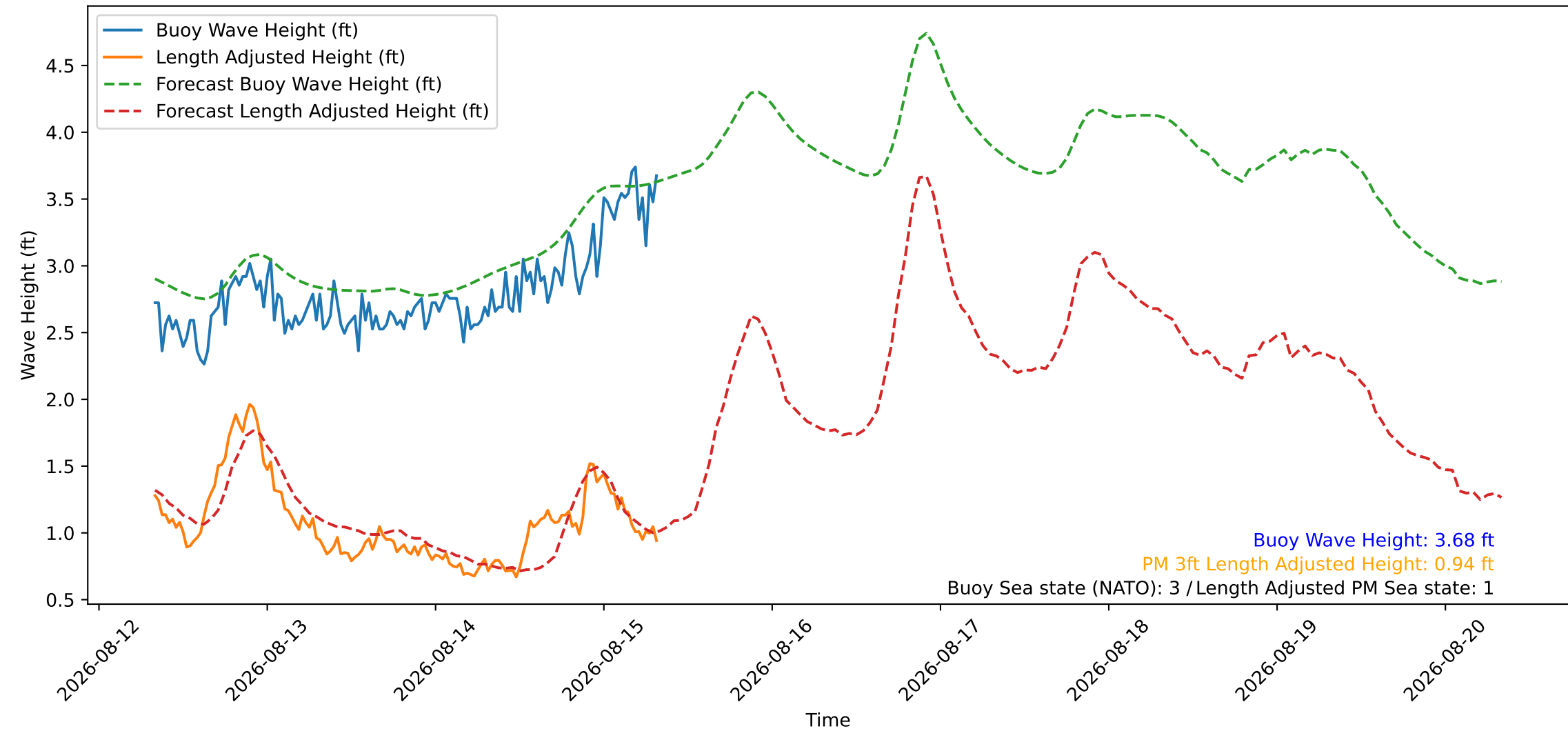
Wave Heights over Time for Green Beach at 2026-08-15 08:11:08
