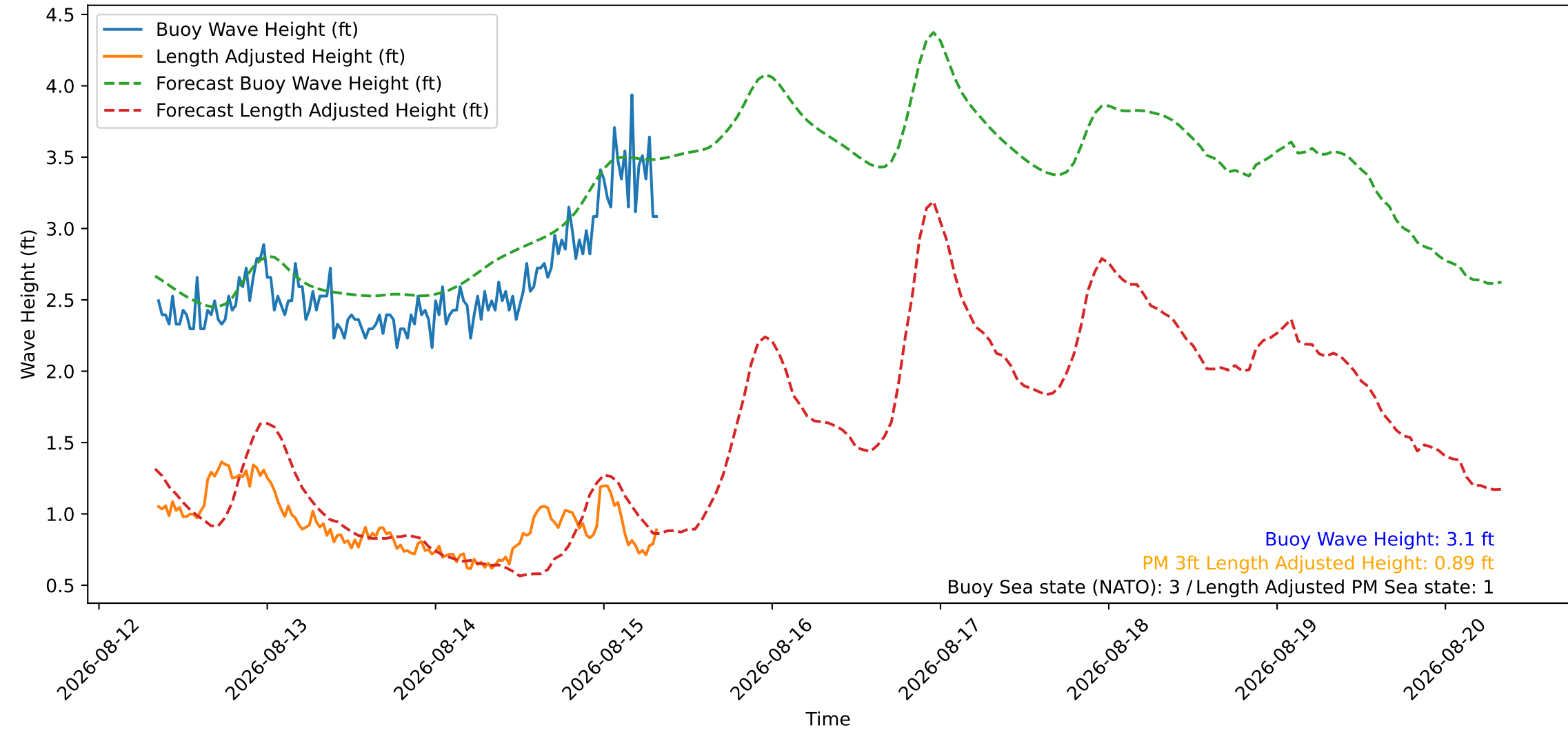
Wave Heights over Time for Red Beach at 2026-08-15 08:10:46
