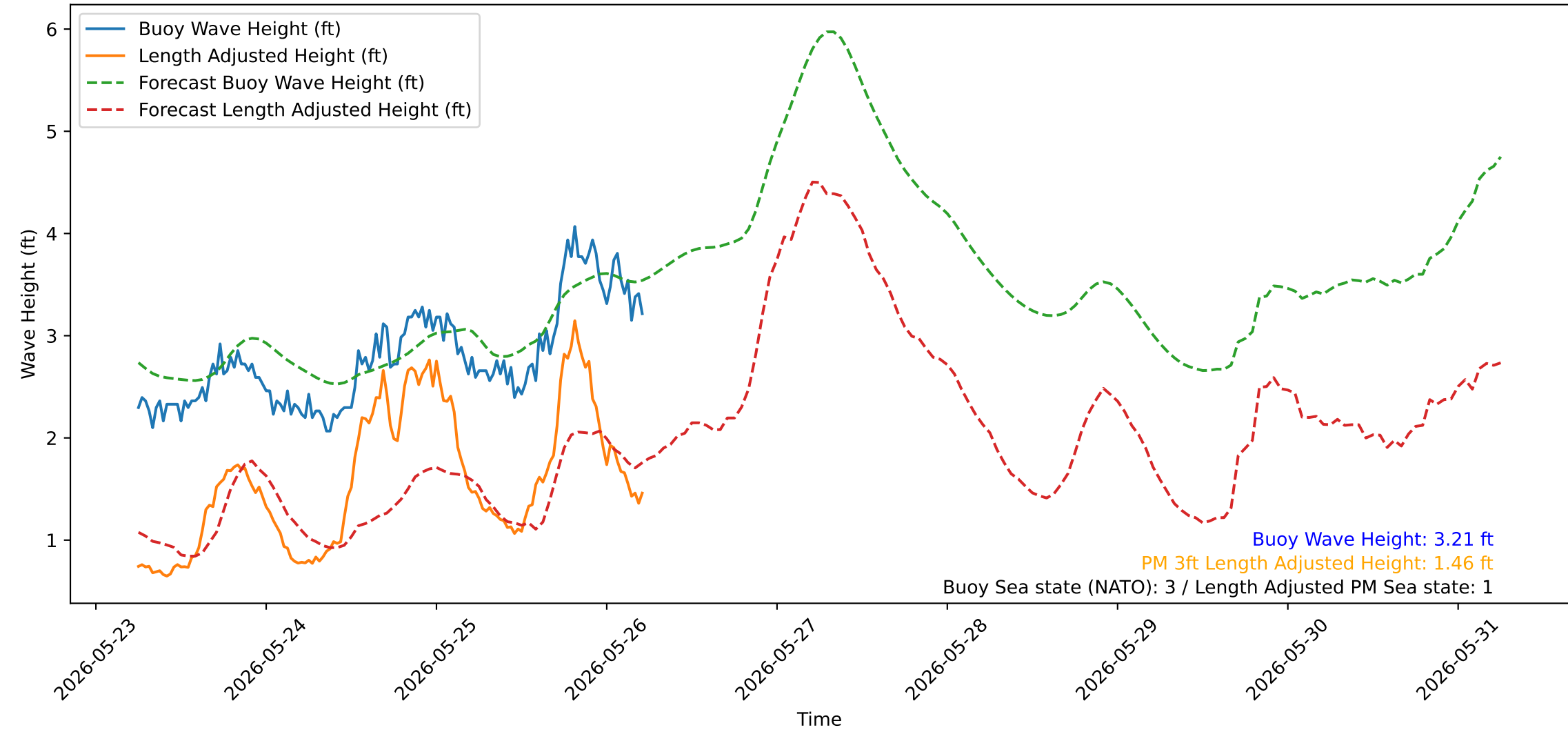
Wave Heights over Time for Green Beach at 2026-05-26 05:51:11
