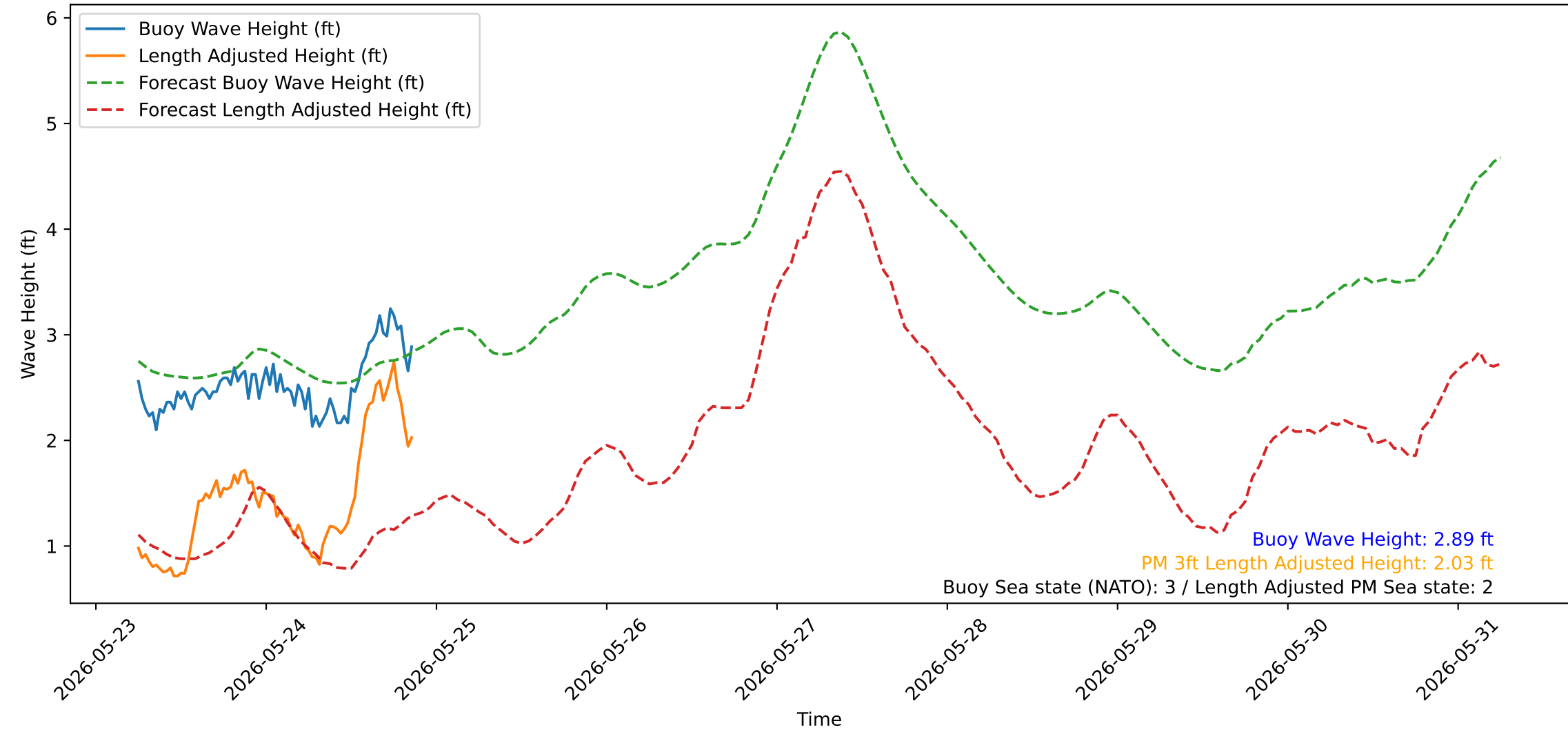
Wave Heights over Time for Oceanside Harbor at 2026-05-26 05:50:28
