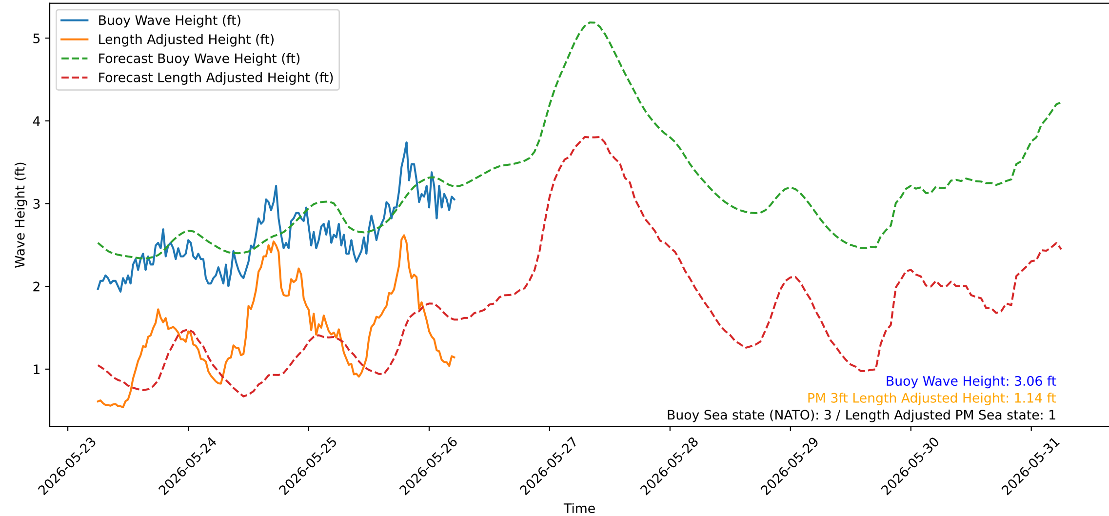
Wave Heights over Time for Red Beach at 2026-05-26 05:50:49
