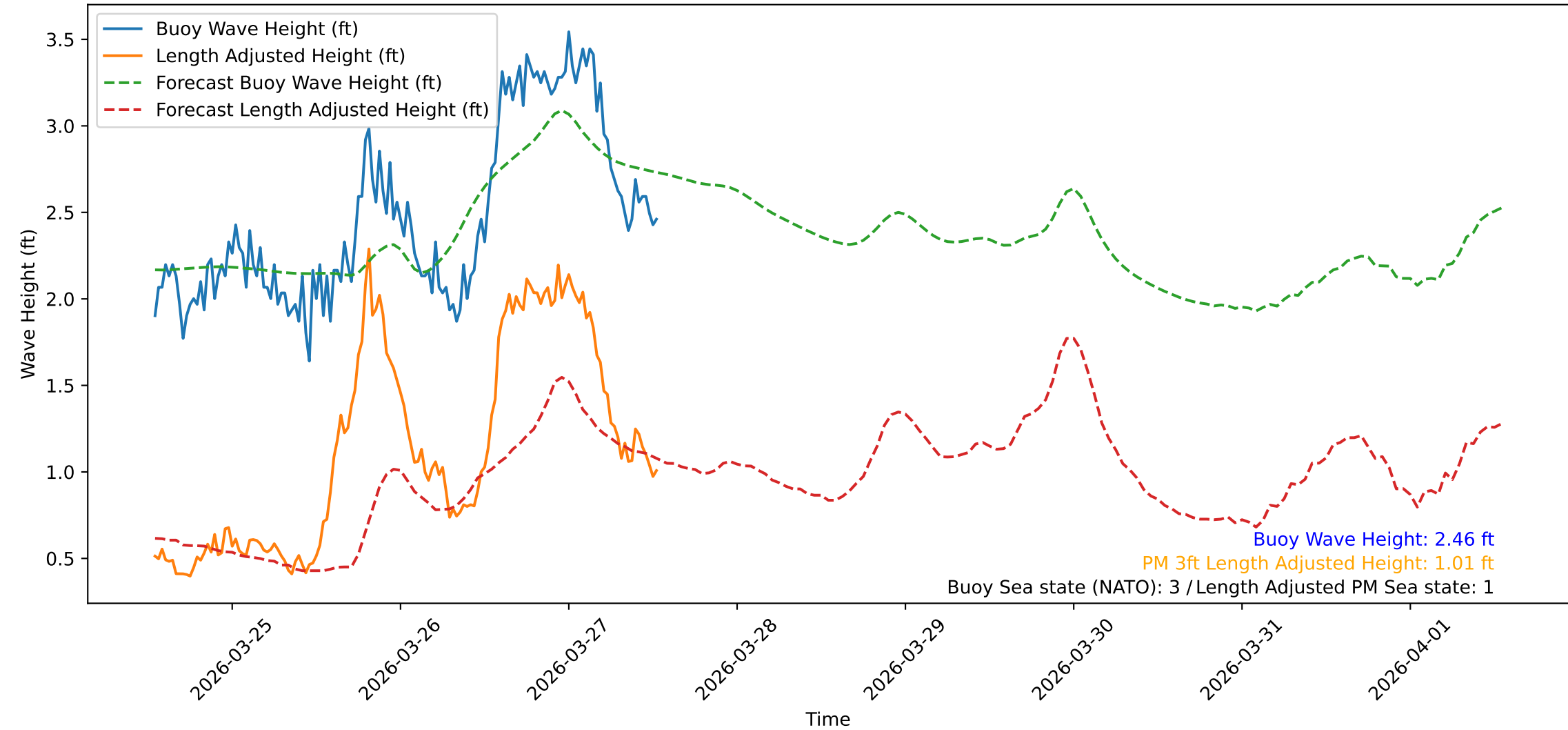
Wave Heights over Time for Green Beach at 2026-03-27 13:11:10
