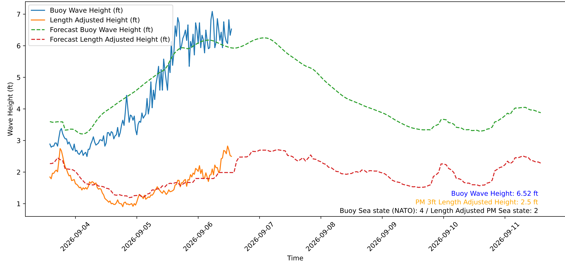
Wave Heights over Time for Green Beach at 2026-09-06 13:51:14
