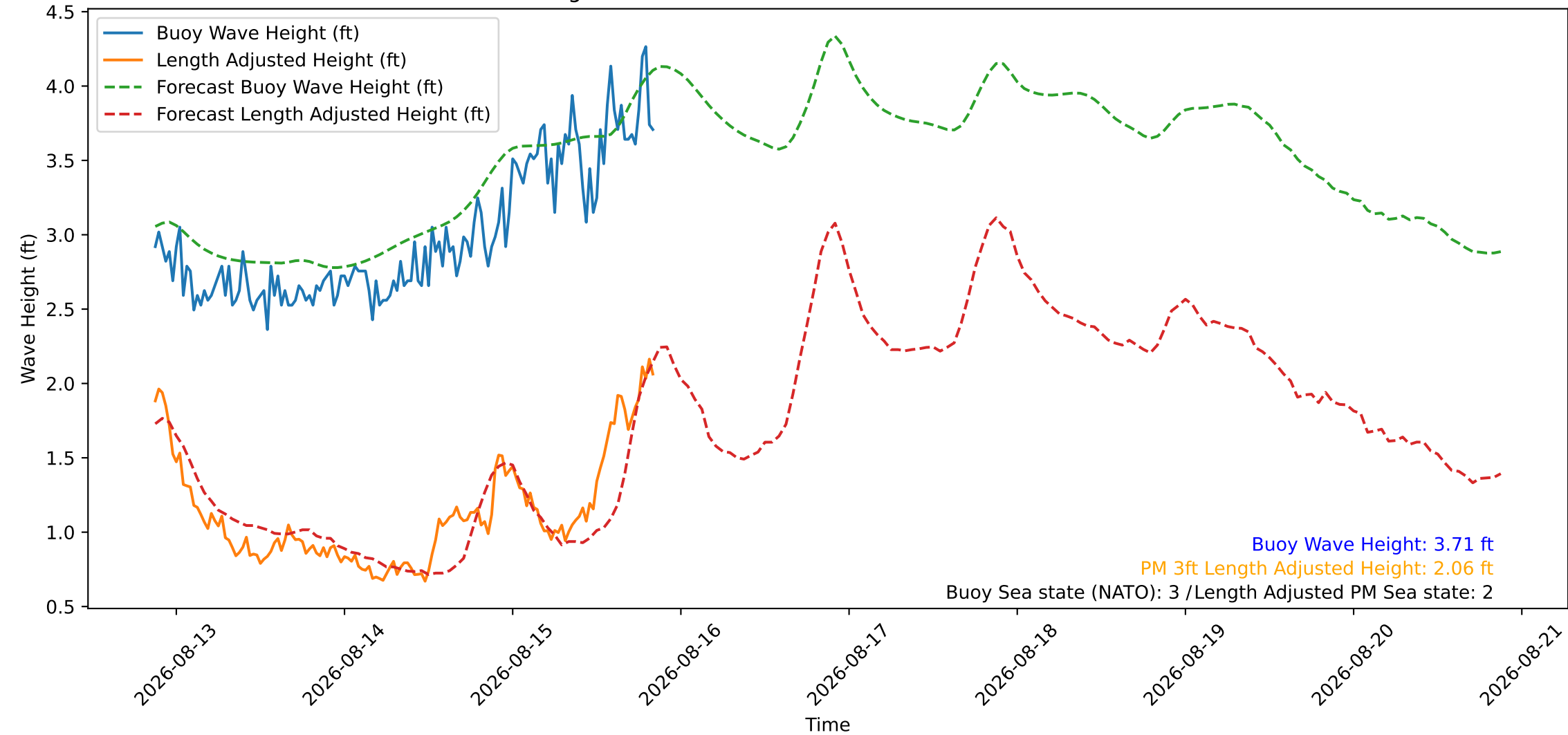
Wave Heights over Time for Green Beach at 2026-08-15 20:51:11
