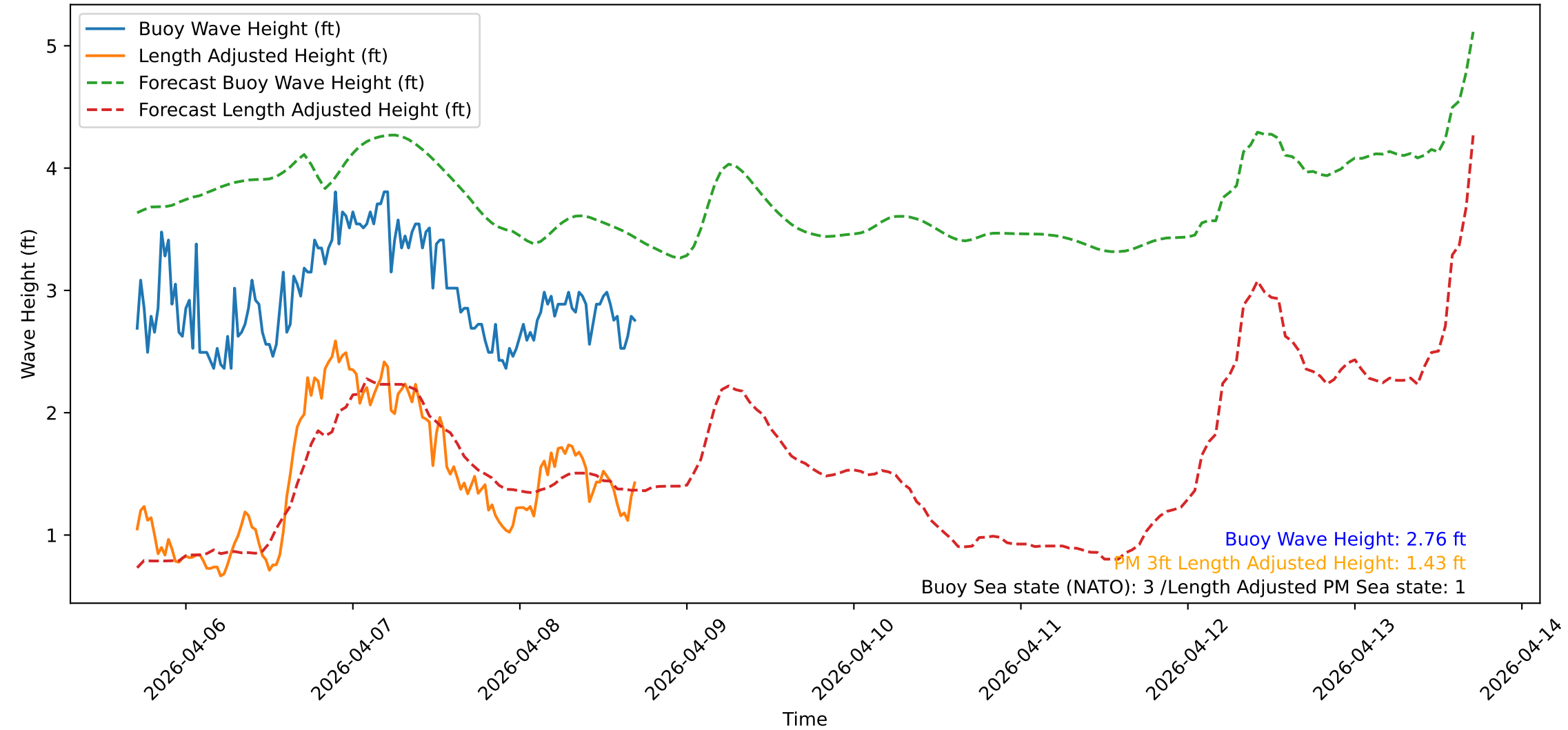
Wave Heights over Time for Green Beach at 2026-04-08 17:11:09
