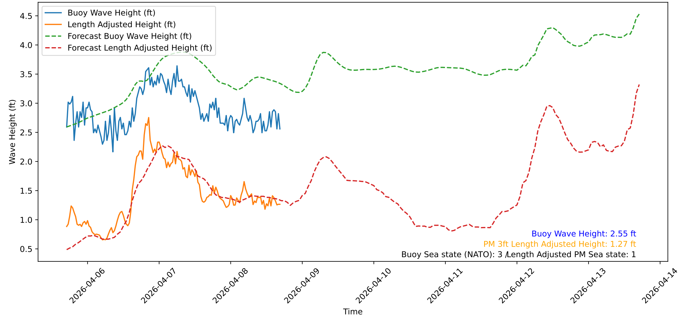
Wave Heights over Time for Oceanside Harbor at 2026-04-08 17:10:31
