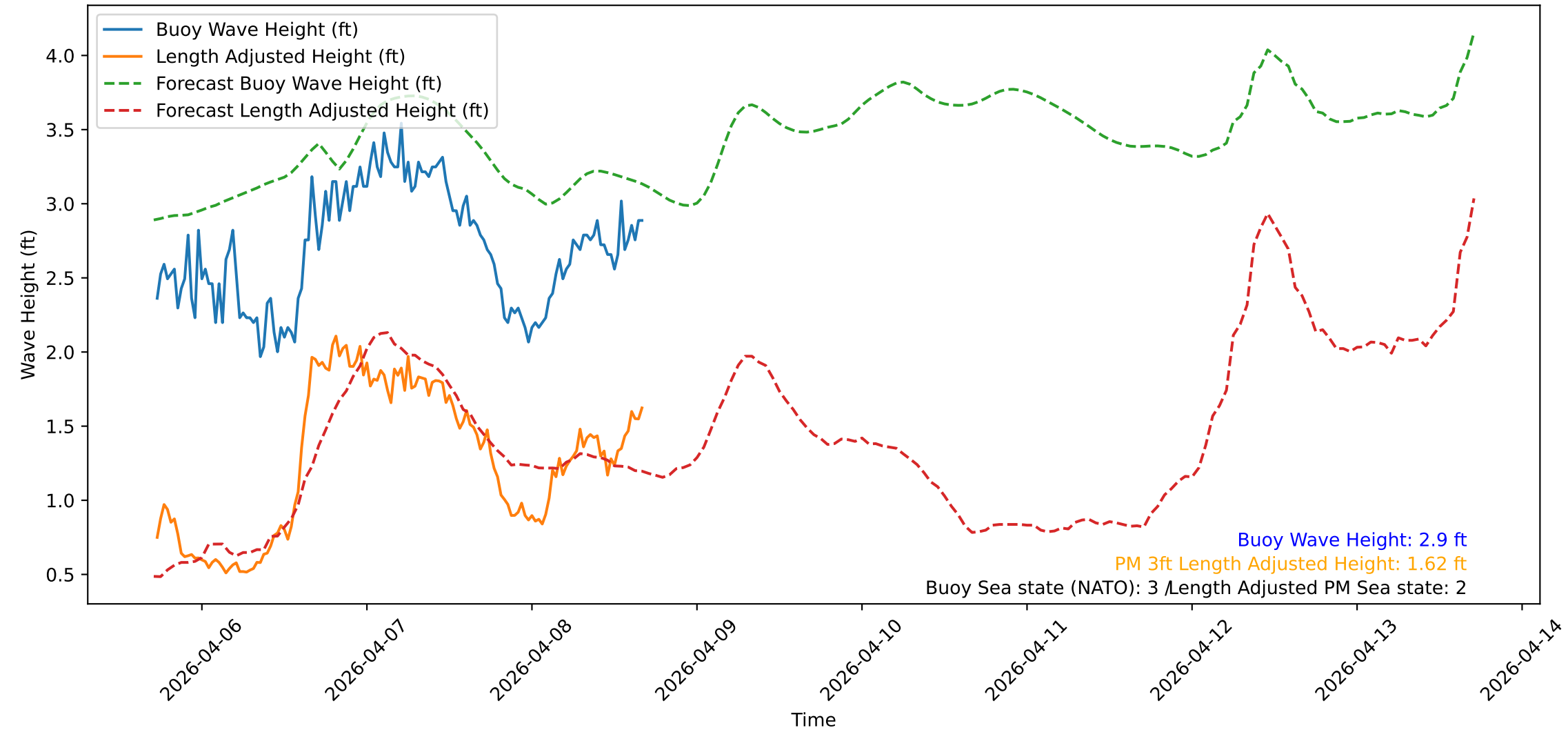
Wave Heights over Time for Red Beach at 2026-04-08 17:10:47
