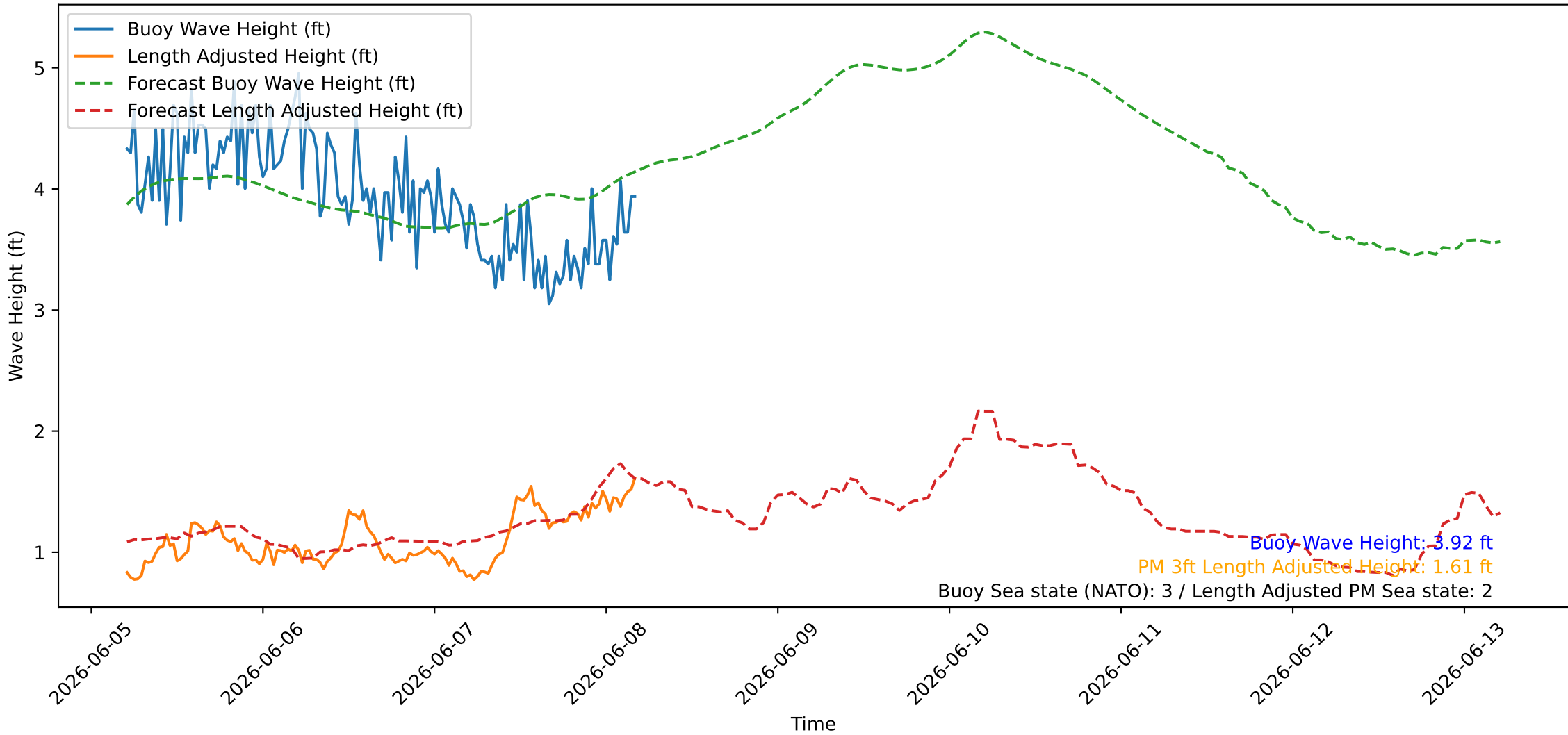
Wave Heights over Time for Red Beach at 2026-06-08 04:50:48
