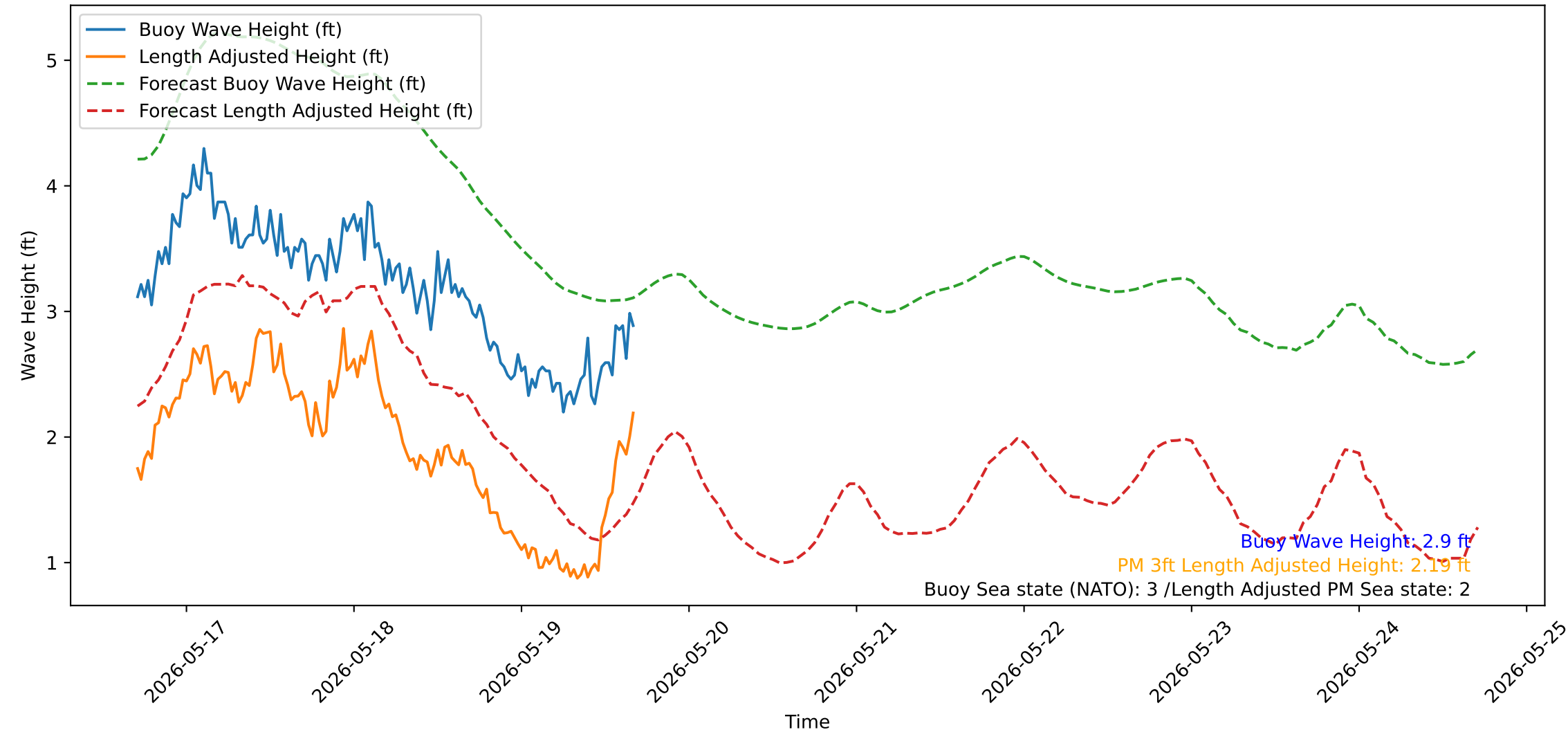
Wave Heights over Time for Oceanside Harbor at 2026-05-19 17:00:31
