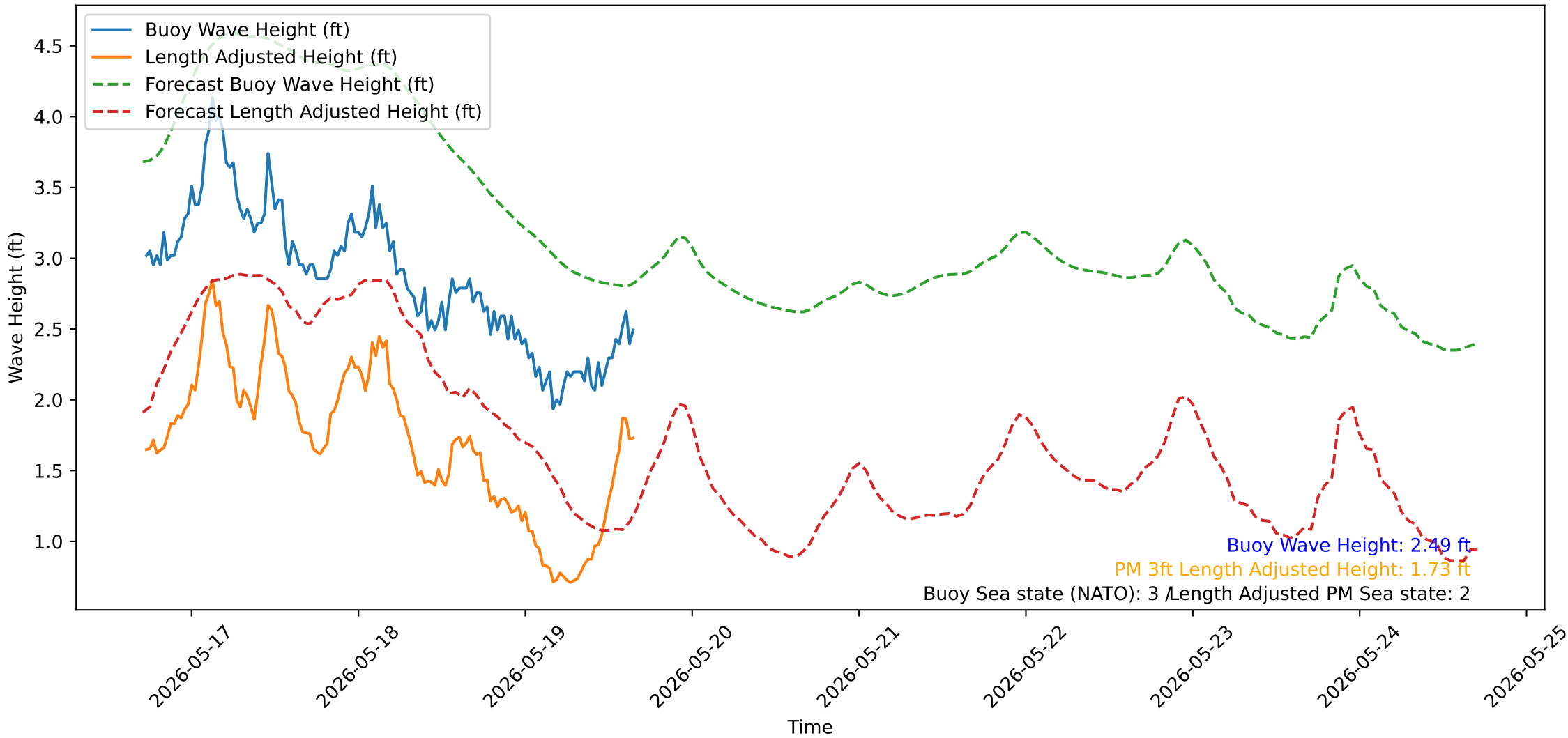
Wave Heights over Time for Red Beach at 2026-05-19 17:00:50
