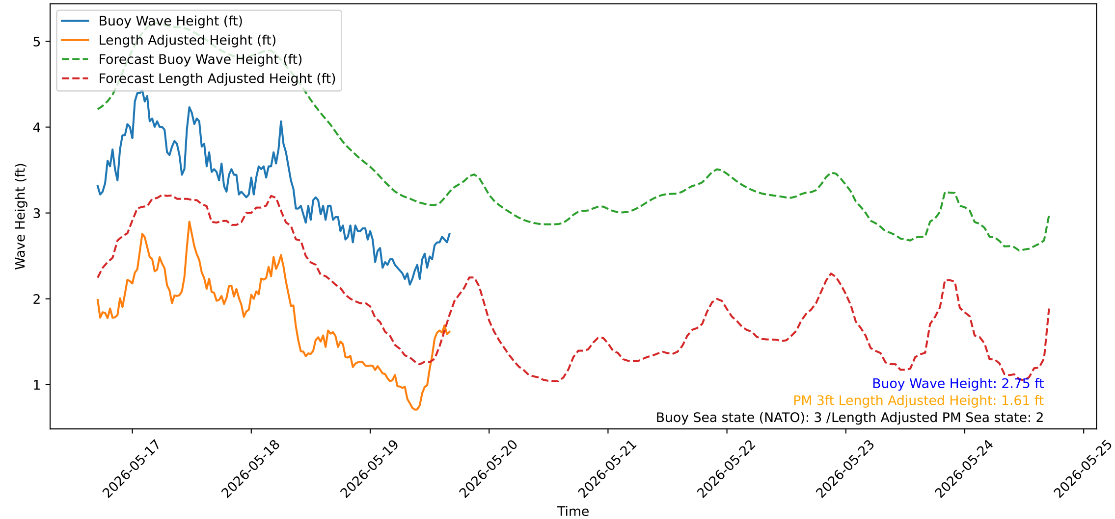
Wave Heights over Time for Green Beach at 2026-05-19 17:01:13
