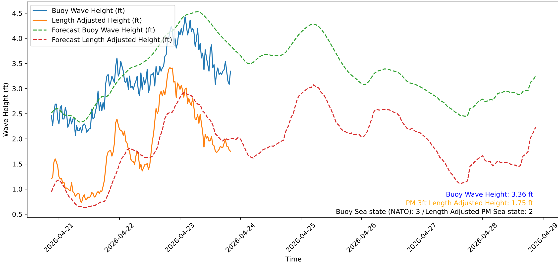
Wave Heights over Time for Oceanside Harbor at 2026-04-23 20:50:31
