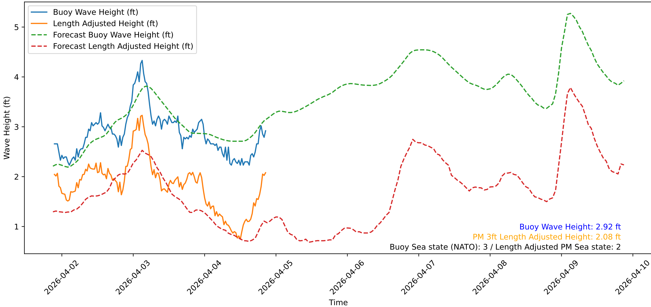
Wave Heights over Time for Green Beach at 2026-04-04 21:21:28
