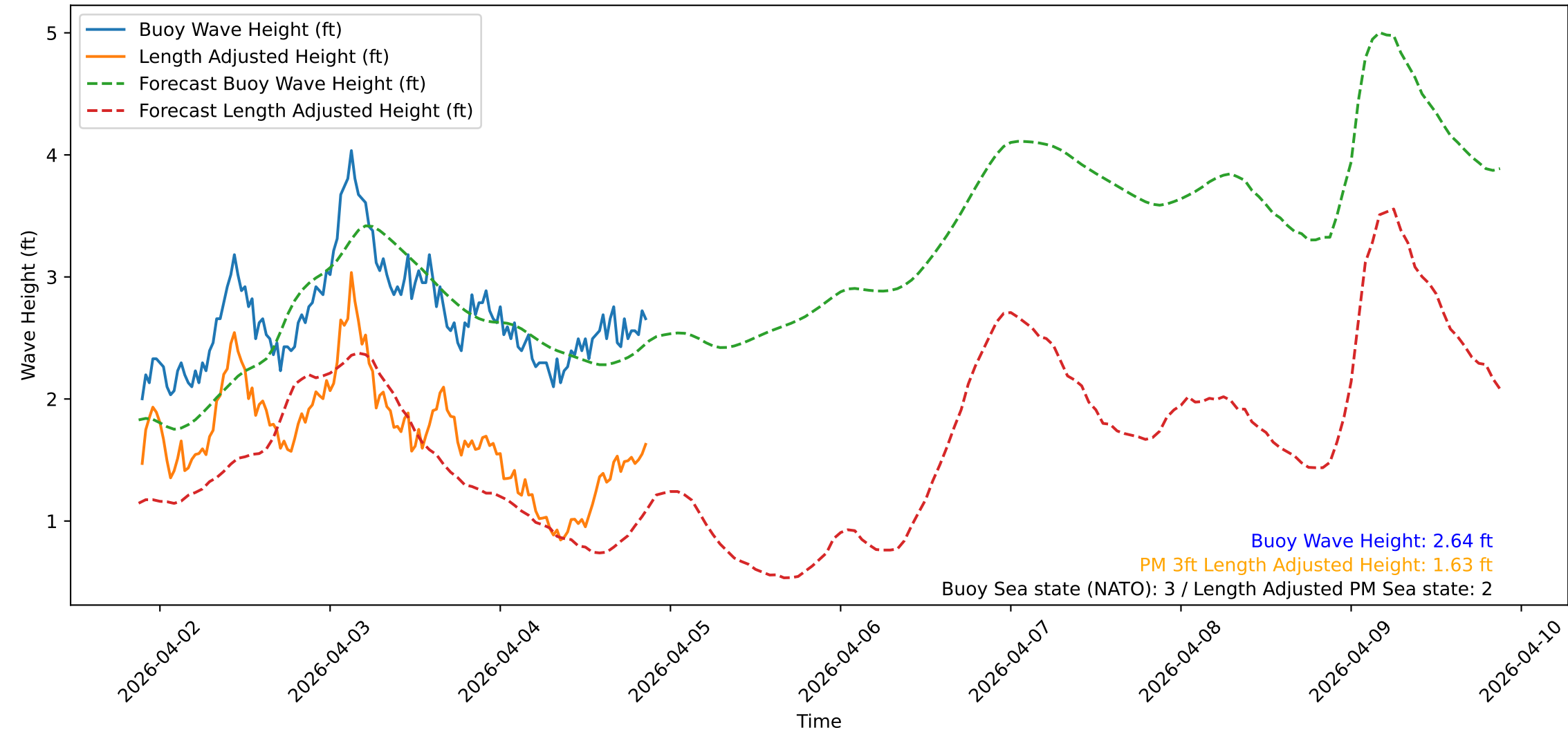
Wave Heights over Time for Oceanside Harbor at 2026-04-04 21:20:38
