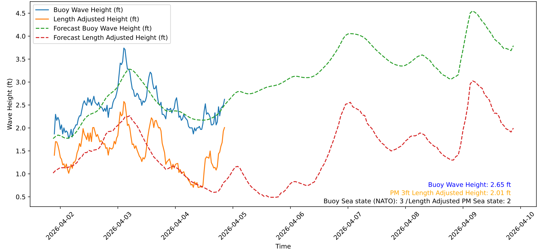
Wave Heights over Time for Red Beach at 2026-04-04 21:20:59
