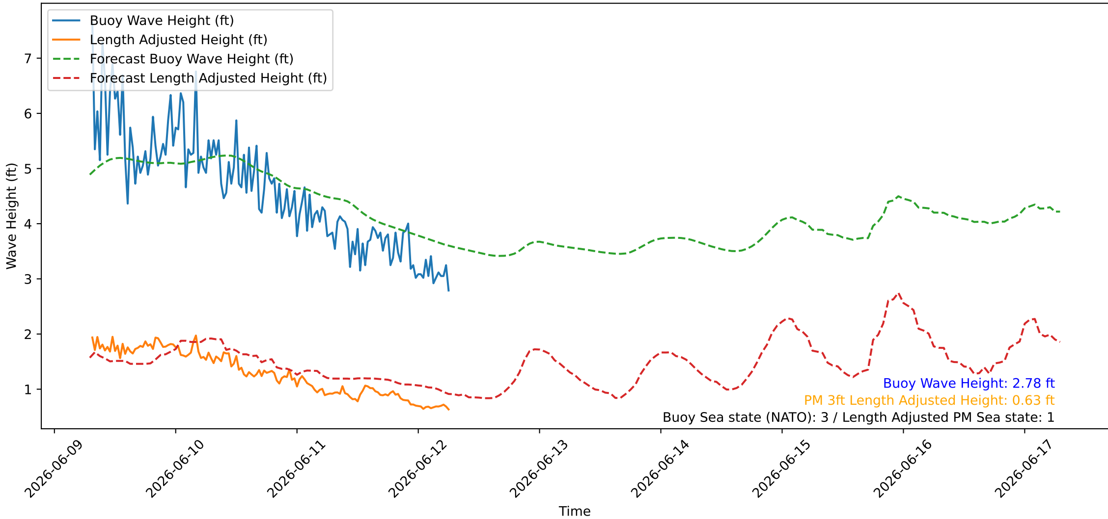
Wave Heights over Time for Red Beach at 2026-06-12 07:00:46
