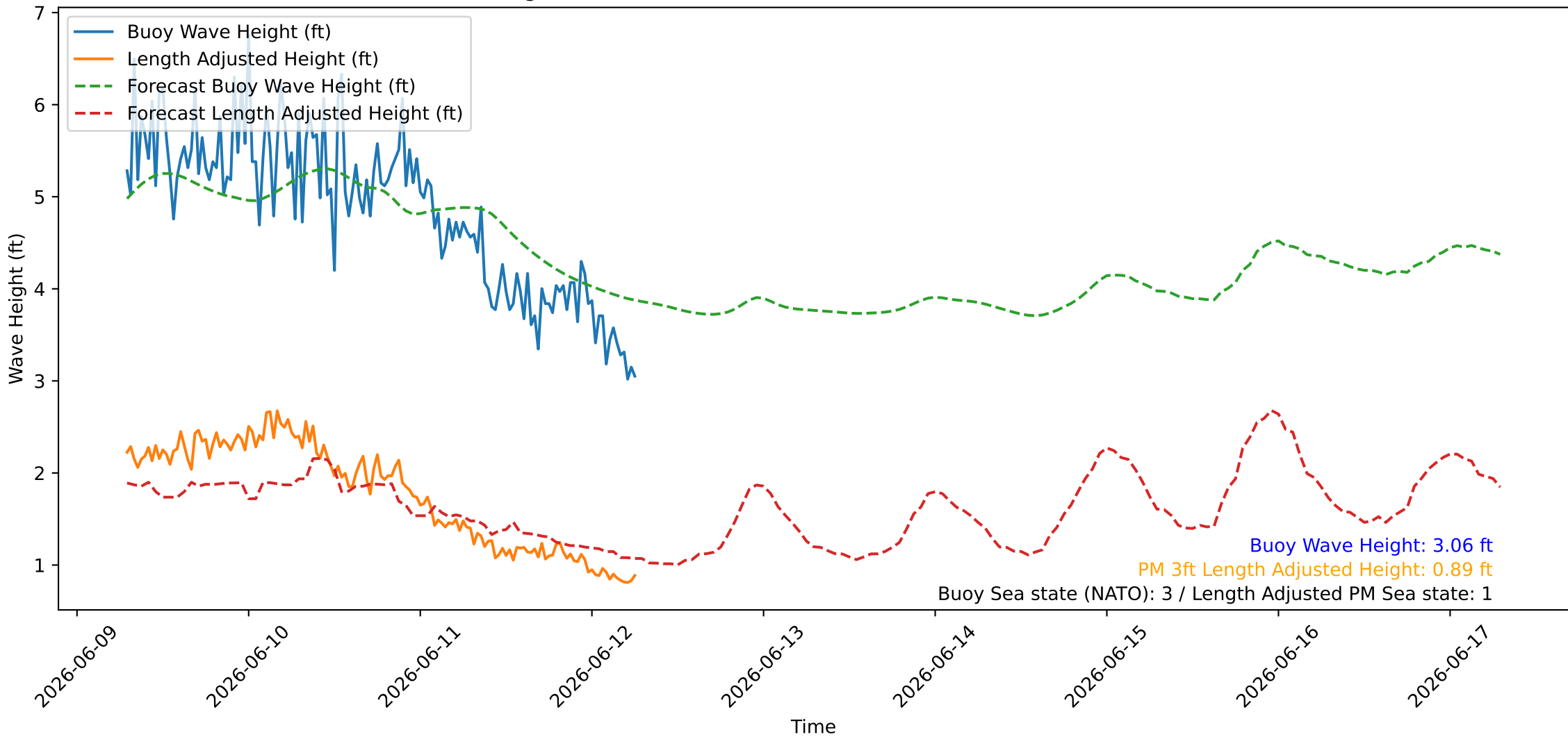
Wave Heights over Time for Oceanside Harbor at 2026-06-12 07:00:26
