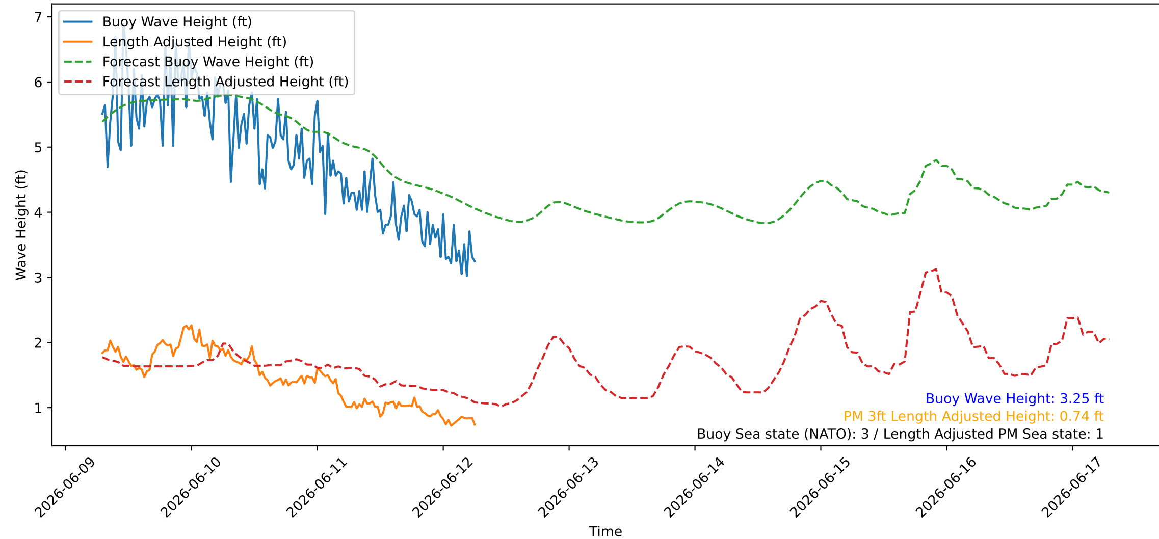
Wave Heights over Time for Green Beach at 2026-06-12 07:01:09
