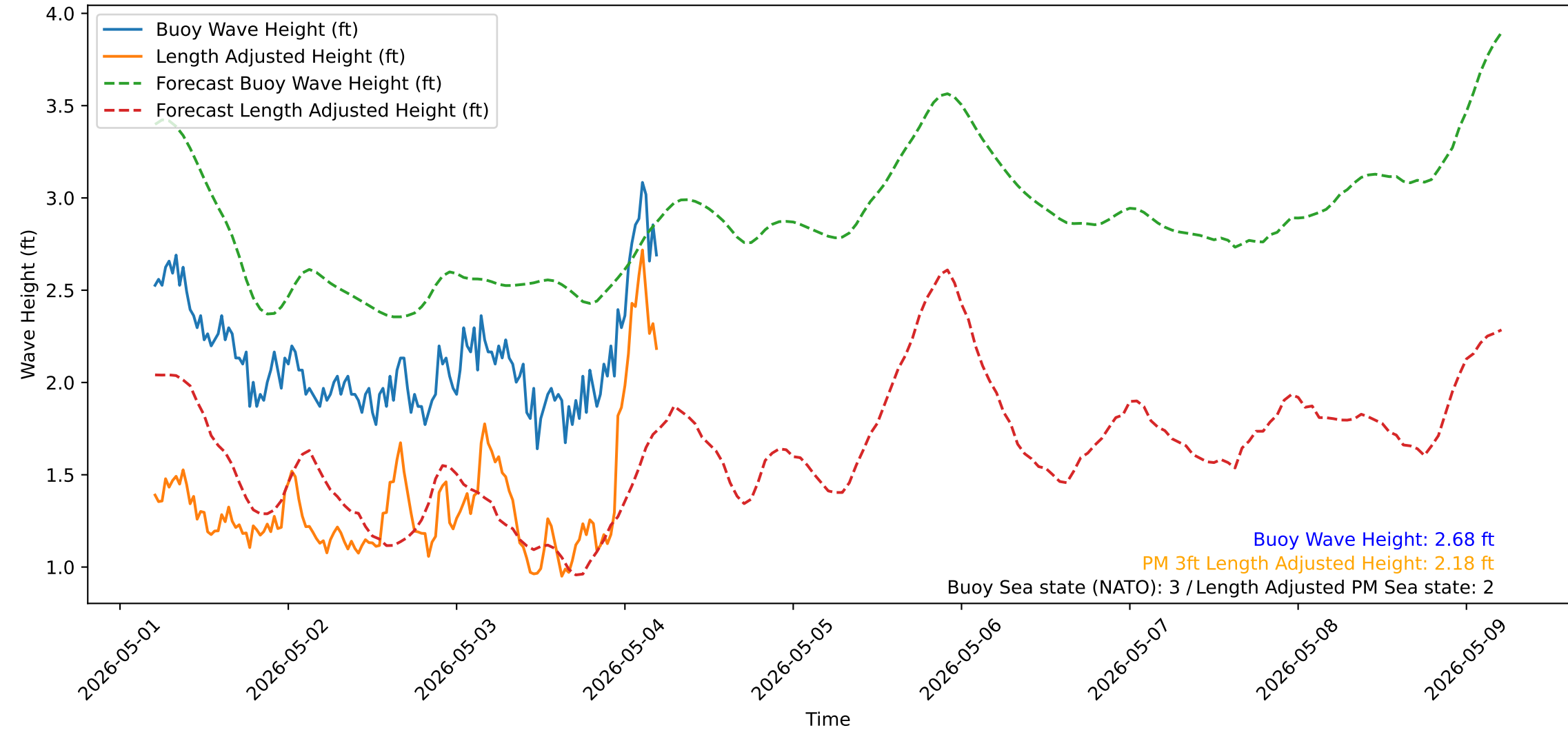
Wave Heights over Time for Oceanside Harbor at 2026-05-04 05:10:31
