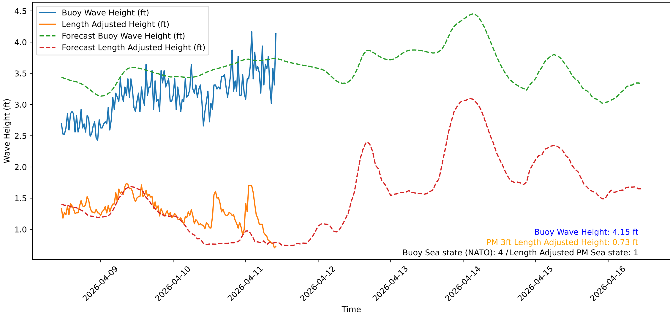
Wave Heights over Time for Oceanside Harbor at 2026-04-11 10:50:31
