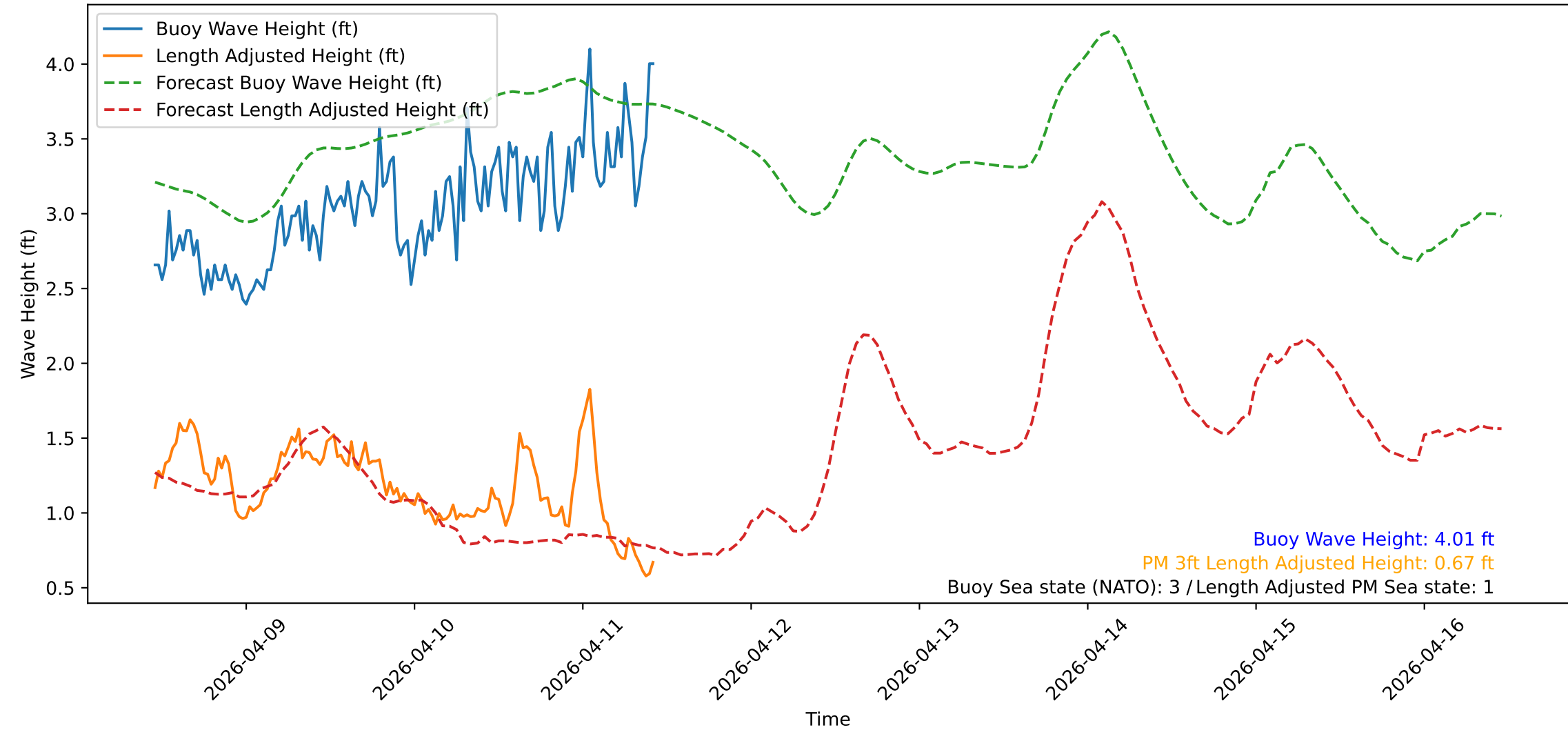
Wave Heights over Time for Red Beach at 2026-04-11 10:50:52
