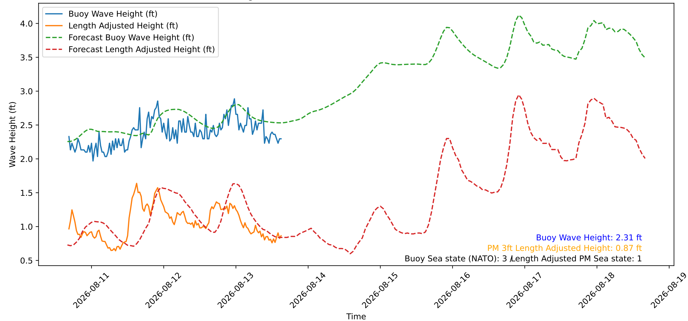
Wave Heights over Time for Red Beach at 2026-08-13 16:20:47
