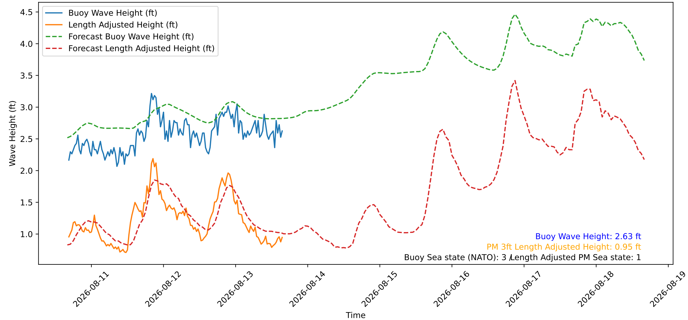
Wave Heights over Time for Green Beach at 2026-08-13 16:21:11
