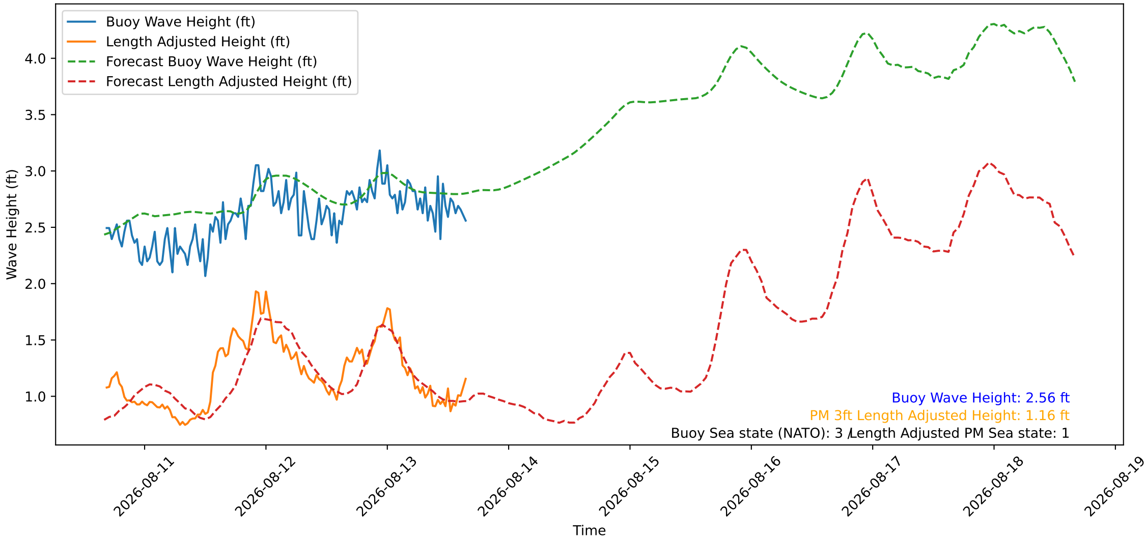
Wave Heights over Time for Oceanside Harbor at 2026-08-13 16:20:27
