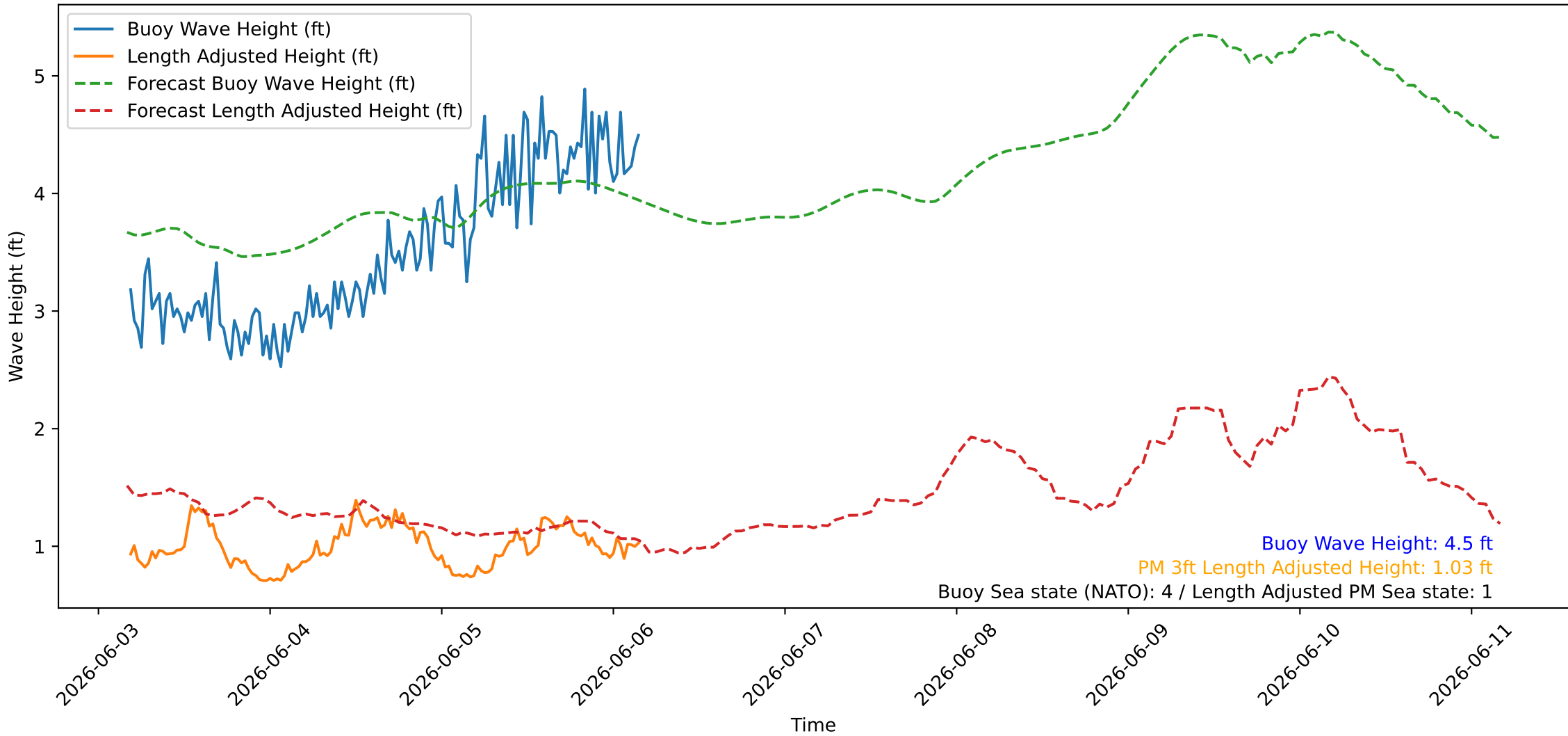
Wave Heights over Time for Red Beach at 2026-06-06 04:10:46
