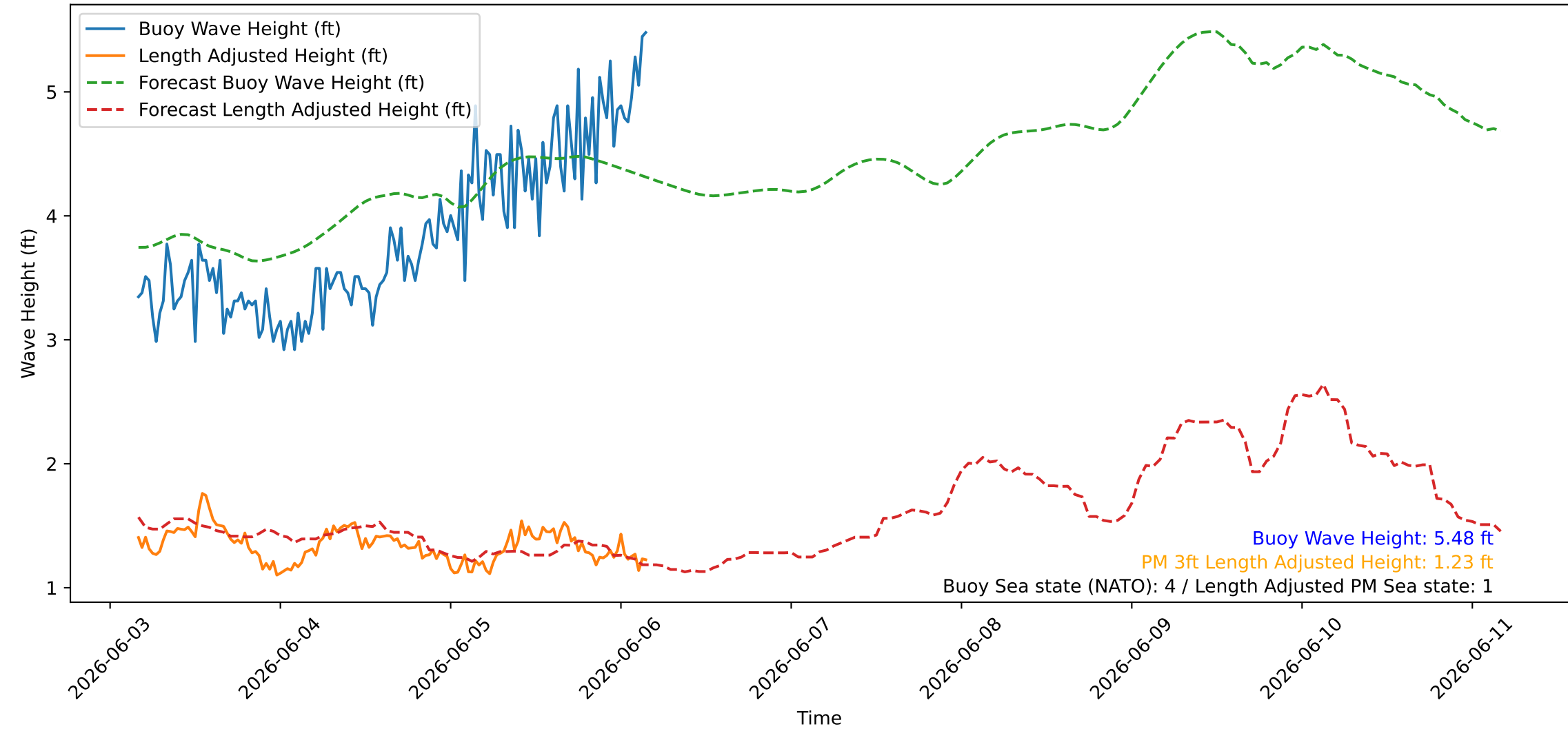
Wave Heights over Time for Oceanside Harbor at 2026-06-06 04:10:26
