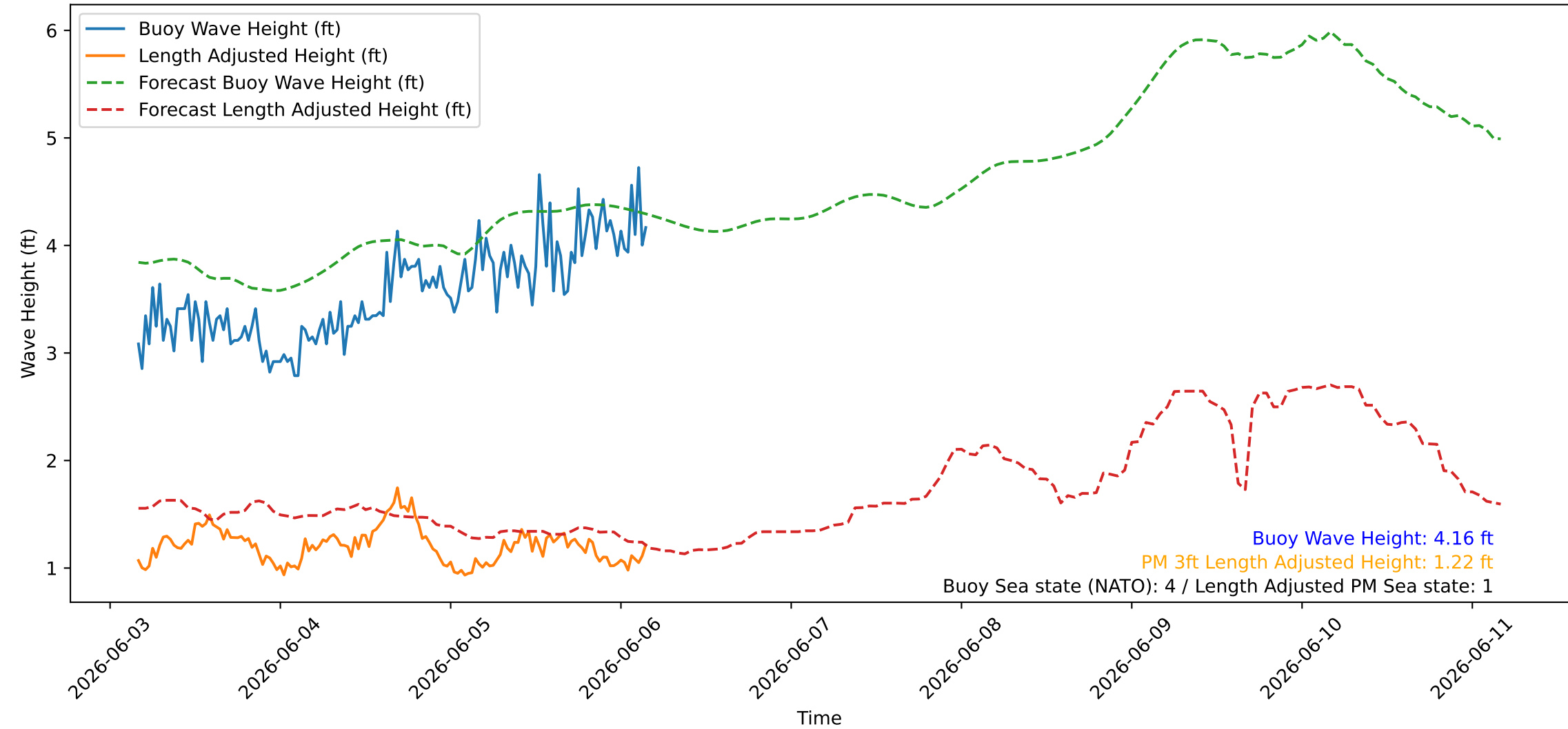
Wave Heights over Time for Green Beach at 2026-06-06 04:11:08
