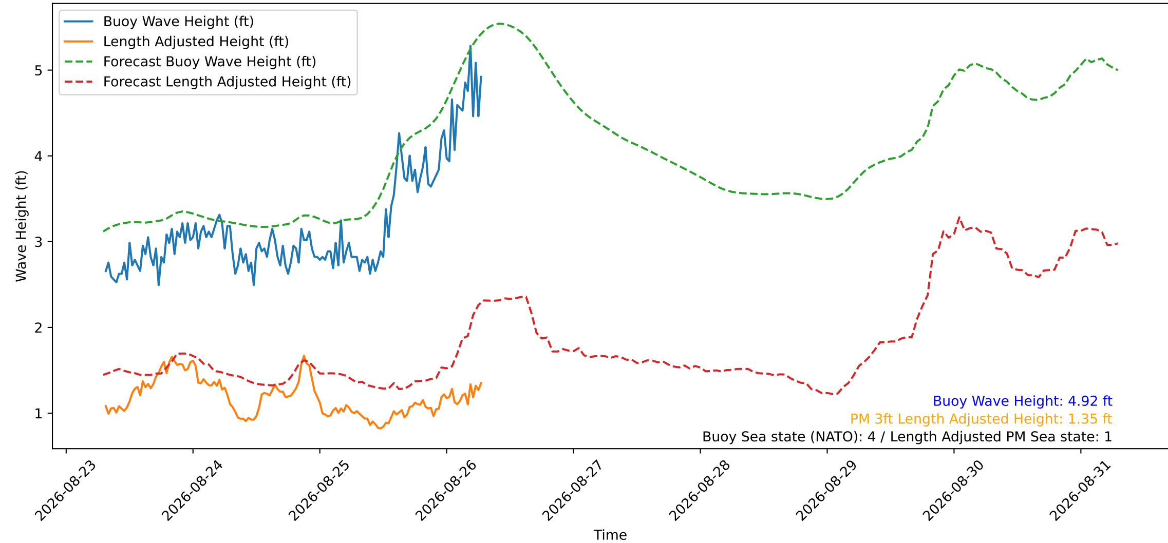
Wave Heights over Time for Green Beach at 2026-08-26 07:21:20
