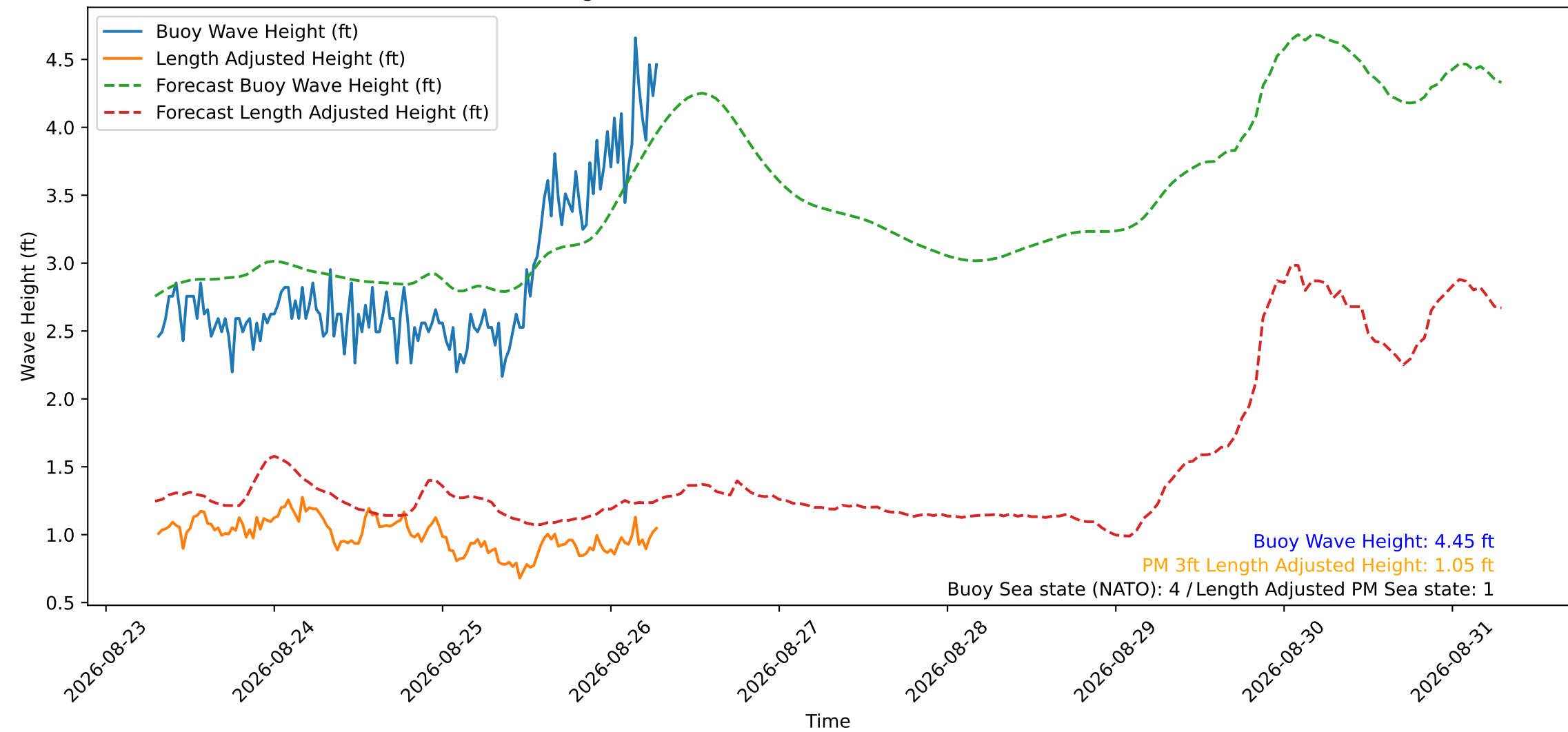
Wave Heights over Time for Red Beach at 2026-08-26 07:20:53
