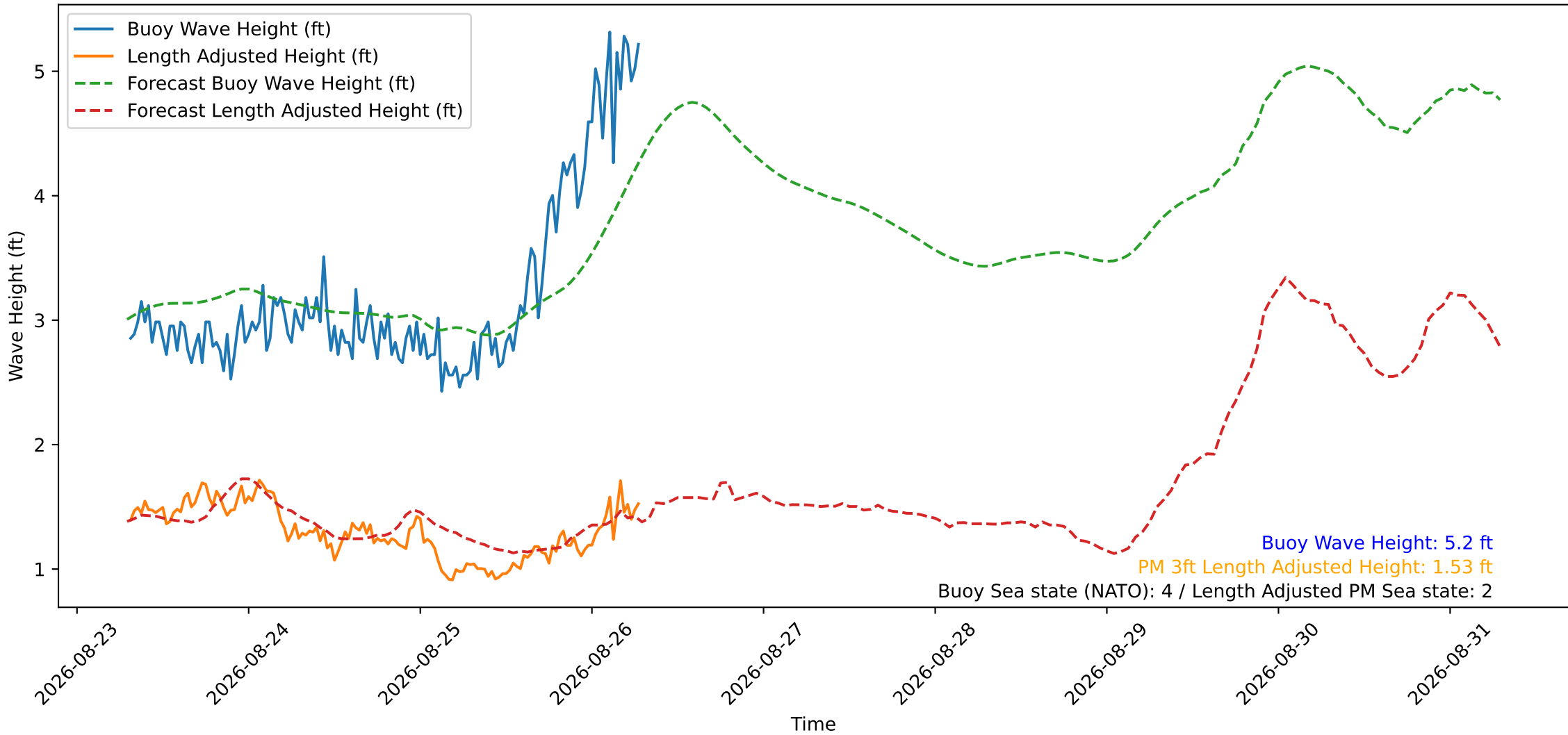
Wave Heights over Time for Oceanside Harbor at 2026-08-26 07:20:31
