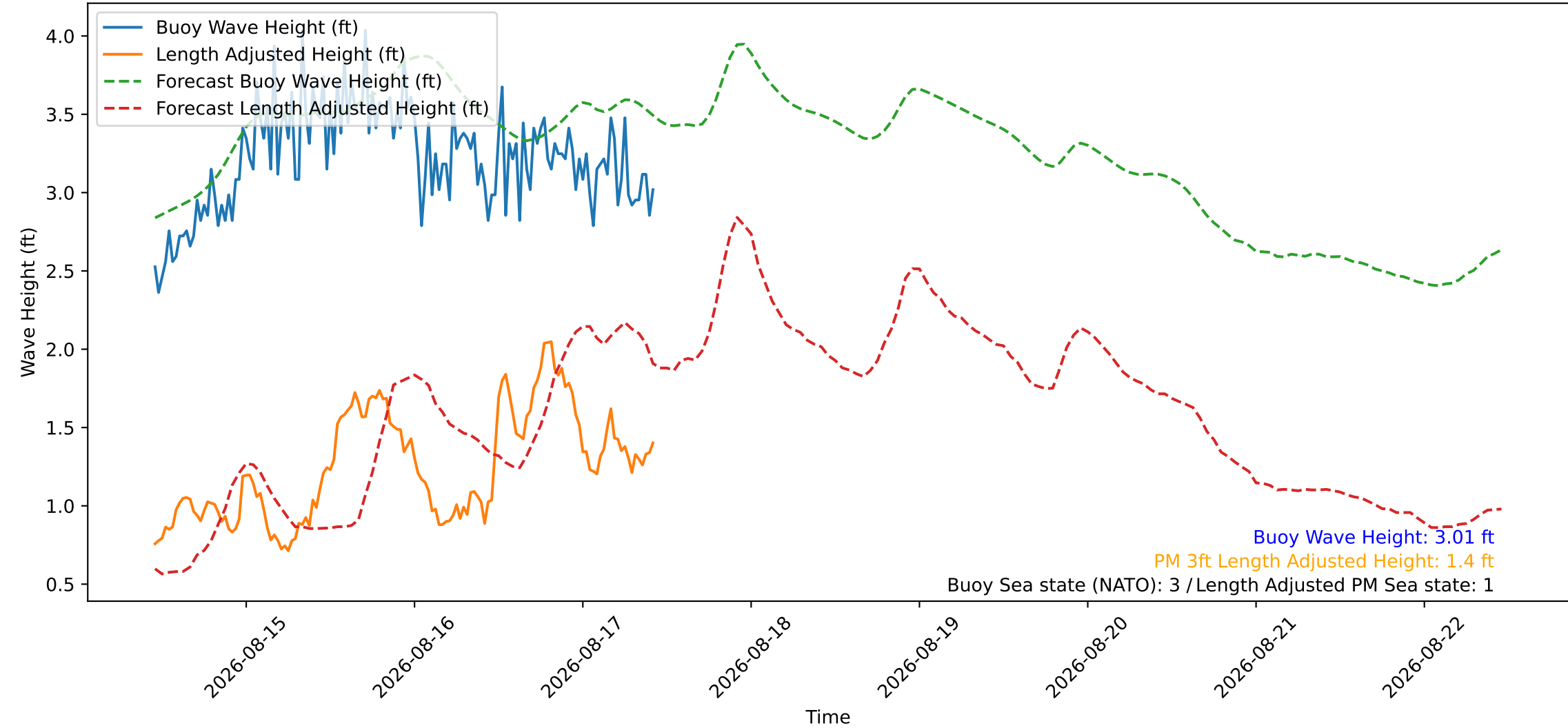
Wave Heights over Time for Red Beach at 2026-08-17 10:50:47
