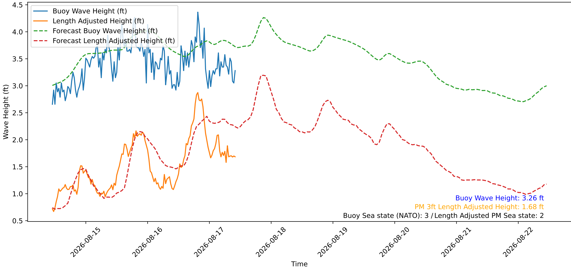
Wave Heights over Time for Green Beach at 2026-08-17 10:51:11
