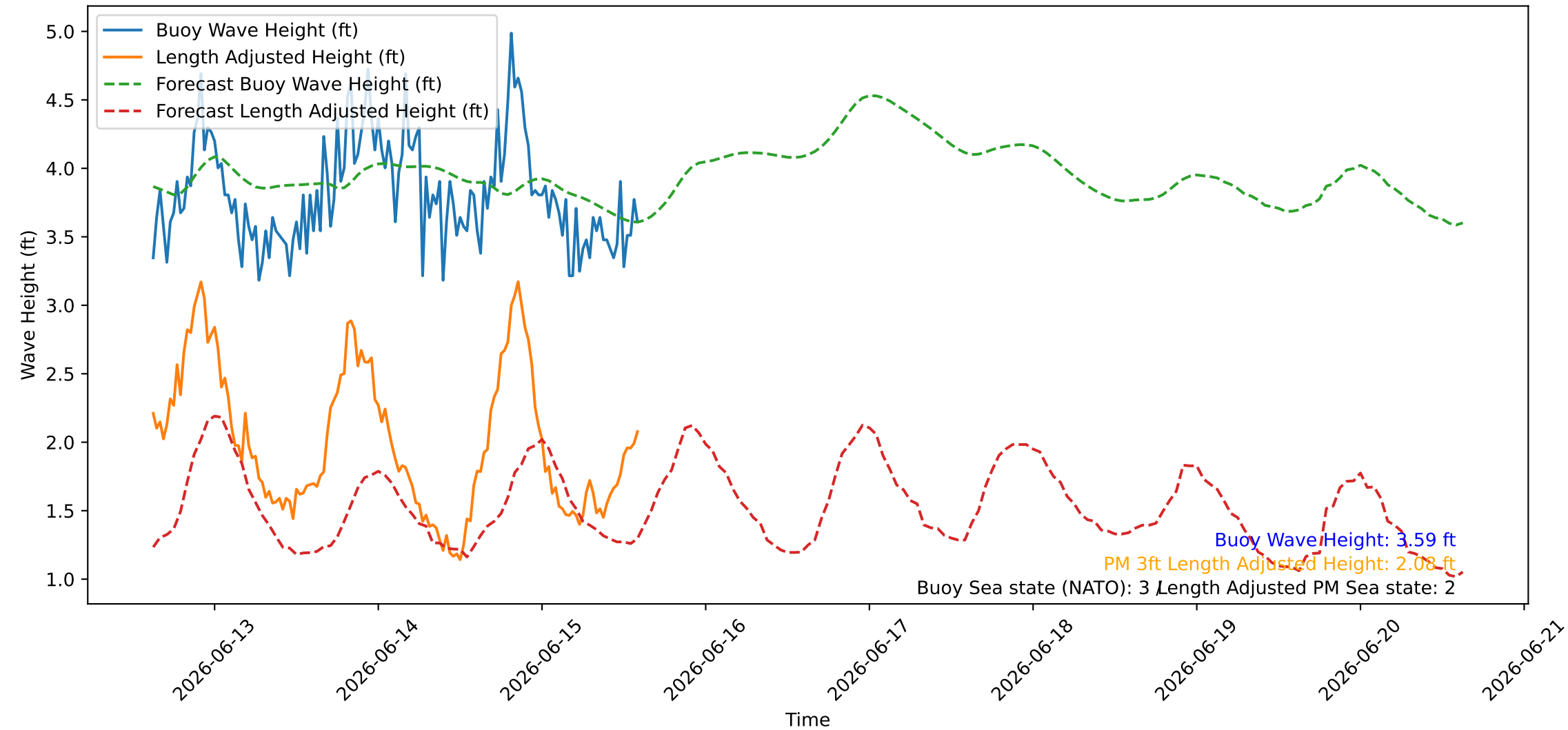
Wave Heights over Time for Oceanside Harbor at 2026-06-15 15:00:26
