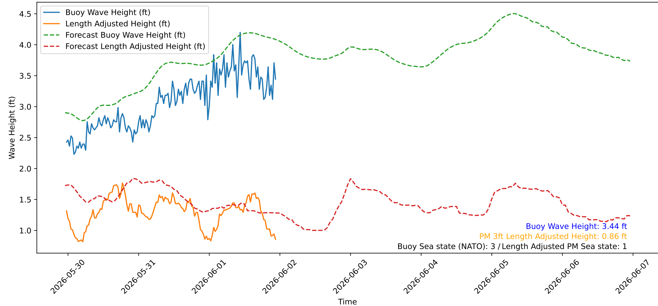
Wave Heights over Time for Red Beach at 2026-06-01 23:20:46
