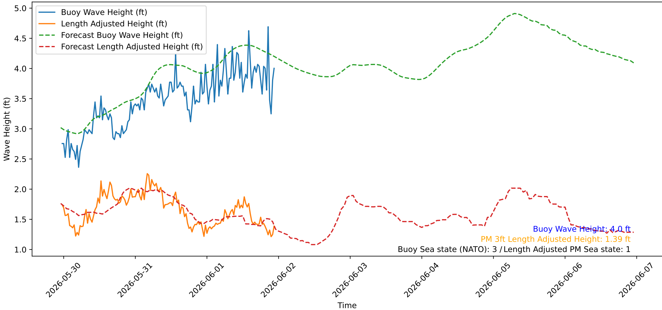
Wave Heights over Time for Oceanside Harbor at 2026-06-01 23:20:26
