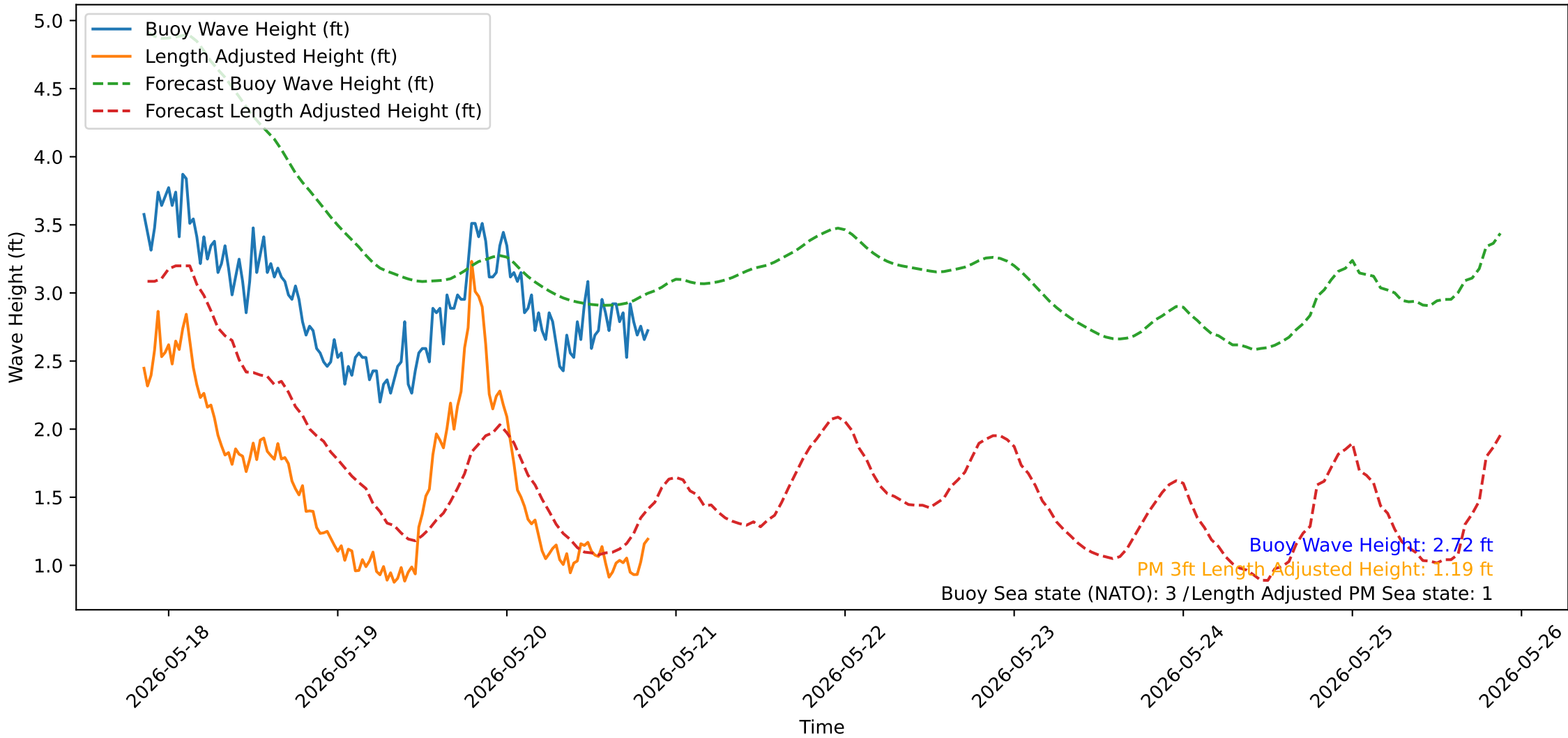
Wave Heights over Time for Oceanside Harbor at 2026-05-20 20:30:32
