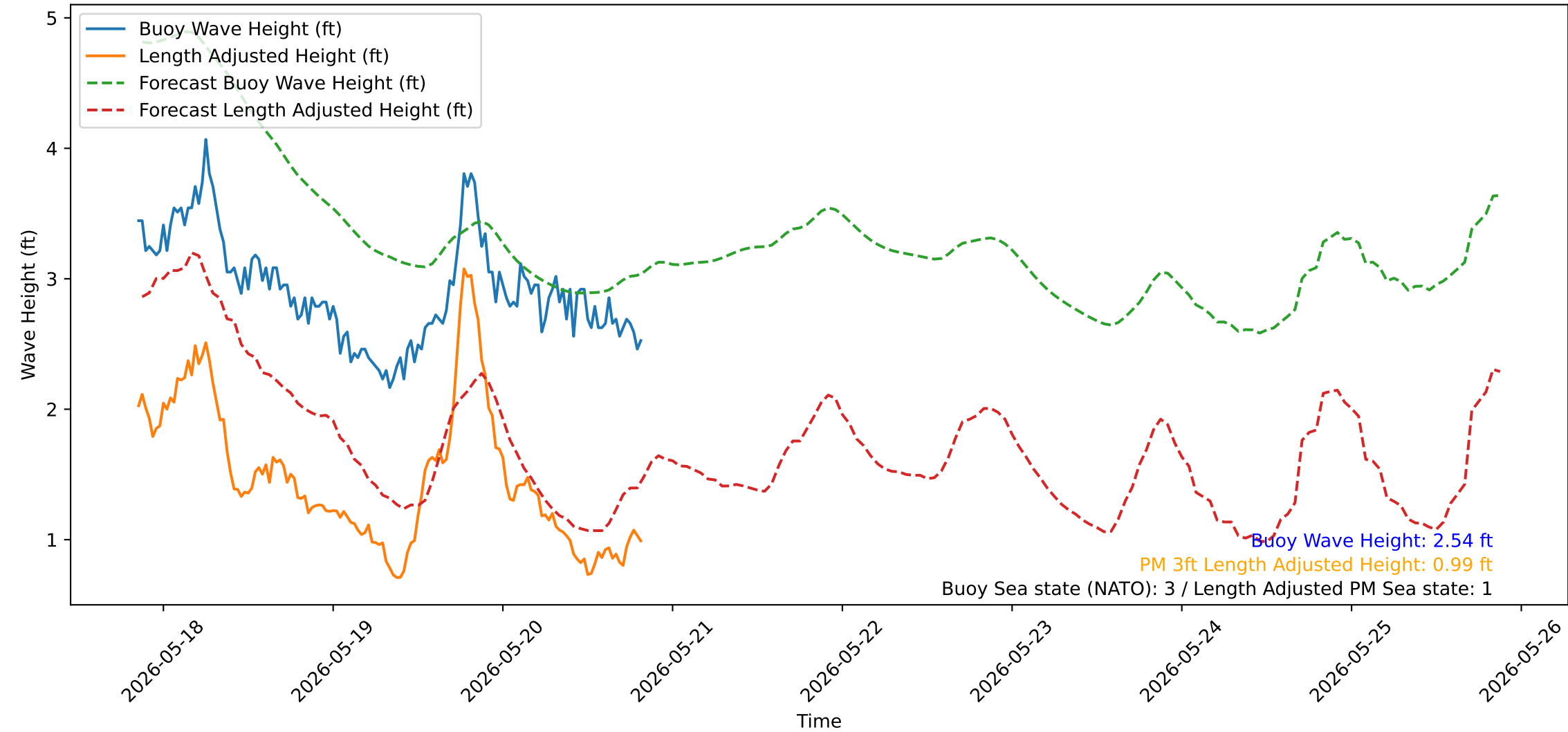
Wave Heights over Time for Green Beach at 2026-05-20 20:31:14
