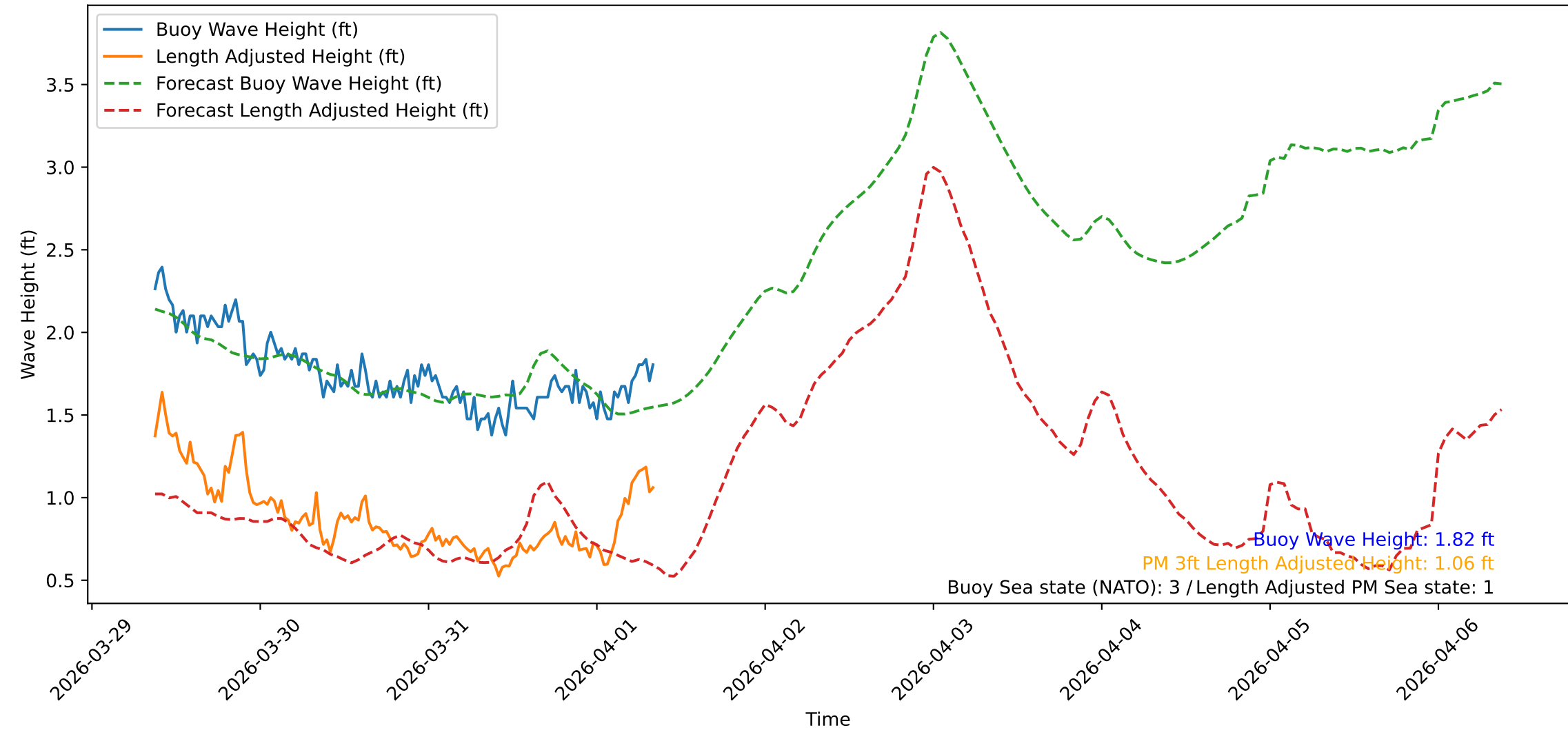
Wave Heights over Time for Red Beach at 2026-04-01 08:50:48
