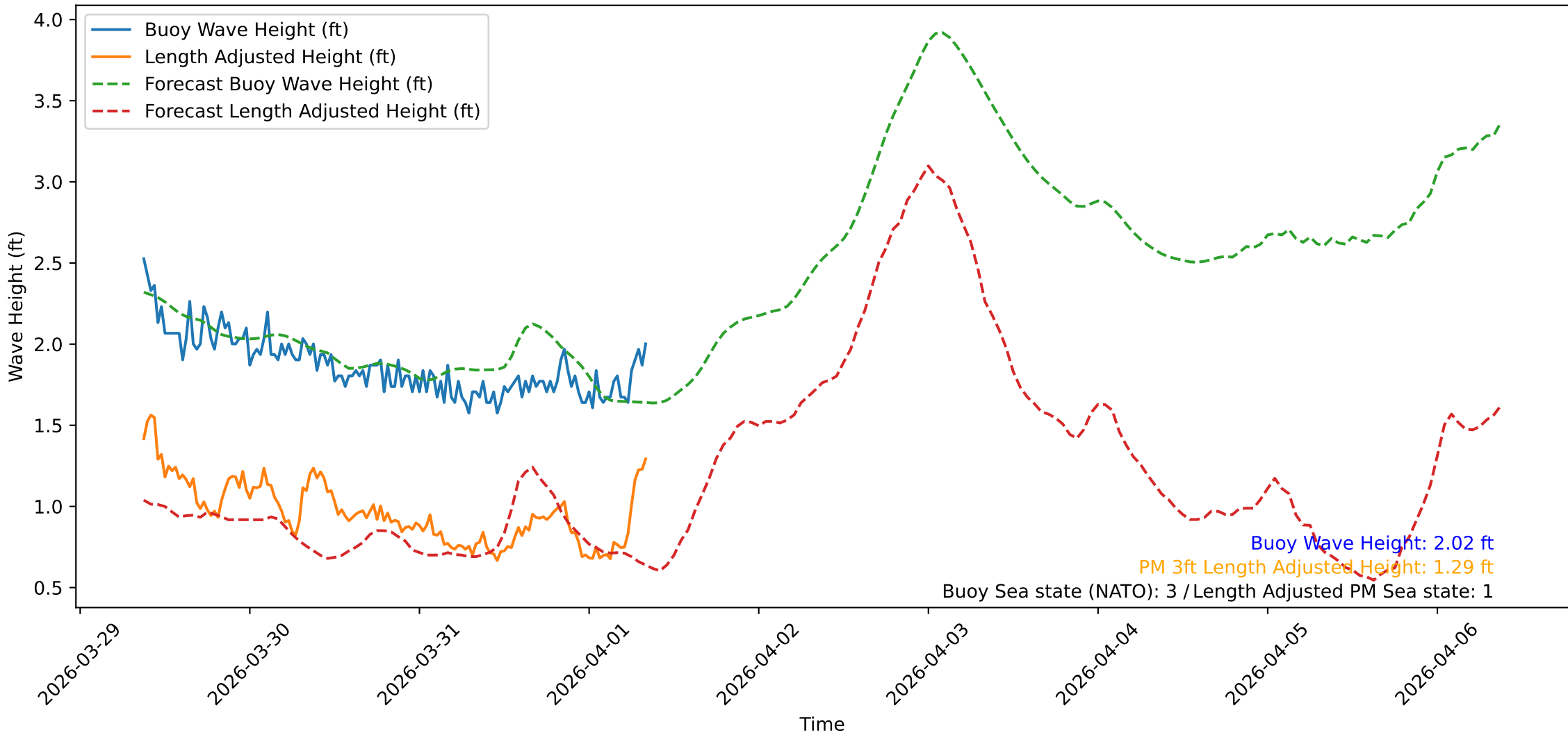
Wave Heights over Time for Oceanside Harbor at 2026-04-01 08:50:31
