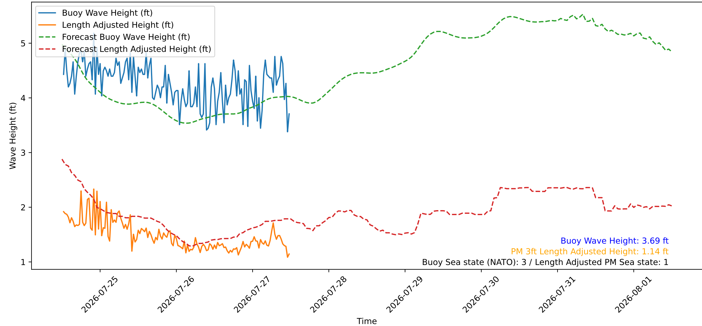
Wave Heights over Time for Green Beach at 2026-07-27 12:21:09
