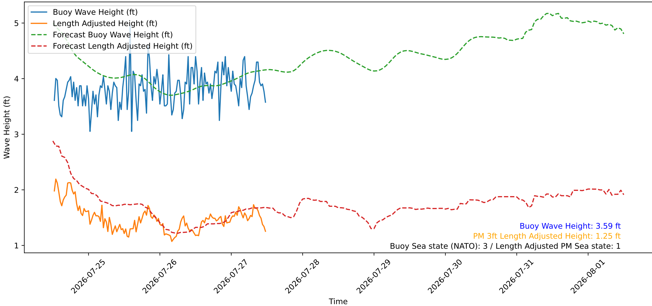
Wave Heights over Time for Oceanside Harbor at 2026-07-27 12:20:26
